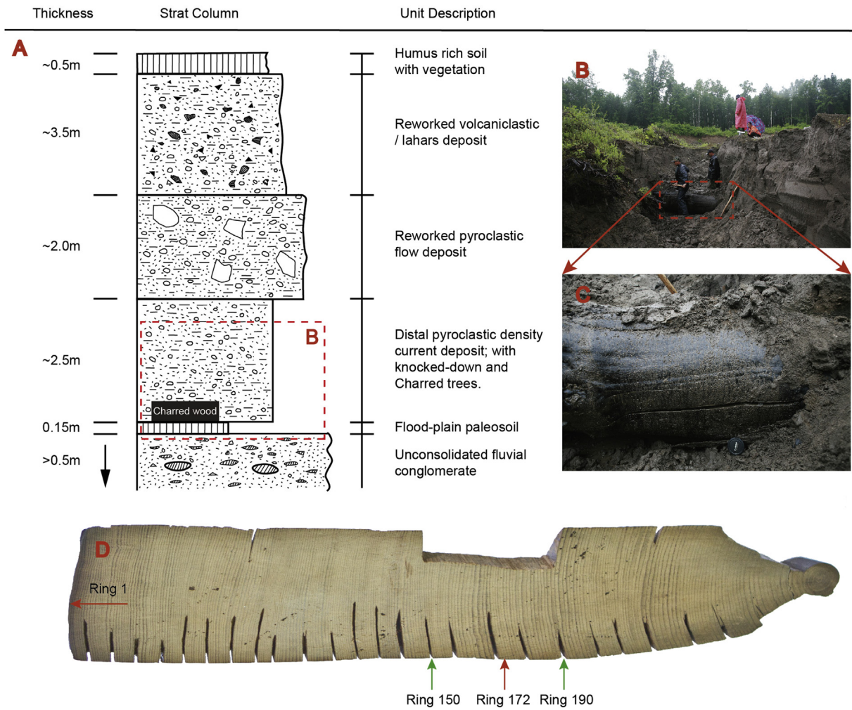
Fig. 3. Context for the sampled Larix stem. (A) Stratigraphic section showing location of tree. (B) The tree in situ at the sampling location; the deposits encasing it correspond to the part of the stratigraphy highlighted by the dashed box labelled 'B' in the schematic section to the left. (C) a close-up view of the tree. (D) Cross-section of sampled trunk (approximately 0.35 m radius) showing selected ring numbers.
