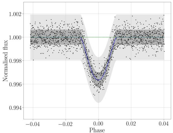
Figure 6. Transit light curve of the TOI-503, fitted with the GP model described in Section 3.1.3. The blue line represents the best fitting transit light curve, and the green line shows the model without the transit function. The dark and light gray regions represent the 1\sigma and 3\sigma prediction of the GP model.
