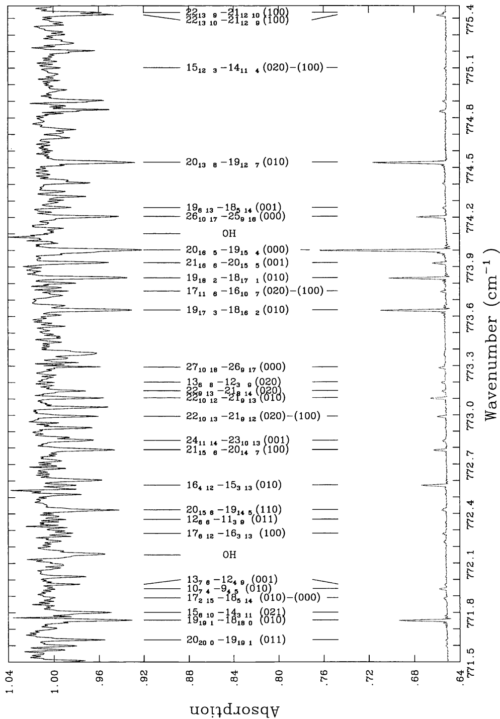
Figure 6.3: Top: part of the sunspot spectrum of Wallace et al (1995). The region covered is from 771.5 to 775.5 cm -1 . Quantum number assignments, given as J_{K_a K_c} (upper)- J'_{K'_a K'_c} (lower) for various vibrational states (labelled using standard notation (v_1 v_2 v_3) ), are marked. Bottom: the corresponding part of the laboratory spectrum (Polyansky et al , 1996b). For convenience, we have normalized the intensity.
