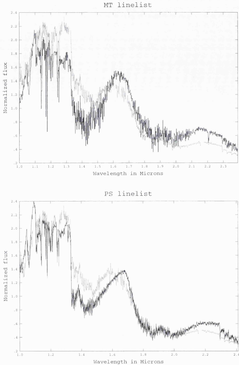
Figure 7.7: Comparisons of observed and synthetic spectra for the star TVLM. The models were computed at T_{eff} = 2500 K, [M/H] = 0.0 , \log g = 5.0 . Top: the model includes the MT linelist for the opacity of water. Bottom: the model includes the PS linelist. The dotted curve is the observed spectrum
