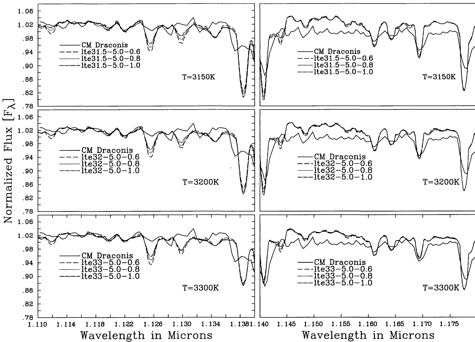
Figure 9.30: Left: Detailed comparison of the region 1.11-1.40 \mu\text{m} . Right: Detailed comparison of the region 1.40-1.80 \mu\text{m}
