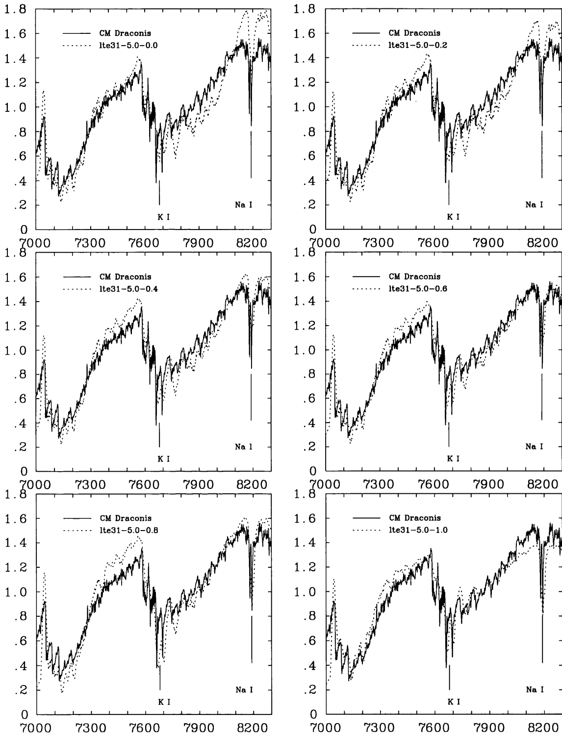
Figure 9.10: Comparison of observed spectrum with models at T_{\text{eff}}=3100 K in the region 7000–8300 Å
