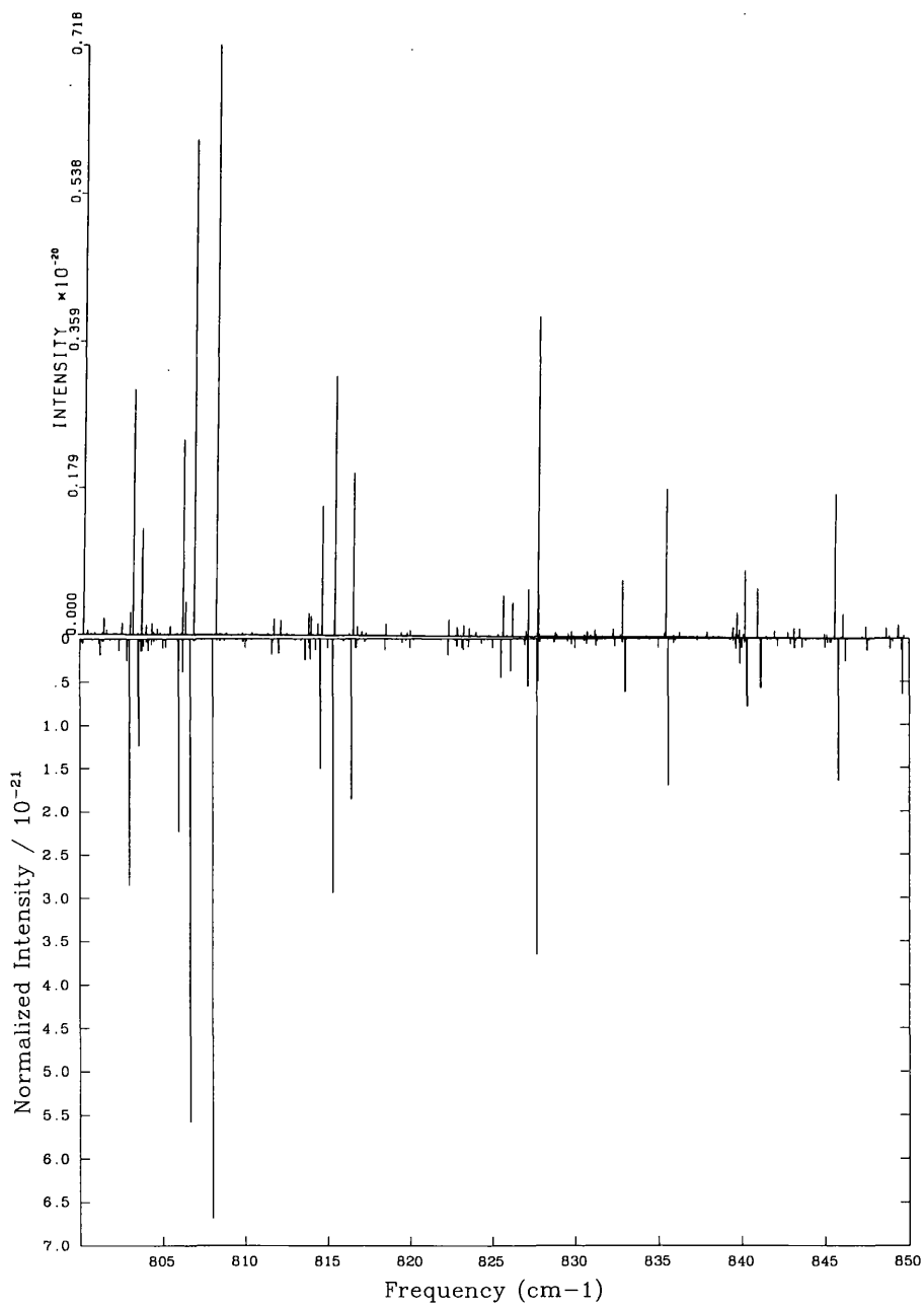
Figure 5.4: Top: HITEMP spectrum at 1000K. The graph has been kindly provided in hardcopy by Rothman (private communications 1996). Bottom: VTP1 spectrum at 1000K. The slight deposition is not due to difference in frequency but to graphical problems in scaling VTP1 to fit a scanned picture of the HITEMP spectrum.
