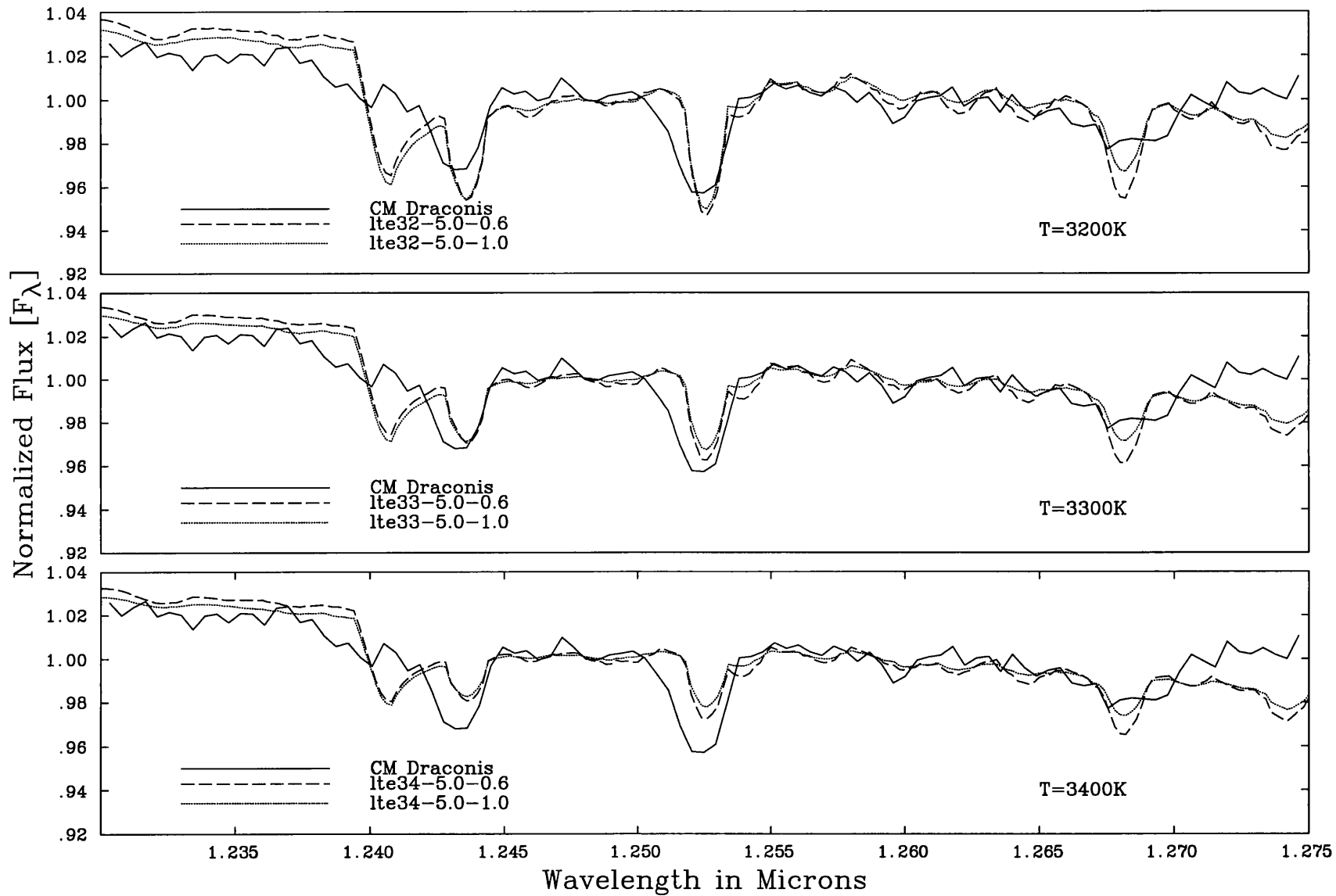
Figure 9.31: Detailed comparison of the region 1.230–1.275 \mu\text{m} .
