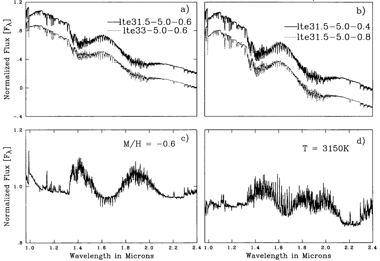
Figure 9.2: Sensitivity of the models to changes in T_{\text{eff}} and [M/H] . The different models are distinguished using the notation lteTT-G.G-Z.Z, where lte = local thermodynamic equilibrium assuming \zeta(\text{LTE}) = 2 \text{ km s}^{-1} , TT = T_{\text{eff}}/100 , G.G = \log g (surface gravity), Z.Z = [M/H] (metallicity), where [M] \equiv \log M_{\text{star}} - \log M_{\odot} for any abundance quantity M . Top left: comparison of the T_{\text{eff}}=3150 \text{ K} model with the T_{\text{eff}}=3300 \text{ K} one at a fixed metallicity, [M/H]= -0.6 . The y axis of the 3300 K model has been shifted by 0.2 for clarity. Bottom left: the 3150 K model divided by the 3300 K one. Top and bottom right: same as left but comparing [M/H]= -0.4 with [M/H]= -0.8 for a fixed T_{\text{eff}}=3150\text{K} .
