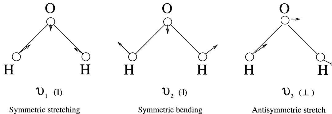
Figure 3.1: The three fundamental vibrational modes of water.
