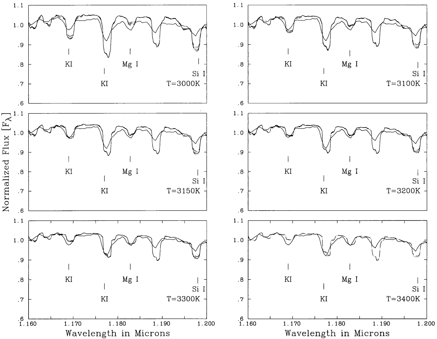
Figure 9.28: Comparisons of the region 1.16–1.2 \mu\text{m} . Again continuous line is CM Dra; dashed, dotted, dot-dotted and double dot-dotted lines are the models at respectively
