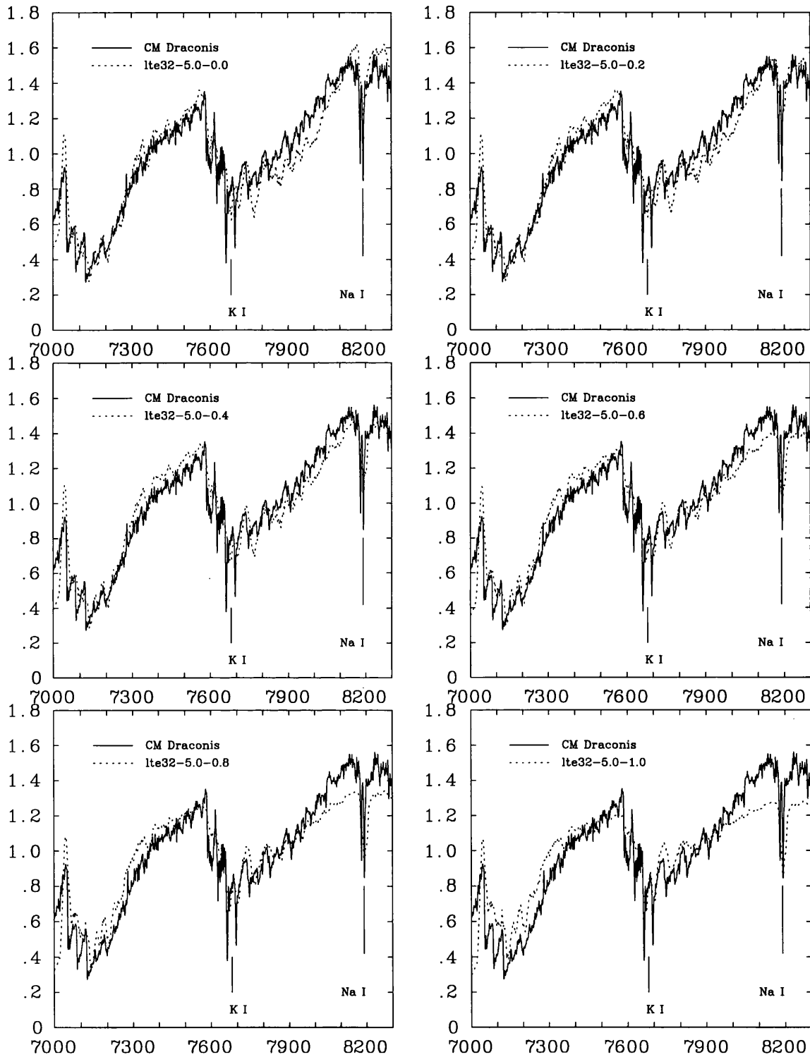
Figure 9.12: Comparison of observed spectrum with models at T_{\text{eff}}=3200 K in the region 7000–8300 Å
