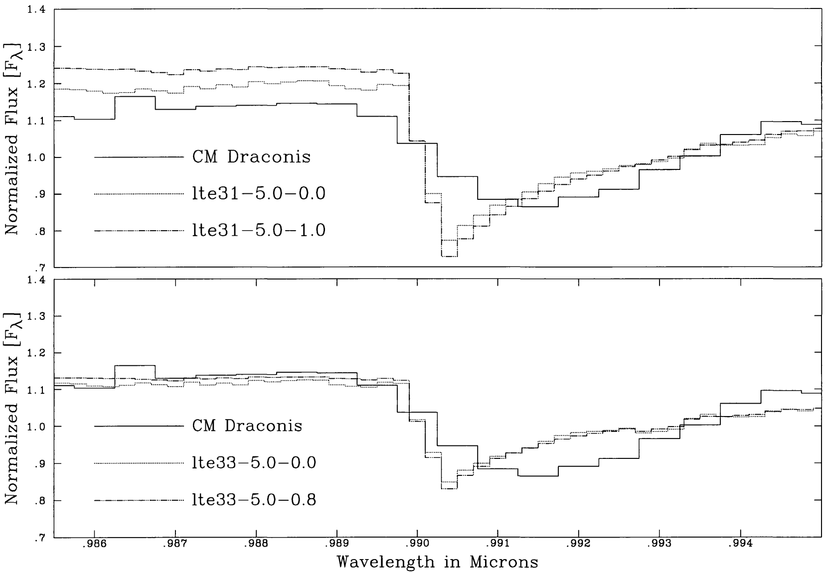
Figure 9.19: Fit to the FeH band centered at \sim 0.992 \mu\text{m} for the T_{\text{eff}}=3100\text{K} , [M/H]=0.0 , -1.0 models (top plot) and for the T_{\text{eff}}=3300\text{K} , [M/H]=0.0 , -0.8 models (bottom plot).
