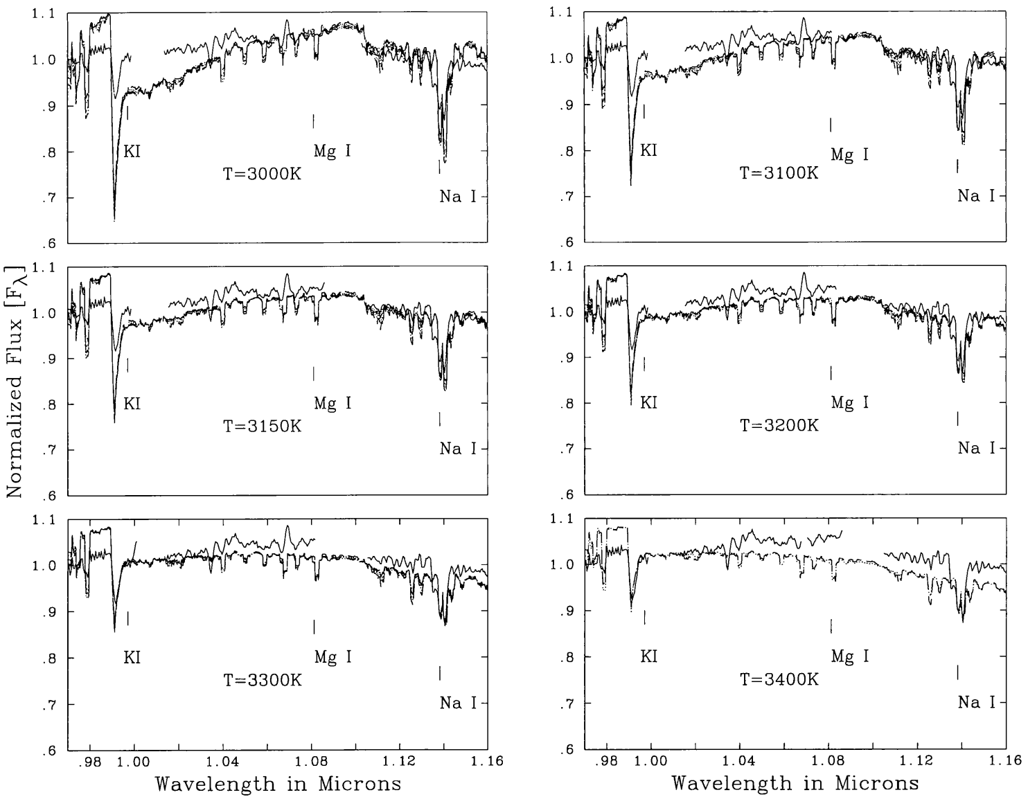
Figure 9.27: Comparisons of the region 0.95–1.16 \mu\text{m} . Continuous line is CM Dra; dashed, dotted, dot-dotted and double dot-dotted lines are the models at respectively [M/H] = -0.4, -0.6, -0.8, -1.0 .
