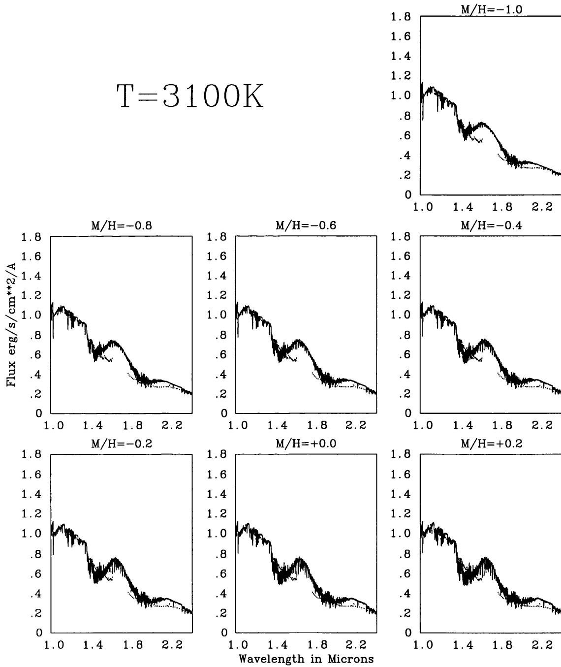
Figure 9.21: Infrared SED comparison at T_{\text{eff}}=3100\text{K}
