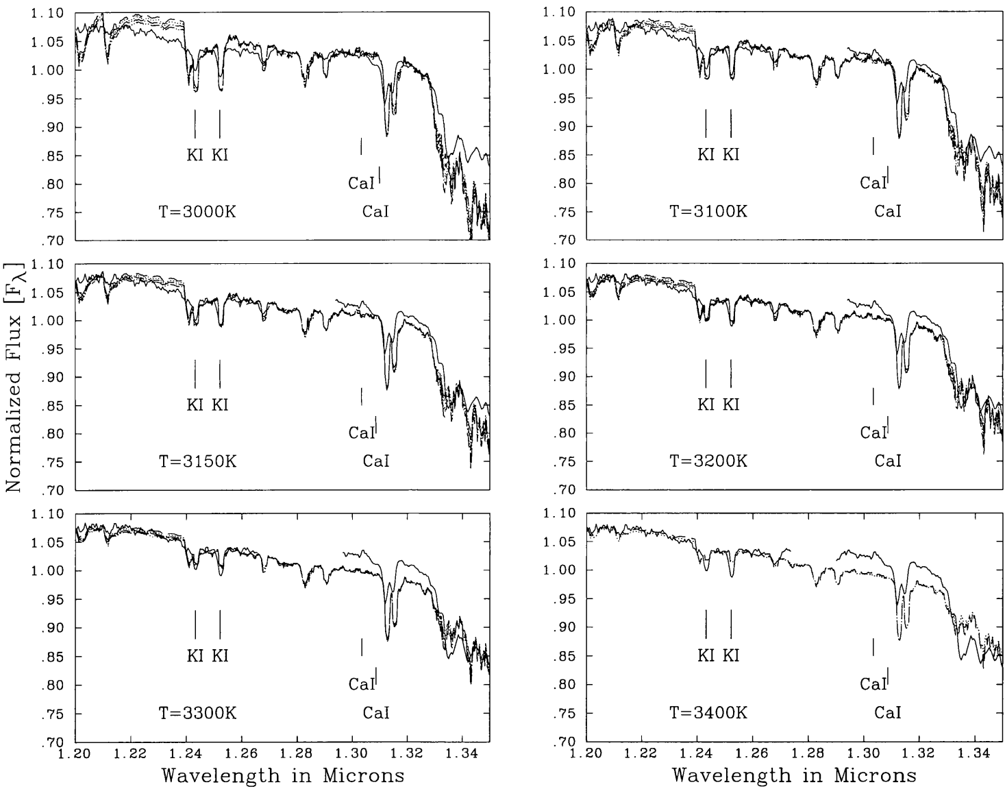
Figure 9.29: Comparisons of the region 1.2–1.34 \mu\text{m} . Continuous line is CM Dra; dashed, dotted, dot-dotted and double dot-dotted lines are the models at respectively [M/H] = -0.4, -0.6, -0.8, -1.0 .
