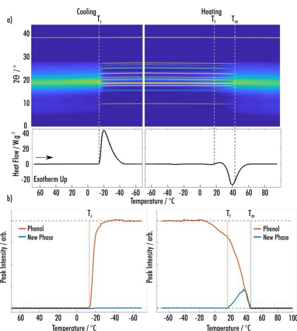
Figure 2 a) (Top) Surface plot of pXRD patterns of an 8:1 phenol:MAP VODES as a function of temperature. (Bottom) DSC trace for the temperature cycle shown in the pXRD surface plot. b) Integrated peak intensities of phenol and the new phase of phenol:MAP as a function of temperature during the cycle shown in a).
