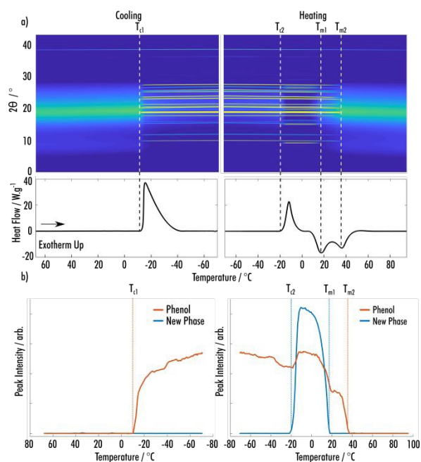
Figure 3 a) (Top) Surface plot of pXRD patterns of an 8:1 phenol:2EB VODES as a function of temperature. (Bottom) DSC trace for the temperature cycle shown in the pXRD surface plot. b) Integrated peak intensities of phenol and the new phase of phenol:2EB as a function of temperature during the cycle shown in a).
