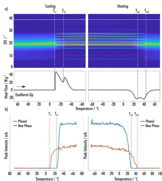
Figure 5 a) (Top) Surface plot of pXRD patterns of a 9:1 phenol:BZM VODES as a function of temperature. (Bottom) DSC trace for the temperature cycle shown in the pXRD surface plot. b) Integrated peak intensities of phenol and the new phase of phenol:BZM as a function of temperature during the cycle shown in a).
