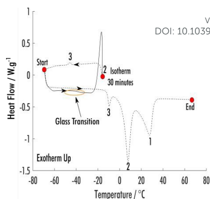
Figure 4 DSC of an 8:1 phenol:2EB VODES. At the point "start" the sample has been cooled to -70\text{ }^{\circ}\text{C} from 70\text{ }^{\circ}\text{C} . The thermogram follows the solid line and then dashed lines. The numbers highlight the crystallisation and melts of the different phases. 3 is the phase formed on cooling the sample after it had been held at T_{c2} . 2 is the new phase that formed during synchrotron-DSC analysis. 1 is the ambient crystal structure of phenol, which had already crystallised during the initial cool from 70\text{ }^{\circ}\text{C} .
