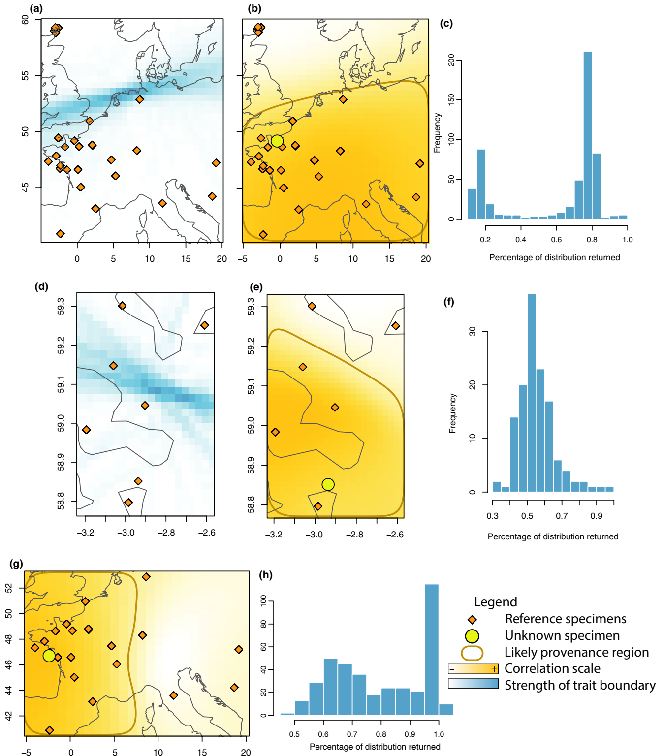
FIGURE 3 Microtus arvalis results at three different geographic scales: (a–c) Combined European and Orkney archipelago range; (d–f) Orkney archipelago; (g–h) Mainland Europe. The results of the boundary finder method are presented in (a) and (d). Example identification outputs are presented in (b), (e) and (g). Histogram showing the percentage of the species range returned by the provenancing method at a 95% confidence level in (c), (f) and (h)
