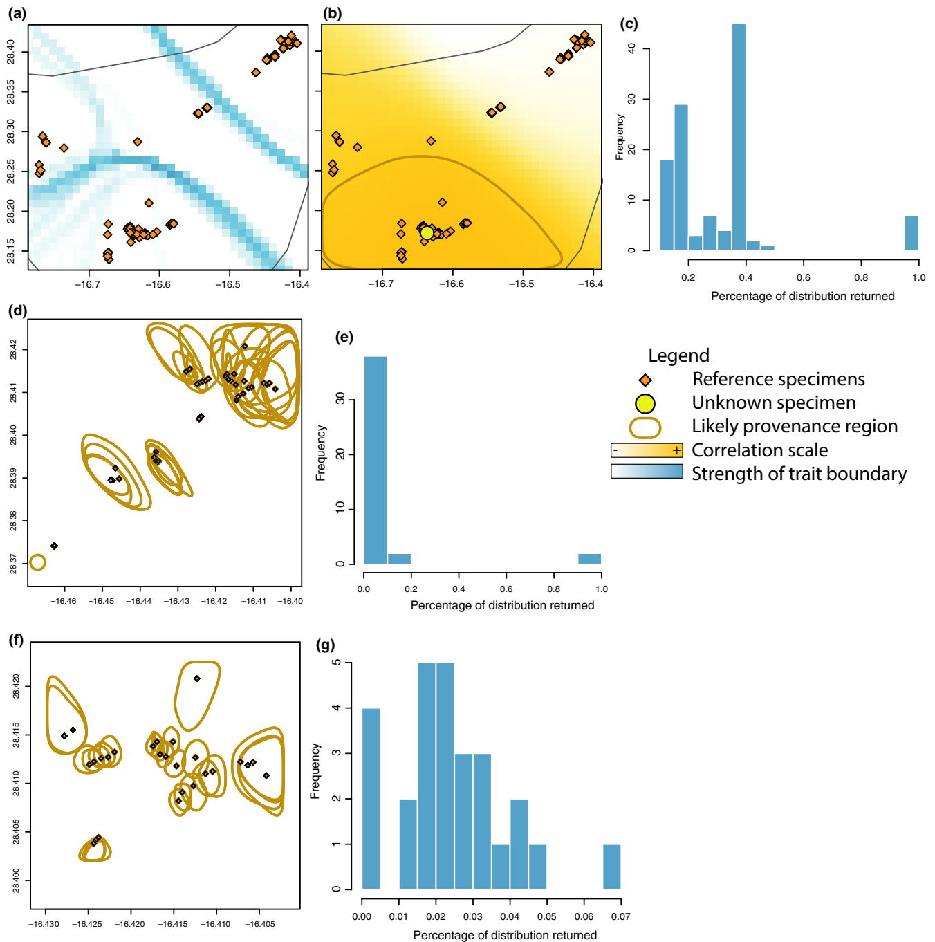
FIGURE 4 Fringilla teydea provenancing and boundary finding at different geographic scales. (a–c) The results from island-wide analyses on the raw dissimilarity data; (d–e) The results from the Northern sub-region; (f–g) The results from most densely sampled NE area. At the highest resolution (f–g) the results of all the individual cross-validation identifications are superimposed as polygons around the specimen's true location (note that almost all points fall within a spatial provenancing polygon). The proportion of reference distribution identified is calculated at each resolution level separately and as a result the analyses run on subsets of the data are not the proportion of the total species range
