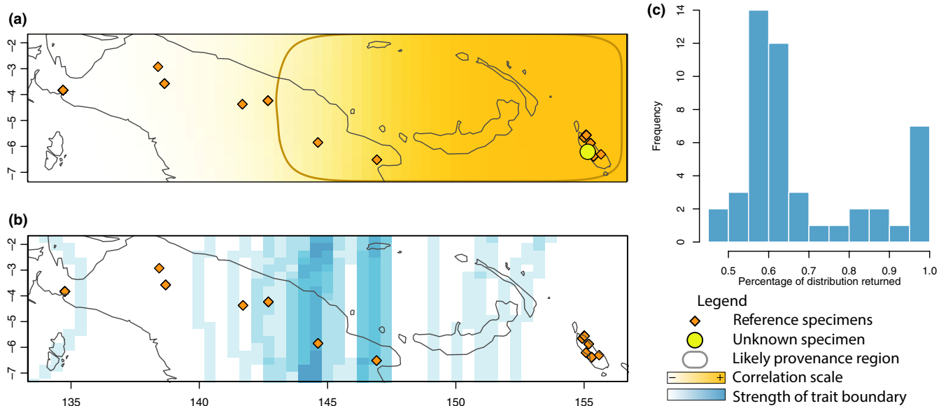
FIGURE 2 Spatial identification by distance of Rattus praetor . (a) Example output of result—the polygon encompasses the region of correlation values at the 95% r threshold. (b) Boundary finder output demonstrating identification gradient and boundaries around the 145th meridian. (c) Histogram showing the percentage of the species range returned by the provenancing method at a 95% confidence level
