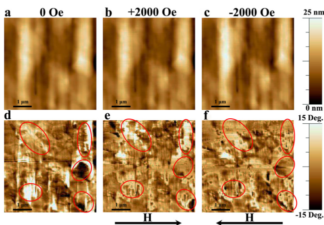
FIG. 5. Ferroelectric domain switching in BLFCT under the applied magnetic field ( H is parallel to the surface of the sample). (a) Topography and (d) vertical PFM phase at 0 Oe; (b) topography and (e) vertical PFM phase at +2000 Oe; and (c) topography and (f) vertical PFM phase at −2000 Oe.
