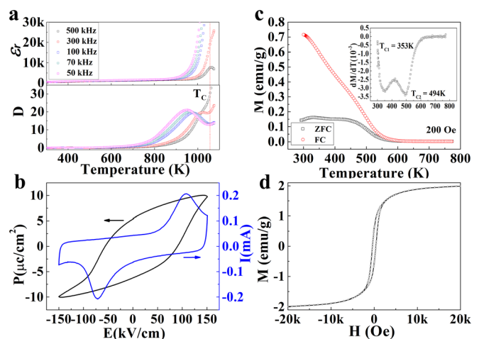
FIG. 2. (a) The temperature dependence of the relative dielectric permittivity (above) and loss tangent (down) of BLFCT ceramics measured perpendicular [ \perp ] to the SPS pressure direction. (b) The P - E and I - E hysteresis loops of the textured BLFCT ceramics measured perpendicular to the SPS pressure direction. The curves demonstrate the domain switching characteristic of a ferroelectric. (c) The temperature dependence of the magnetization for BLFCT ceramics [ \perp ] in the ZFC/FC modes measured in H = 200 Oe. The inset shows the first derivative of magnetization dM/dT as a function of temperature. (d) The field dependence of magnetization at 300 K for the BLFCT sample.
