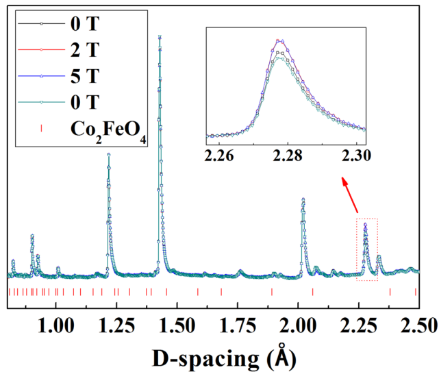
FIG. 4. The room-temperature neutron diffraction pattern obtained for the BLFCT ceramic at different magnetic fields (from 0, 2, and 5 T and then back to 0 T).
