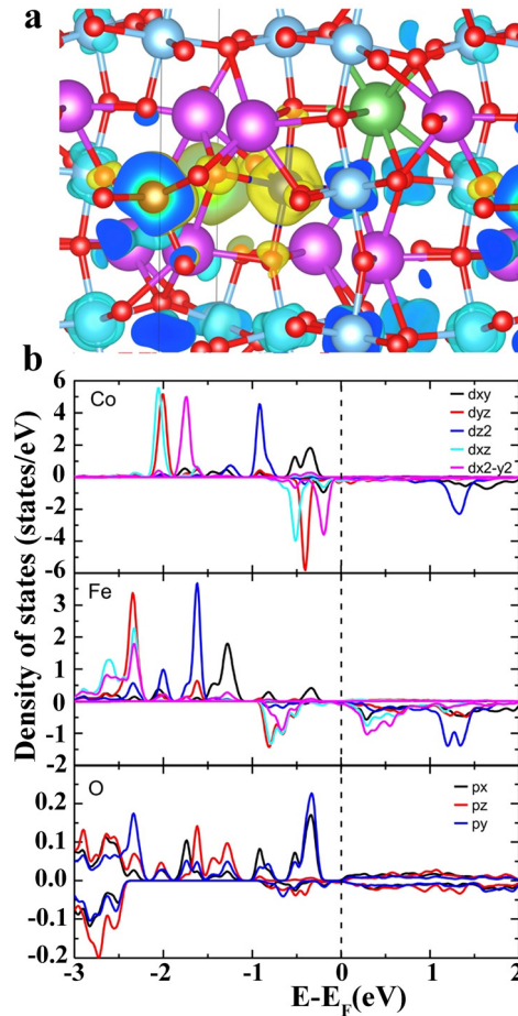
FIG. 3. (a) Spin density of the system (isosurface level = 0.005): O (red), Bi (pink), La (green), Ti (light blue), Co (dark blue), and Fe (yellow) atoms. (b) A detailed inspection of the density of state in \text{Fe}^{3+}\text{-O-Co}^{3+} .
