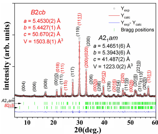
FIG. 1. X-ray diffraction pattern of the BLFCT powder.
