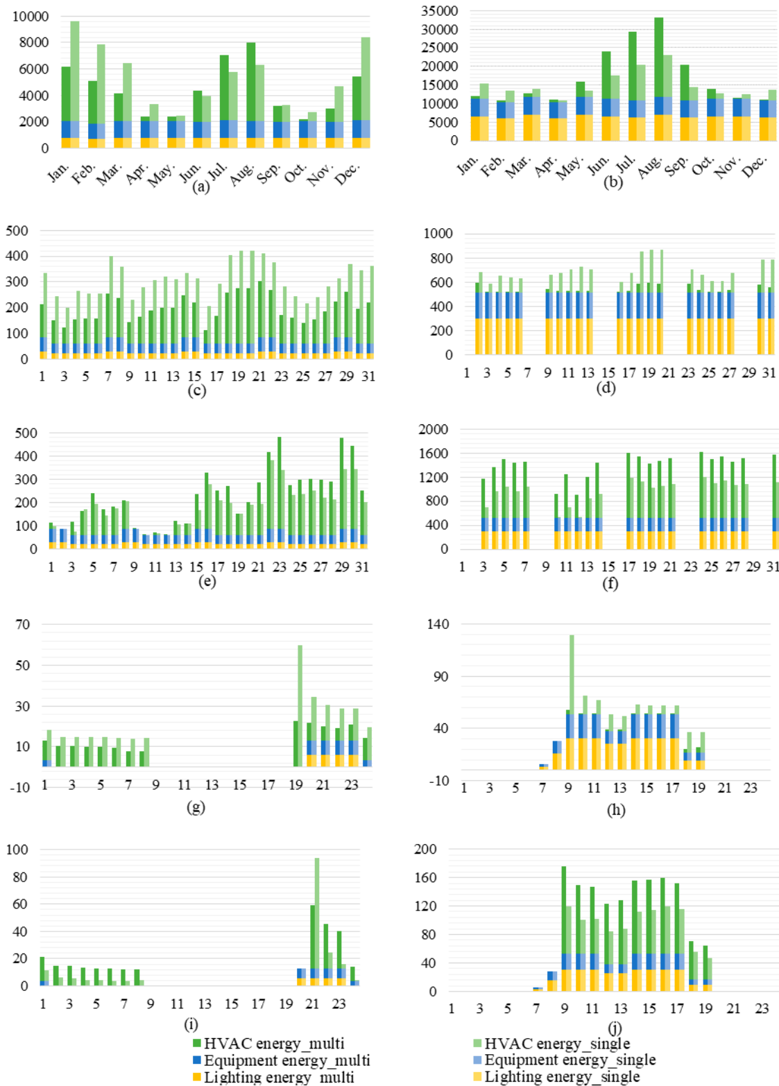
Figure 10. Energy consumption of residential and public buildings (MWh/m 2 -a): (a) monthly energy consumption of residential buildings; (b) monthly energy consumption of public buildings; (c) daily energy consumption of residential buildings in January; (d) daily energy consumption of public buildings in January; (e) daily energy consumption of residential buildings in July; (f) daily energy consumption of public buildings in July; (g) hourly energy consumption of residential buildings on 12 January; (h) hourly energy consumption of public buildings on 12 January; (i) hourly energy consumption of residential buildings on 21 July; (j) hourly energy consumption of public buildings on 21 July.
