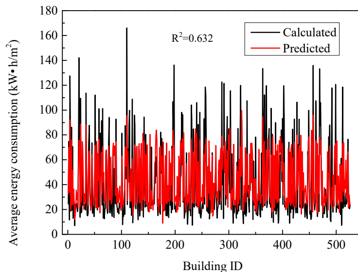
Figure 8. Comparisons of the multi-zone method and single-zone method.
