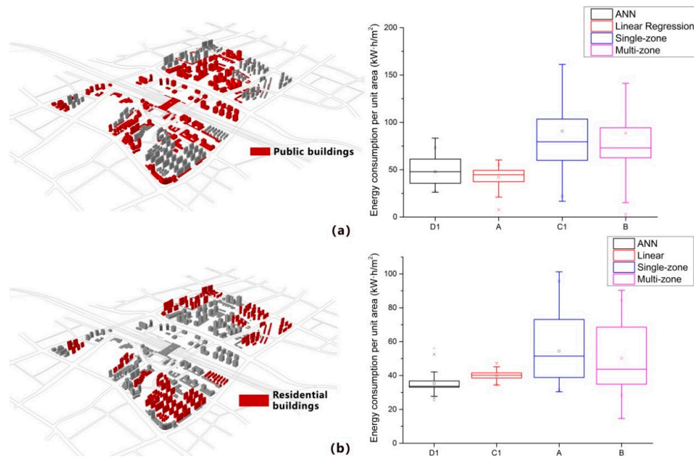
Figure 9. Comparison of energy consumption per unit area of four calculation methods: (a) dispersion of energy consumption intensity of public buildings; (b) dispersion of energy consumption intensity of residential buildings.
