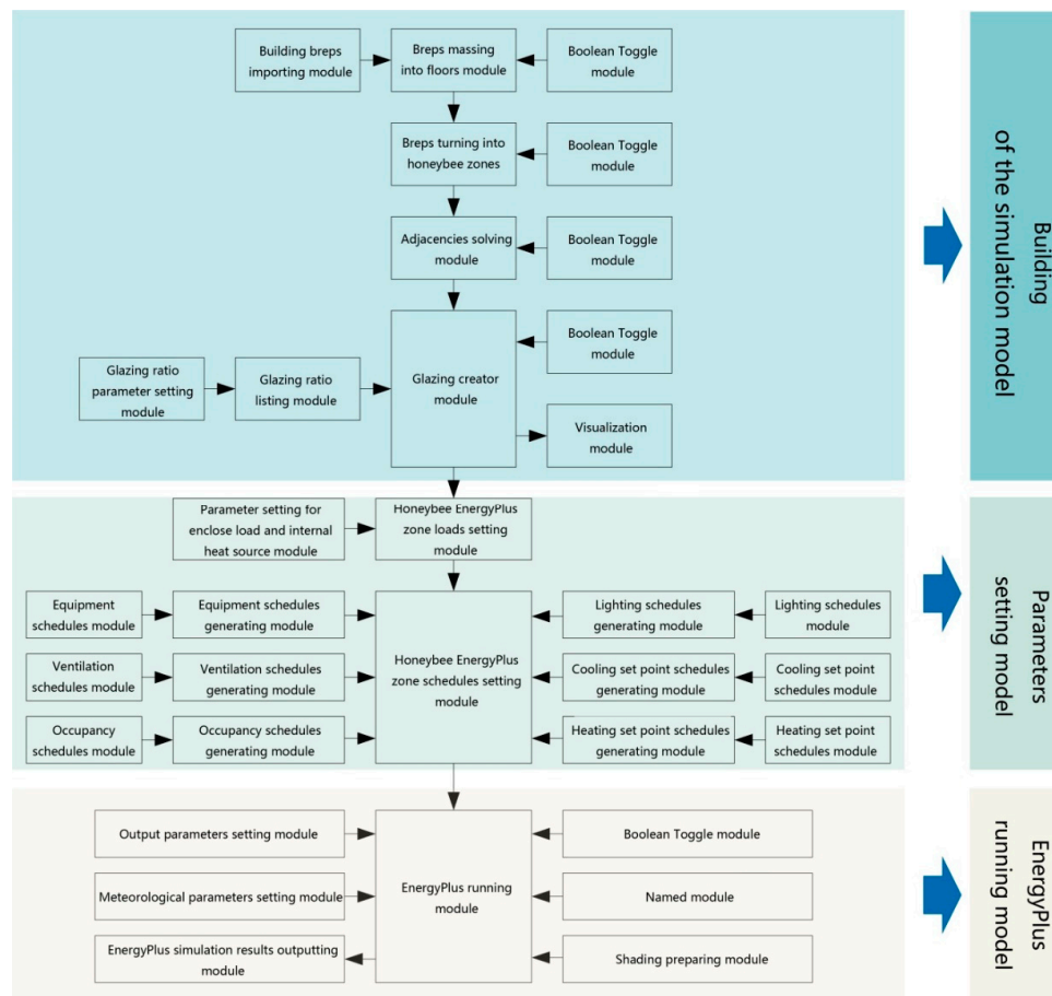
Figure 6. Components of the urban building energy simulation.
