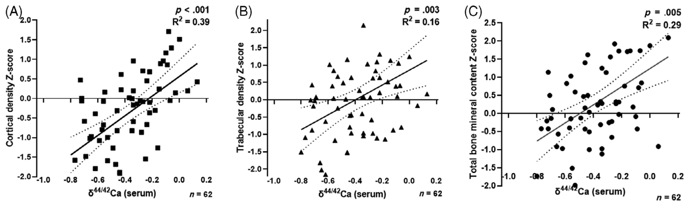
Fig 4. Correlation of \delta^{44/42}\text{Ca}_{\text{serum}} (‰) with bone density markers on peripheral quantitative computed tomography scan of the tibia in 62 participants (42 children older than 5 years and 20 adults). Tibial cortical density Z-score (A), trabecular density Z-score (B), and total bone mineral content Z-score (C) showed significant correlations with \delta^{44/42}\text{Ca}_{\text{serum}} , confirming an increase in bone mineral density as bone Ca content increases.
