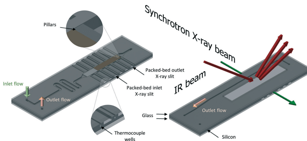
Fig. 2 Schematic representation of the back and front side of the microreactor for operando XAS/MS and DRIFTS/MS studies. A packed-bed catalyst (brown) and glass beads (light grey) upstream of the catalyst bed are depicted on the back side image. Insets show detailed view of the pillars used for retaining the catalyst particles and the thermocouple wells.
