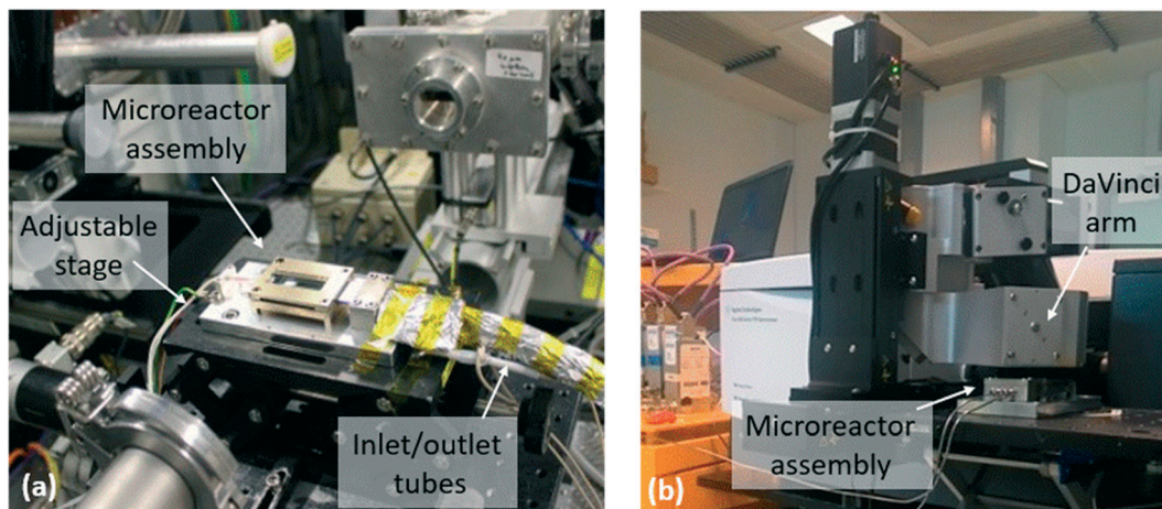
Fig. 3 Microreactor assembly (a) at the beamline B18 at the Diamond Light Source for the operando XAS/MS study and (b) at the Research Complex at Harwell for the operando DRIFTS/MS study.
