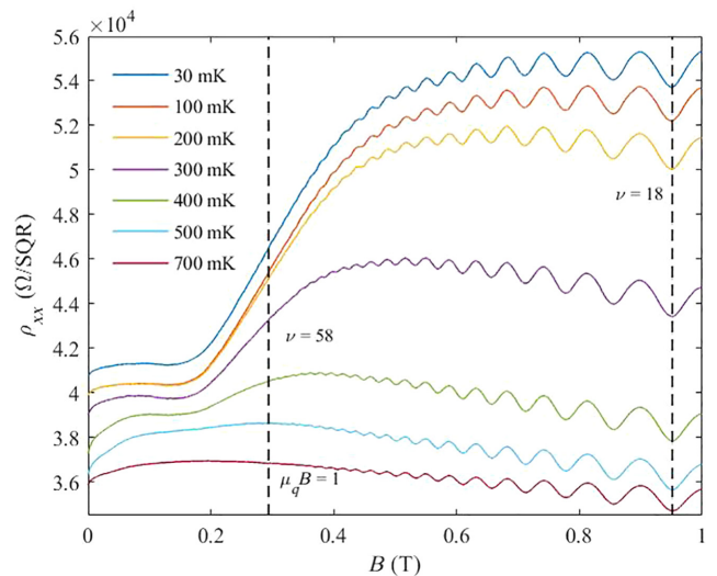
FIG. 6. \rho_{xx} up to 1 T from 30 to 700 mK. The oscillatory structure in \rho_{xx} can be seen down to \nu = 58 where the condition \mu_q B = 1 is then satisfied. The data for each temperature is plotted on the same scale, however the data for temperatures between 100 and 700 mK is shifted vertically by an arbitrary resistivity.
