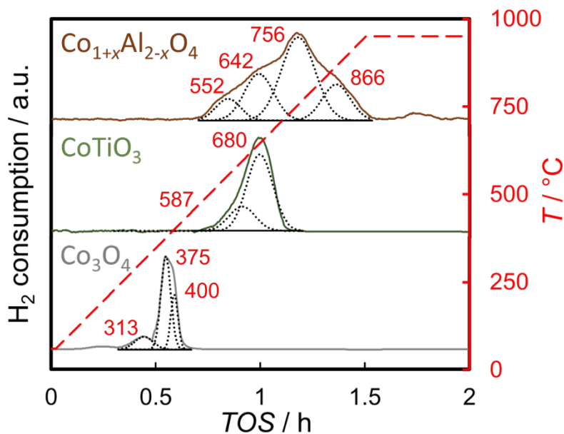
Figure 3 Temperature programmed reduction profiles with deconvoluted peaks of \text{Co}_{1+x}\text{Al}_{2-x}\text{O}_4 and \text{CoTiO}_3 nanoparticles synthesised via the benzyl alcohol route after calcination at 600 °C for 12 h, as well as of nano-sized \text{Co}_3\text{O}_4 for comparison.
