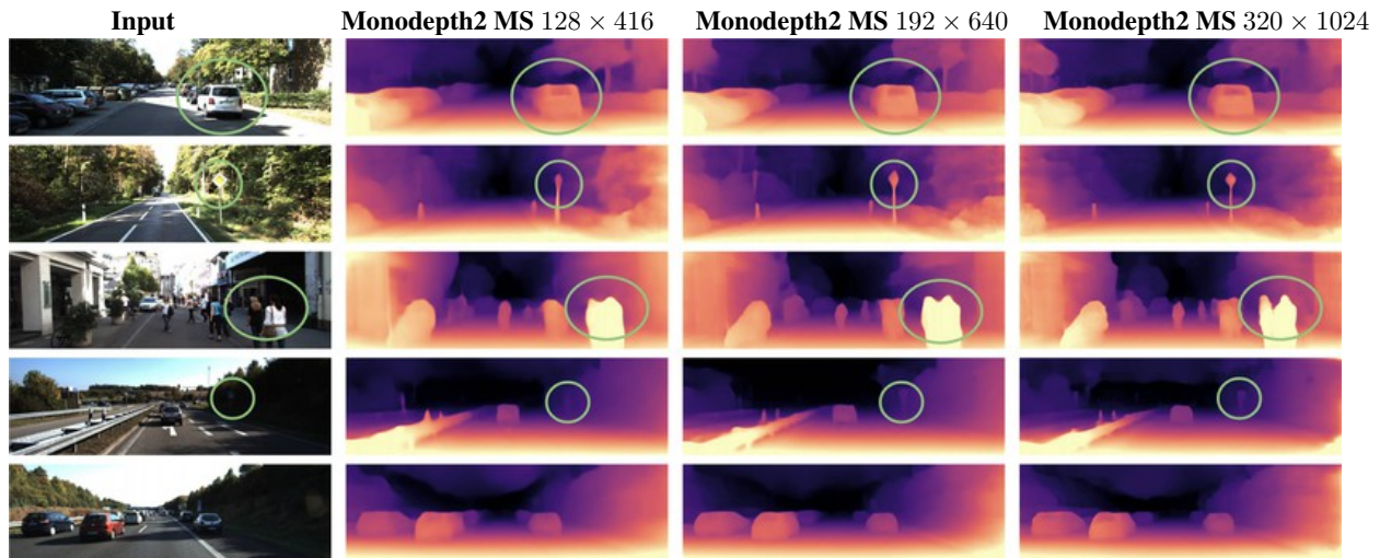
Figure 11. Effect of varying resolutions on the KITTI Eigen split. All predicted disparity maps have been resized to the same size for visualization. Our lowest resolution model (128 × 416) captures the broad shape of the scene successfully, but struggles with thin objects and sometimes fails to accurately capture the shape of depth discontinuities around object boundaries.
