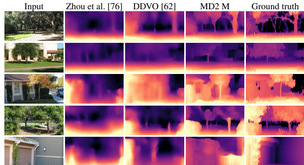
Figure 10. Additional Make3D results. Our model (MD2 M) trained on KITTI results in plausible depths, predicting more detail than existing monocular methods. The last row is an interesting failure for all methods as it contains an image that is very different than those from the KITTI training set.
