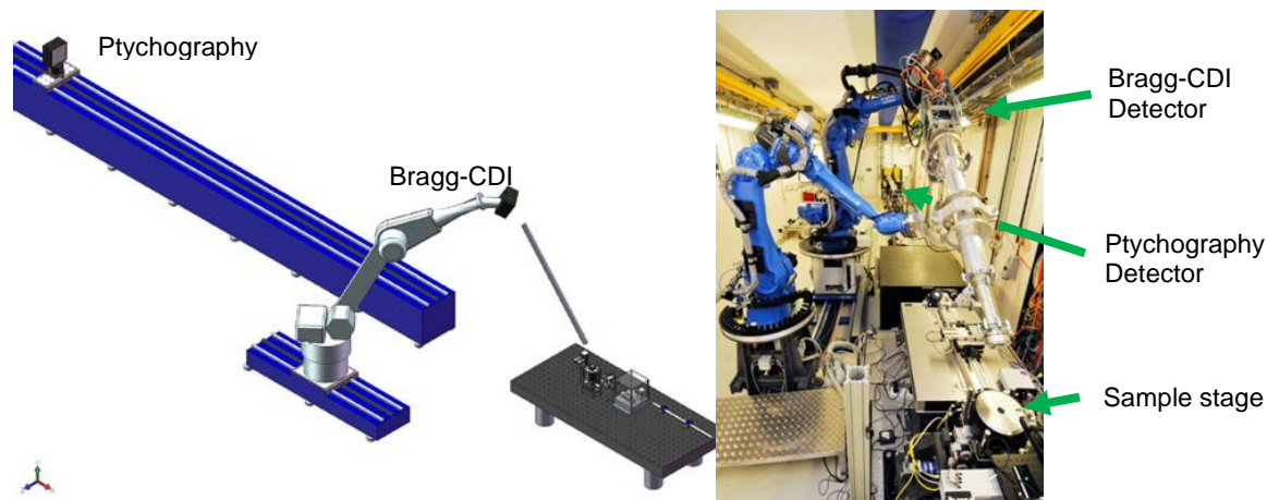
Figure 1: Left: Scheme for experimental setup on coherence branch. Right: Image of experimental hutch. In foreground sample stage, robot arm and detector for Bragg CDI. In the far background at the end of the hutch the ptychography detector is located.
