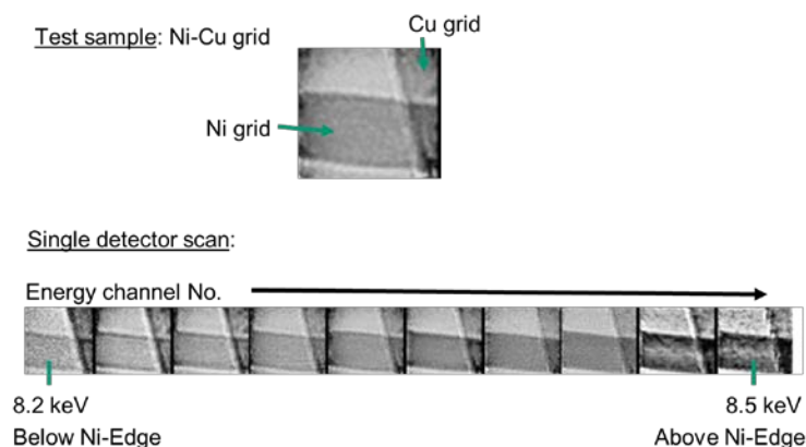
Figure 2: Image series extracted from single ptychographic scan using energy selective SLcam hyper-spectral detector. Test sample consists of a stacked copper and nickel grid, the latter can be identified by its absorption edge [16].
