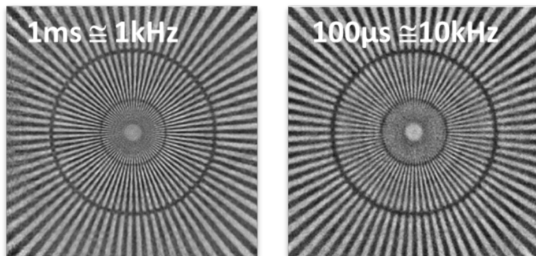
Figure 3: Reconstructed data of Siemens star with short exposure times, left 1ms, right 100 \mu\text{s} . The latter proves the feasibility of scanning at 10kHz rate. The two circular indicator lines are positioned at spoke separations of 200 and 100nm [11].
