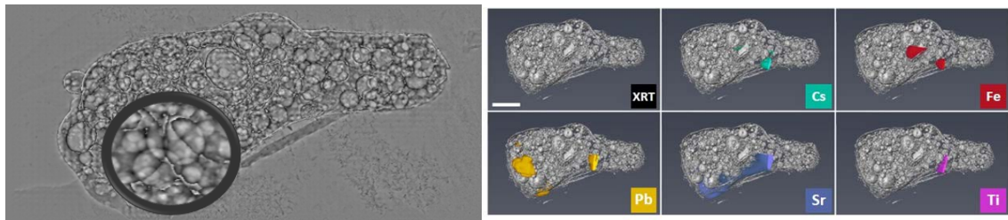
Figure 5: Example of multi-scale and multi-modal imaging; study of fall-out particle from Fukushima accident. Left: ptychographic reconstruction of single projection. Right: 3D rendering of micro-tomographic data (upper left) and correlation of different elements detected by fluorescence [26].
