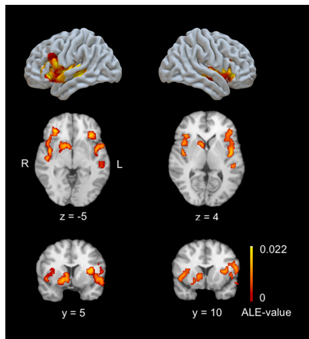
Fig. 2. Brain regions involved in the conjunction analysis of FTD and music perception. z = axial location of x,y,z coordinates. y = coronal location of x,y,z coordinates. The ALE-scores are demonstrated. For the coordinates and brain regions see Table 4. All results were thresholded at a cluster-wise threshold of p < 0.05 (FWE-corrected).
