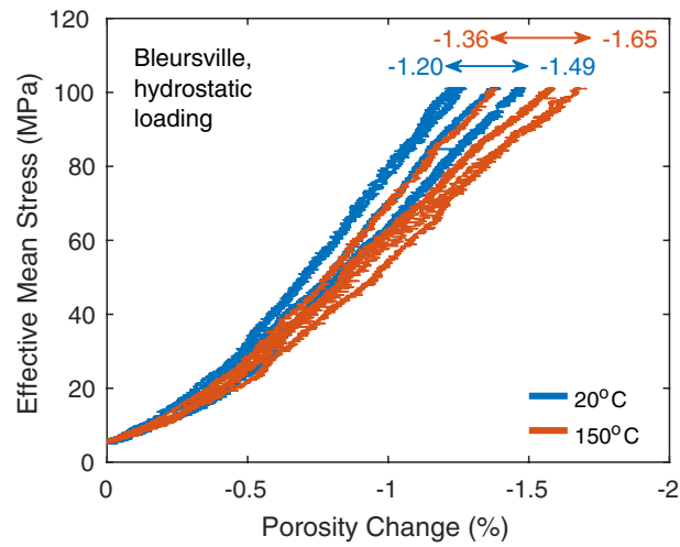
Figure A1. Porosity change as a function of effective mean stress for the hydrostatic loading of Bleursville sandstone from 10 to 100 MPa. Blue curves indicate room temperature tests and red curves represent experiments carried out at 150°C.
