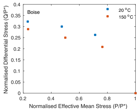
Figure 15. The yield envelope of Boise sandstone with the values of both differential stress and effective mean stress normalized by the P^* stress value.
