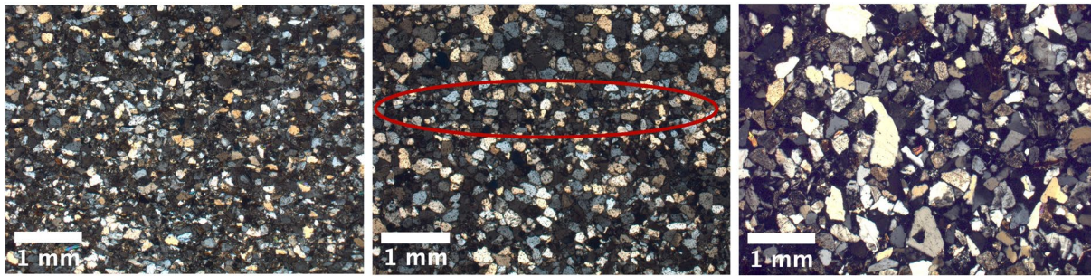
Figure 1. Micrograph images of undeformed sample of Bleurville (left), Locharbriggs (center), and Boise (right). The red ellipse in the center image highlights a region of Locharbriggs sandstone where the grain diameter is smaller by a factor of about two, which corresponds to sub-millimeter dark bands present in the undeformed Locharbriggs samples.
