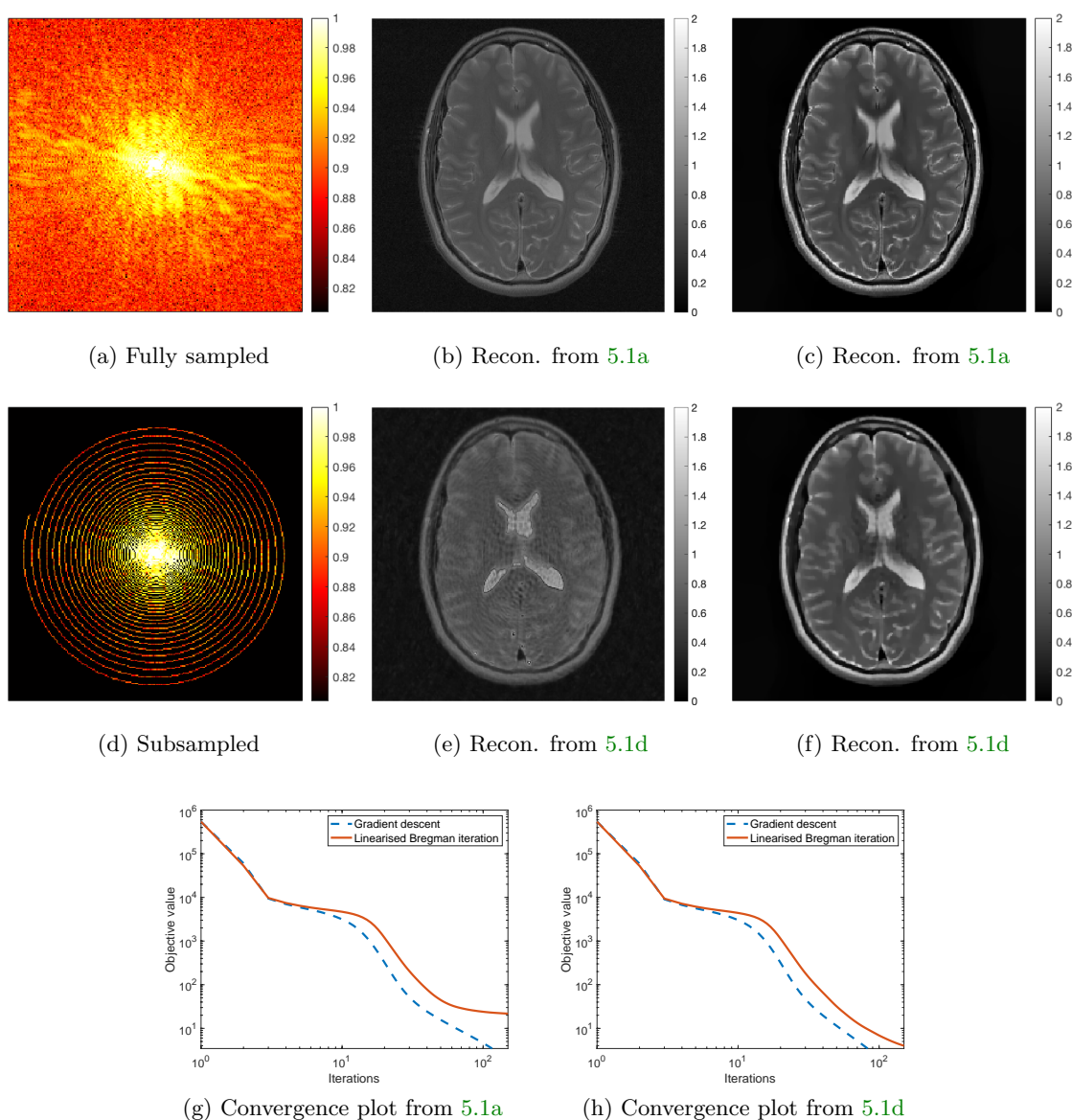
Figure 5.1. Figure 5.1(a) shows a log-plot of the modulus of the fully sampled k -space data of the first coil taken from [48]. Figure 5.1(b) shows the reconstruction of the spin proton density from the data visualized in Figure 5.1(a) via gradient descent, whereas Figure 5.1(c) shows the reconstruction of the spin proton density from the same data but via Algorithm 3.2. In Figure 5.1(d) we see roughly 25% of the k -space data visualized in Figure 5.1(a), sampled on a spiral on a cartesian grid [11]. Figure 5.1(e) shows the reconstruction of the spin proton density from this subsampled k -space data with gradient descent, while Figure 5.1(f) shows the reconstruction of the spin proton density from the same data but with Algorithm 3.2. Figures 5.1(g) and 5.1(h) show the convergence plots in terms of energy decrease per iteration for the reconstructions that are obtained from the k -space data shown in Figure 5.1(a), respectively, in Figure 5.1(d).
