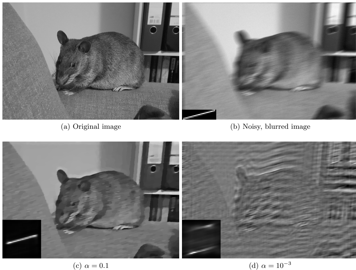
Figure 6.1. Figure 6.1(a) shows an image of Pixel the Gambian pouched rat. Figure 6.1(b) shows a motion-blurred version of that image, together with some added normal distributed noise. The corresponding convolution kernel is depicted in the bottom left corner. Figure 6.1(c) visualizes the reconstruction of the image and the convolution kernel with Algorithm 3.2 for the choice \alpha = 10^{-1} . Figure 6.1(d) shows the reconstructions of the same quantities for the choice \alpha = 10^{-3} . We clearly see that a larger choice of \alpha results in a regular solution, whereas a smaller \alpha will mimic traditional gradient descent with almost no additional regularity of the reconstruction.
