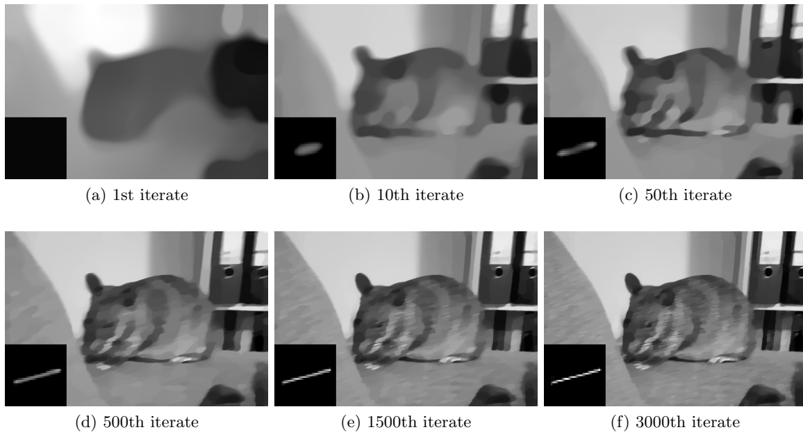
Figure 2.2. Proposed approach for blind deconvolution. Several iterates of the linearized Bregman iteration (2.6) for the choice \alpha = 0.05 . The strong initial effect of the total variation regularization enables the algorithm to converge to a solution close to \hat{u} and \hat{h} .
