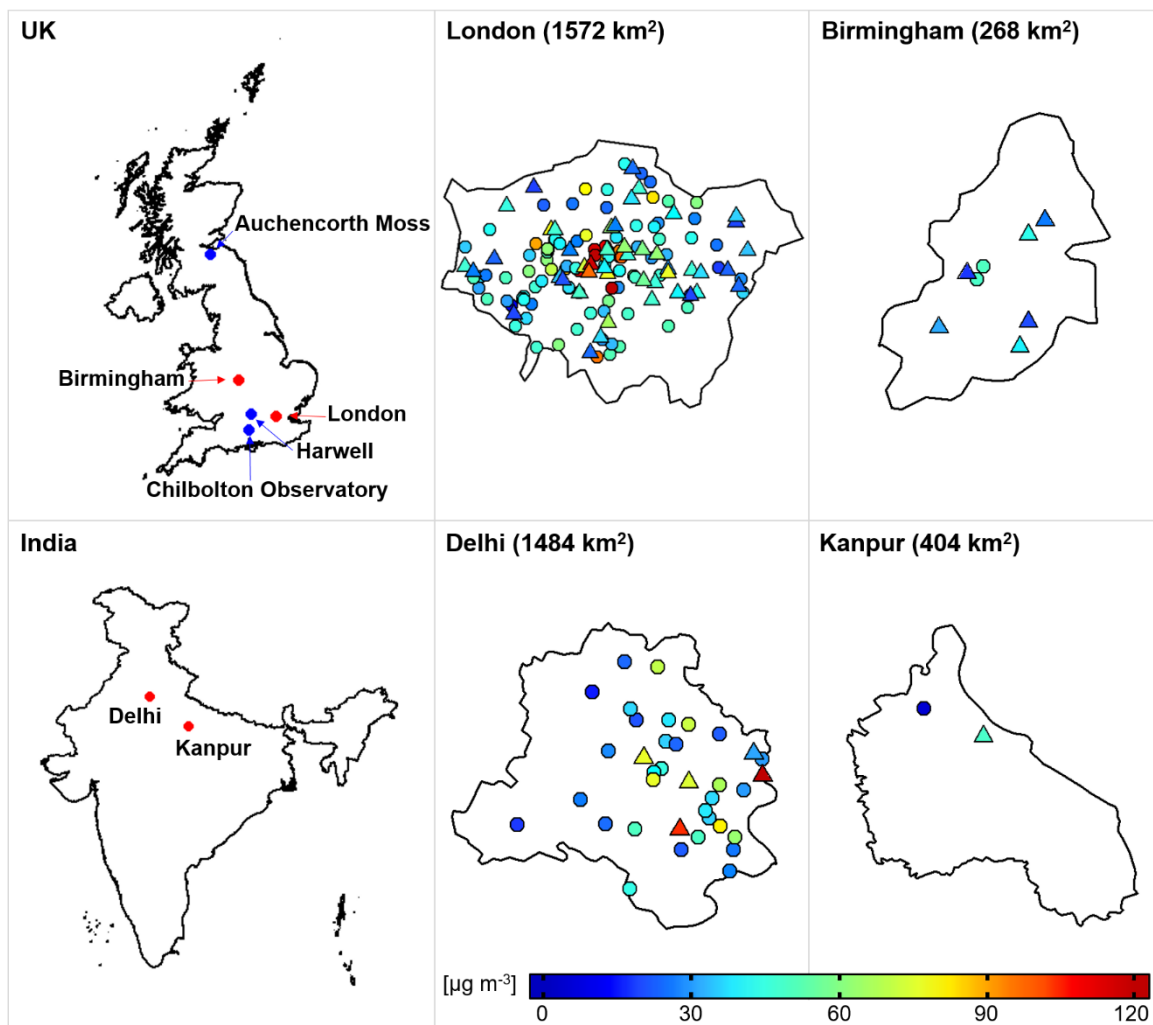
1130 Figure 1 Spatial extent of surface NO 2 monitoring stations in London, Birmingham, Delhi, and Kanpur. The left panel shows the location of the target cities (red) and UK sites that are part of the European Monitoring and Evaluation Programme (EMEP) (blue). The centre and right panels show the locations of local authority regulatory NO 2 monitoring stations within the administrative boundaries of each city, coloured by mean midday NO 2 for 2005-2018, and separated into sites used (triangles) and not used (circles) to assess satellite observations of NO 2 (see text for details). The surface area of each city is indicated. Country and city boundaries are from GADM version 3.6 (GADM, 2018) and DataMeet (DataMeet, 2018).
