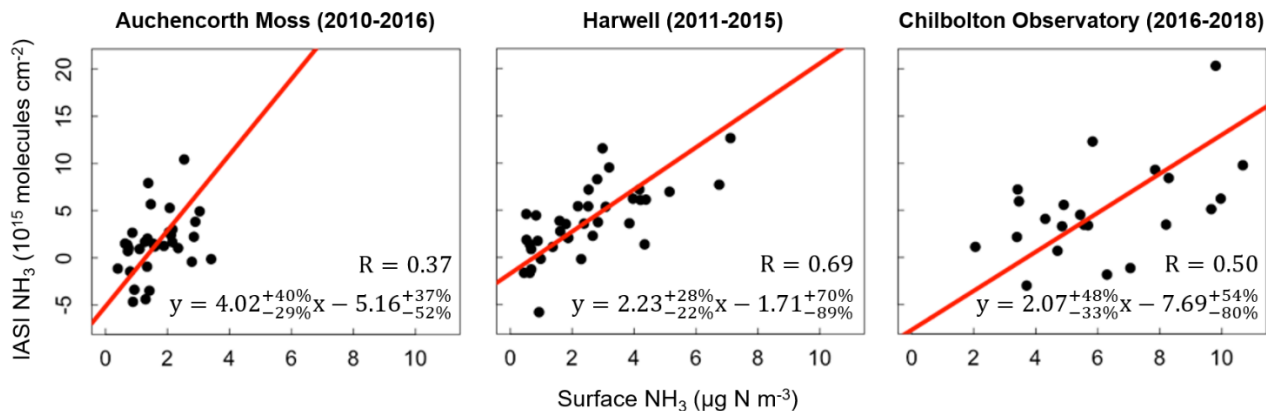
Figure 3 Assessment of IASI \text{NH}_3 with ground-based \text{NH}_3 at UK EMEP sites. Points are monthly means from IASI and the surface sites Auchencorth Moss (left), Harwell (middle) and Chilbolton Observatory (right). The red line is the SMA regression. Values inset are Pearson's correlation coefficients and regression statistics. Relative errors on the slope and intercept are the 95 % CI. Locations of UK EMEP sites are indicated in Figure 1.
