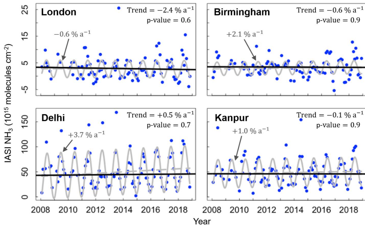
1165 Figure 8 Time series of IASI \text{NH}_3 in 2008-2018 for London, Birmingham, Delhi and Kanpur. Points are city-average monthly means. Black lines are trends obtained with the Theil-Sen single median estimator. The grey lines are the fit (solid) and trend component ( B ) (dashed) obtained with Equation (1). Values inset are annual trends and p-values for the Theil-Sen fit (in black) and annual trends obtained with Equation (1) (grey). Trend errors (not shown) exceed \pm 150\% in all cities.
