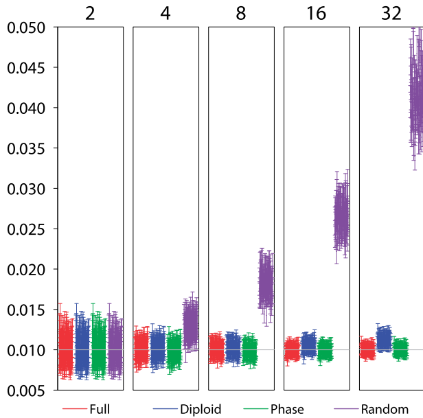
FIGURE 6. The 95% HPDCIs for parameter \theta in the single-population coalescent model in 100 replicate datasets using four phase-resolution strategies: F (the full data), D (diploid), P (PHASE), and R (random). There are 100 independent loci in each data set, and at each locus there are S sequences of 500 sites (or S/2 diploid individuals), with S=2, 4, 8, 16 , and 32 . The true parameter value is 0.01 .
