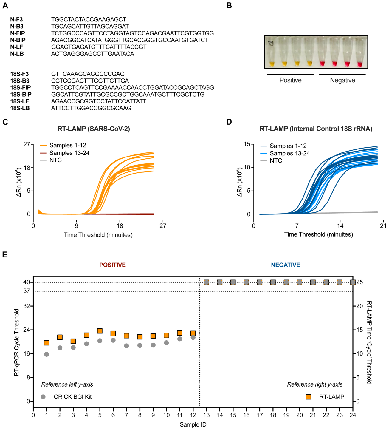
Figure 1. Validation of SARS-CoV-2 detection by RT-LAMP targeting the N gene. (A) The N gene of SARS-CoV-2 was targeted using primers designed by Zhang et al. 10 , whilst the internal control utilised primers for 18S rRNA initially published by Lamb et al. 9 . (B) Upon DNA amplification, a colorimetric pH dye in the reaction mix will change from pink to yellow if the target is present. Four SARS-CoV-2 positive and four SARS-CoV-2 negative patient samples are shown (sideview of PCR tubes). (C–D) Amplification curves from 24 patient samples assessed by SARS-CoV-2 (N gene) RT-LAMP (C) or 18S (D) in a Real-Time PCR machine. (E) Dot plot of the SARS-CoV-2 Ct values from (C–D) compared to Ct values derived from the Crick’s RT-qPCR diagnostic pipeline using the CE marked BGI kit. Ct values of ‘undetermined’ are plotted as “Ct = 40” (left y-axis) or “Ct = 25” (right y-axis) for illustrative purposes. Data are normalised by assay run/cycles determined by the two methods for comparative purposes. The clinical call from the reference laboratory is indicated above the graph.
