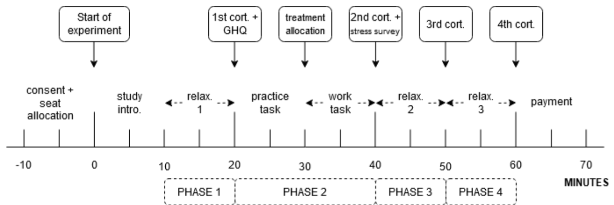
Figure 1. Experiment timeline
