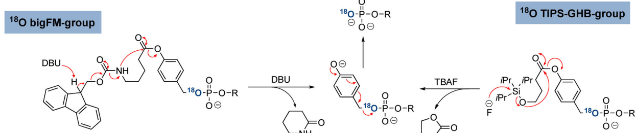
Scheme 3. Synthesis of ^{18}\text{O} -P-amidites (A,B). Self-immolation of novel phosphate protecting groups after the trigger (C). Abbreviations: AB: para -acetoxybenzyl; PMB: para -methoxybenzyl, DCM: dichloromethane; ETT: 5-ethylthio-1 H -tetrazole.
