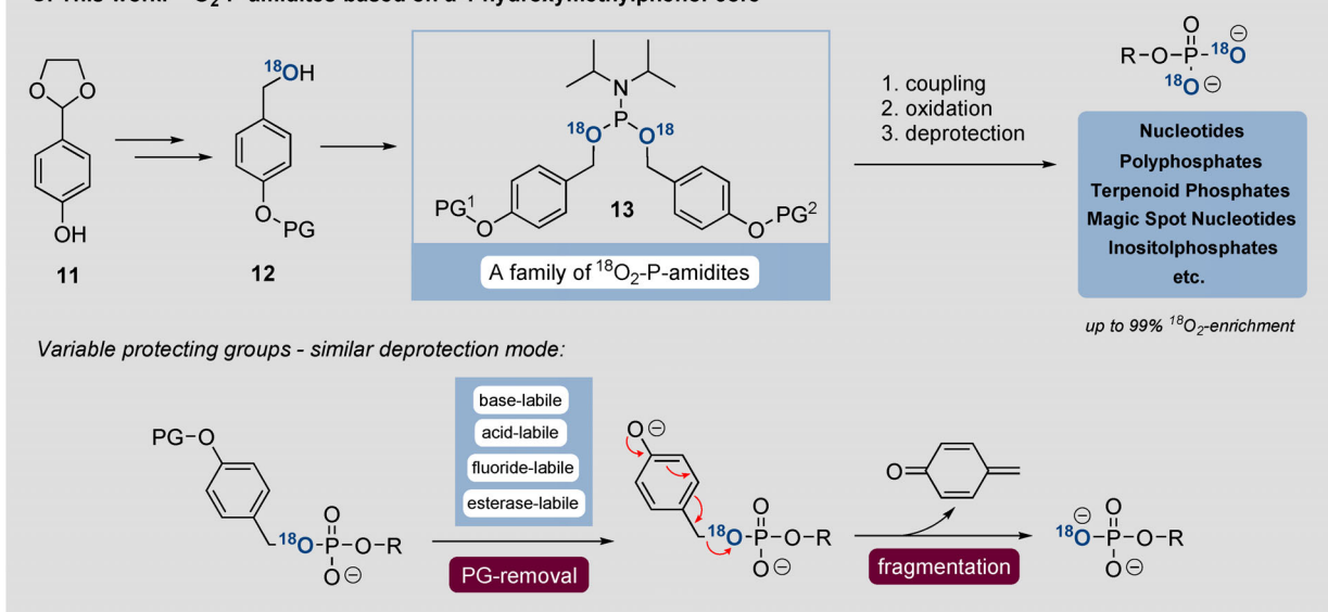
Scheme 1. A) hydrolytic approaches towards 18 O 4 -phosphates. B) Application of (Bn 18 O) 2 -P-amidite towards labelled NTPs. C) New synthetic concept towards 18 O 2 -phosphates. The general deprotection mode of all 18 O-P-amidites developed is shown.
