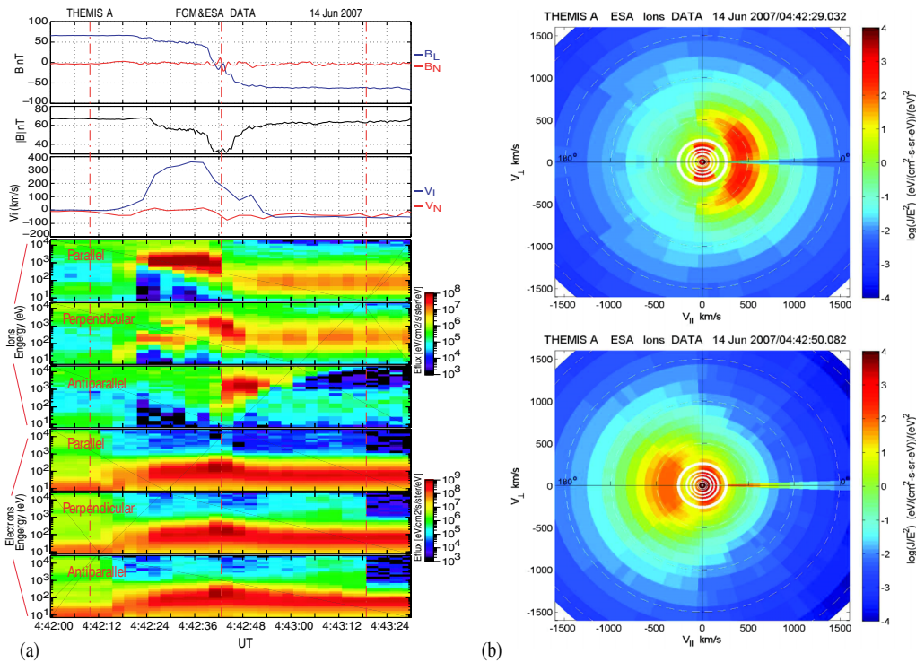
FIG. 3 (color online). (a) THEMIS-A energy spectra for both ions and electrons, separated into angular ranges surrounding the directions parallel, perpendicular and antiparallel to the magnetic field. The six lower panels on the left show these data for the time interval surrounding the boundary crossing, with the magnetic field magnitude, B_N and B_L components, and V_L and V_N , the bulk ion flows, shown in the top three panels. The three vertical dashed lines indicate the inner and outer boundaries of the reconnection layer and the location of the current sheet (middle line). (b) Shows the 2-D ion velocity, perpendicular and parallel to the magnetic field, for times either side of the current sheet. These distributions are reflected about V_{\perp} = 0 .
