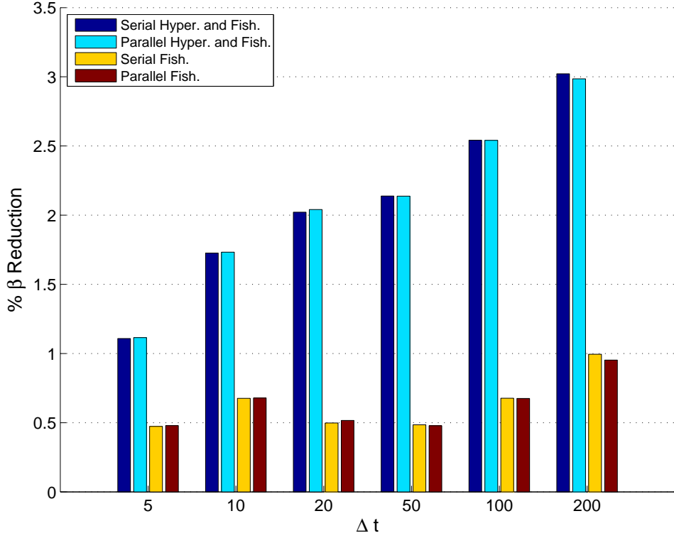
Figure 29: % \beta reduction from Kernel Learning for Subset B
