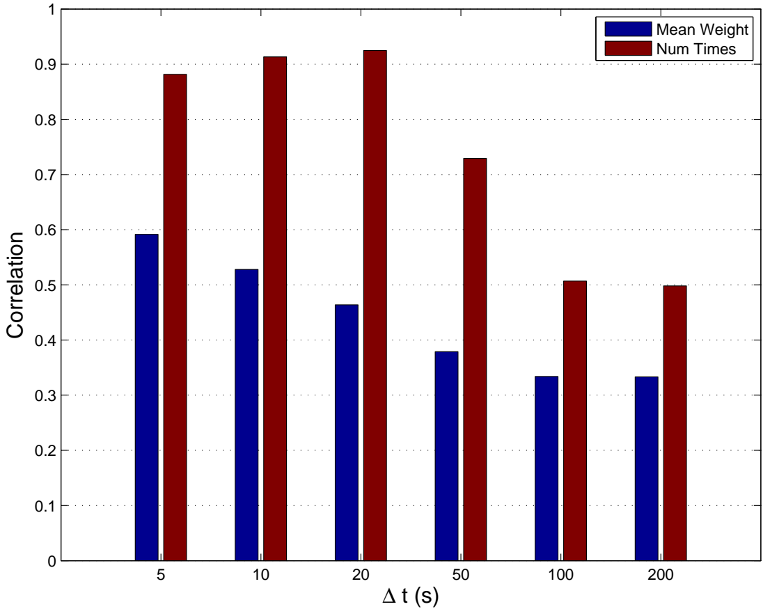
Figure 16: Correlation of MKL average weighting & number of times included vs % accuracy
