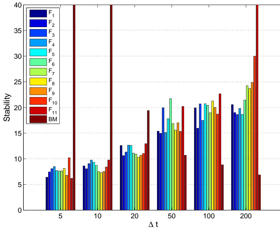
Figure 13: Stability of individual SVM by feature type
