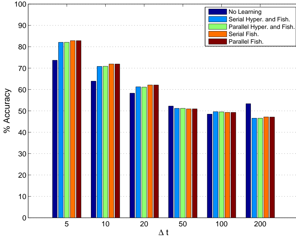
Figure 26: Comparison of % accuracy between kernel learning methods for Subset B
