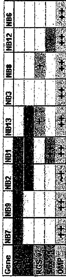
Southern Blot
