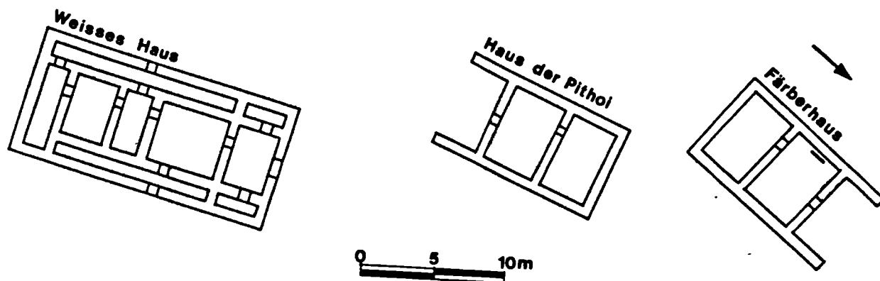
a. Structures of Aigina III ( After Hagg & Konsola 1986, fig. 7 )
