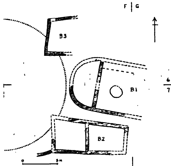
b. Lerna IV: Structures of the 2nd Phase.
