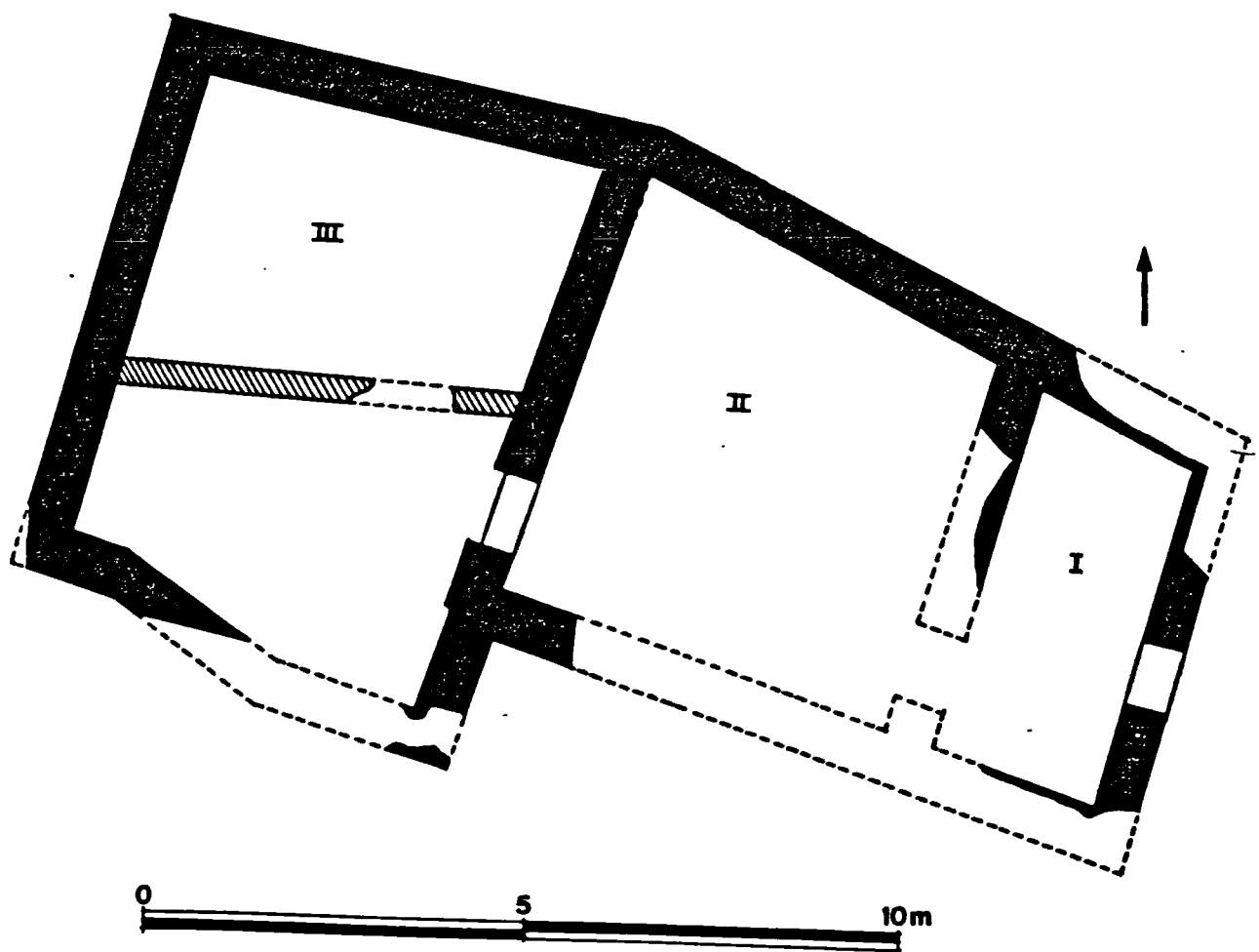
b. Eutresis. Building L ( After Hagg & Konsola 1986, fig. 30 ) FIG. 42
