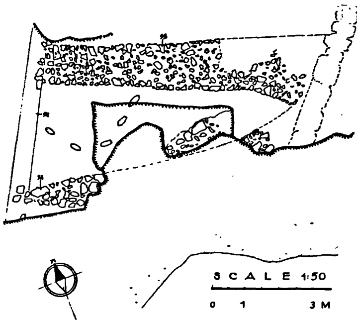
b. Structure J, at Ay. Kosmas ( After Mylonas 1959, fig. 12 )
