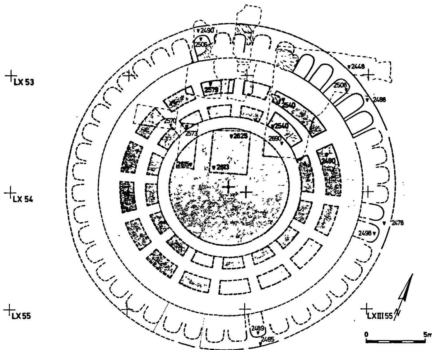
The " Rundbau ". Restored ground plan. ( After Hagg & Konsola 1986 ) FIG. 48 Tiryns
