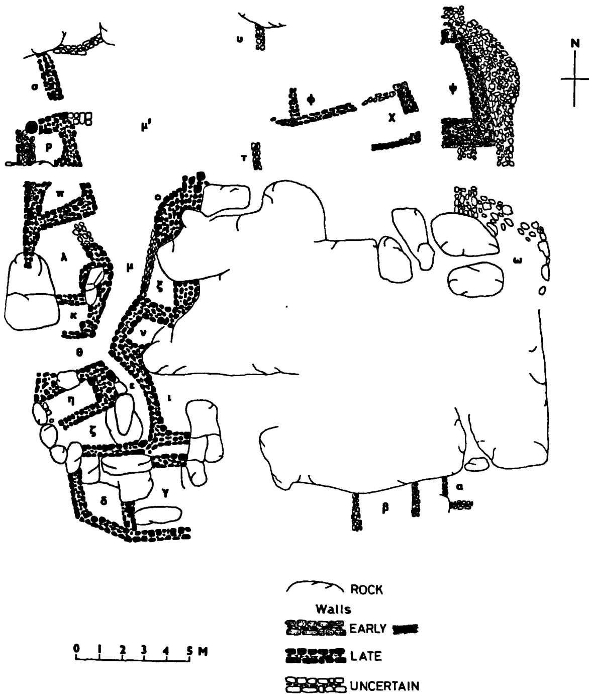
Mt.Kynthos on Delos. Plan of the Early Cycladic Settlement. (after Plassart 1928, Plan III).
