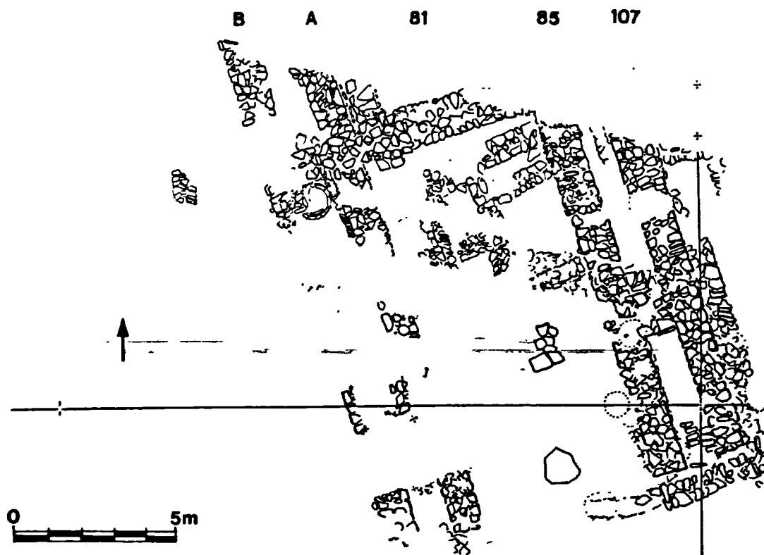
b. Plan of Building BG of Lerna IIIC ( After Hagg & Konsola 1986 )
