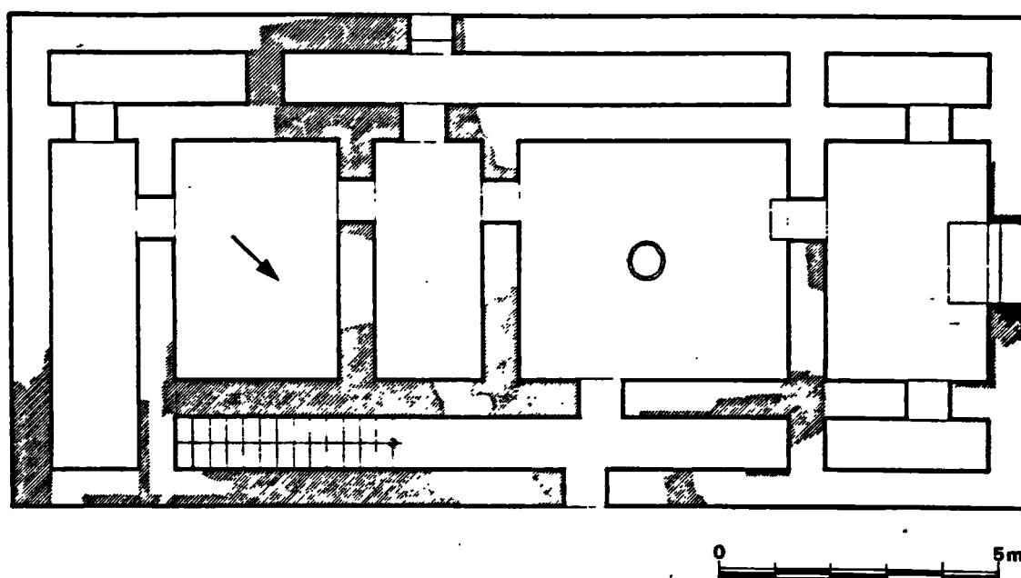
b. Ground Plan of the "Weisses Haus" ( After Hagg & Konsola 1986, fig. 8 )
