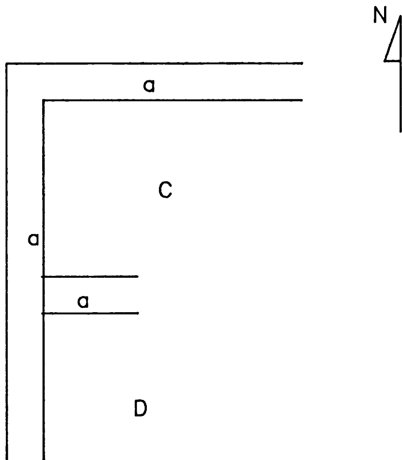
PYRGOS-PAROS House C-D (Walls a) EC II Period Scale 1:50
