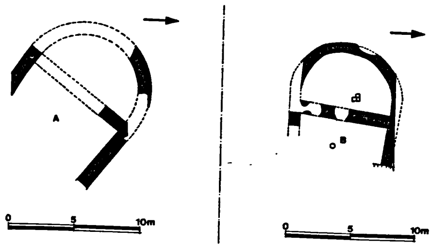
a. Thebes. Apsidal Buildings A and B. ( After Hagg & Konsola 1986, fig. 52 )
