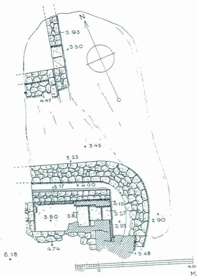
b. Paroikia on Paros. The Architectural Remains at the foot of the hill. ( After Rubensohn 1917, Abb. 6 )
