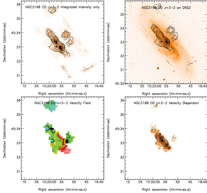
Figure C8. CO J = 3-2 images for NGC 3198. (a) CO J = 3-2 integrated intensity image. Contours levels are (0.5, 1, 2, 4, 8) \text{K km s}^{-1} ( T_{\text{MB}} ). (b) CO J = 3-2 overlaid on a Digitized Sky Survey image. (c) Velocity field. Contour levels are (606, 636, 666, 696, 726, 756) \text{km s}^{-1} . (d) The velocity dispersion \sigma_v as traced by the CO J = 3-2 second moment map. Contour levels are (4, 8, 16, 32) \text{km s}^{-1} .
