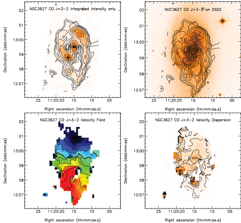
Figure C11. CO J = 3-2 images for NGC 3627. (a) CO J = 3-2 integrated intensity image. Contours levels are (0.5, 1, 2, 4, 8, 16, 32) \text{K km s}^{-1} ( T_{\text{MB}} ). (b) CO J = 3-2 overlaid on a Digitized Sky Survey image. (c) Velocity field. Contour levels are (559, 605, 651, 697, 743, 789, 835, 881) \text{km s}^{-1} . (d) The velocity dispersion \sigma_v as traced by the CO J = 3-2 second moment map. Contour levels are (4, 8, 16, 32, 64, 128) \text{km s}^{-1} . Similar images derived from the same data have been published in Warren et al. (2010).
