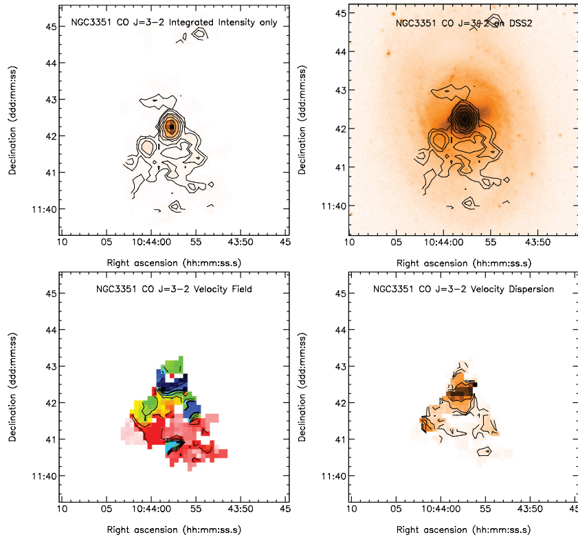
Figure C9. CO J = 3-2 images for NGC 3351. (a) CO J = 3-2 integrated intensity image. Contours levels are (0.5, 1, 2, 4, 8, 16, 32) \text{K km s}^{-1} ( T_{\text{MB}} ). (b) CO J = 3-2 overlaid on a Digitized Sky Survey image. (c) Velocity field. Contour levels are (702, 735, 768, 801, 834, 867, 900) \text{km s}^{-1} . (d) The velocity dispersion \sigma_v as traced by the CO J = 3-2 second moment map. Contour levels are (4, 8, 16, 32, 64) \text{km s}^{-1} .
