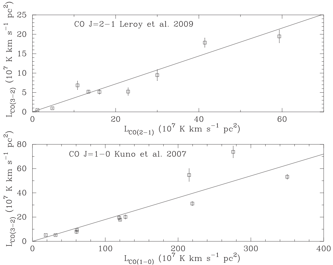
Figure 2. Top: L_{\text{CO}(3-2)} versus L_{\text{CO}(2-1)} for all galaxies detected in both the NGLS and the HERACLES surveys (Leroy et al. 2009). The HERACLES luminosities have been adjusted to use the distances adopted in this paper. Calibration uncertainties in the HERACLES data are estimated at 20 per cent (Leroy et al. 2009). The line shows the mean CO J = 3-2/2-1 ratio of 0.36 determined from the data points (see text). Bottom: L_{\text{CO}(3-2)} versus L_{\text{CO}(1-0)} for all galaxies detected in both the NGLS and the survey of Kuno et al. (2007). The CO J = 1-0 luminosities have been adjusted to use the distances adopted in this paper. The line shows the mean CO J = 3-2/1-0 ratio of 0.18 determined from the data points (see text).
