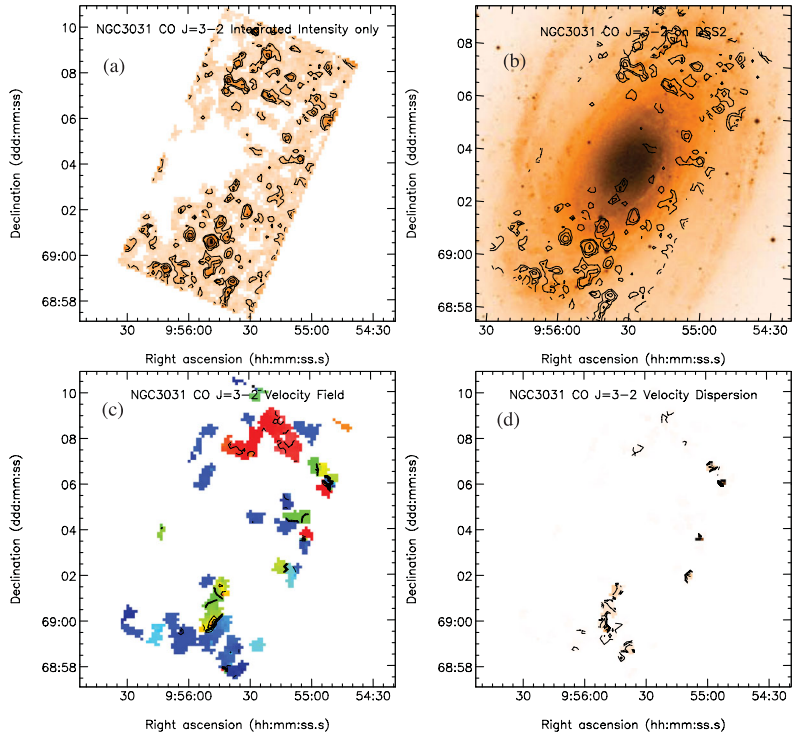
Figure C5. CO J = 3-2 images for NGC 3031. (a) CO J = 3-2 integrated intensity image. Contour levels are (0.5, 1, 2, 4) \text{K km s}^{-1} ( T_{\text{MB}} ). (b) CO J = 3-2 overlaid on a Digitized Sky Survey image. (c) Velocity field. Contour levels are (-328, -258, -188, -118, -48, 22, 92, 162) \text{km s}^{-1} . (d) The velocity dispersion \sigma_v as traced by the CO J = 3-2 second moment map. Contour levels are (4, 8, 16, 32, 64, 128) \text{km s}^{-1} . Images derived from the same data using careful flagging and analysis to detect weak but real features have been published in Sanchez-Gallego et al. (2011).
