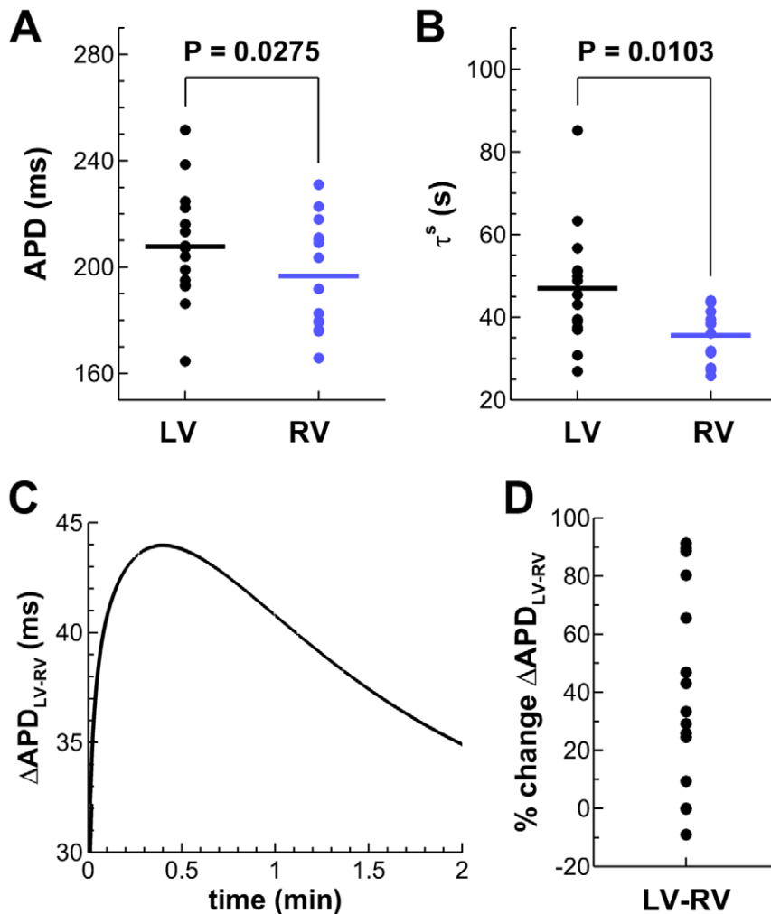
Figure 3. Functional LV/RV differences in the in vivo human heart. A,B: Unipolar electrograms revealed longer steady-state APDs at the study CL and slower APD adaptation dynamics in LV compared to RV. C: Transient increased LV/RV APD dispersion following rate acceleration in a representative patient (Patient 3). D: Percent of \Delta\text{APD}_{\text{LV-RV}} increase following rate acceleration for all patients of the study. doi:10.1371/journal.pone.0052234.g003
