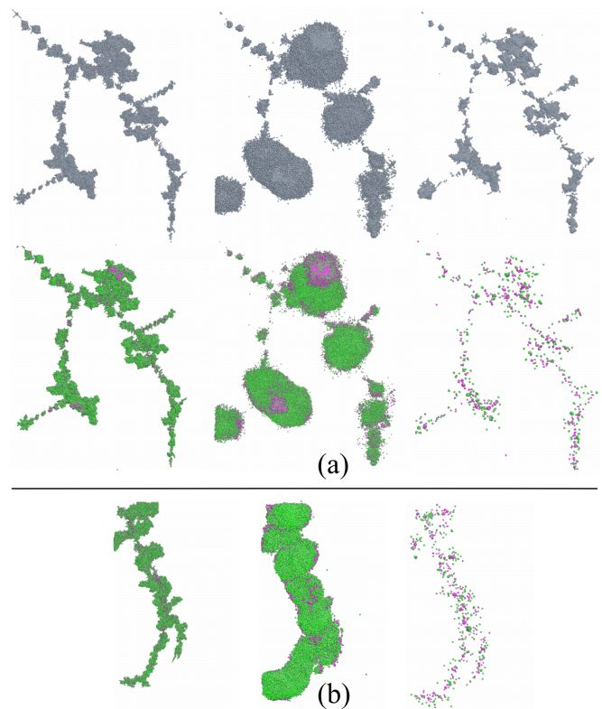
FIG. 3: (a) and (b) show two representative 0.5 MeV cascades. The knock-on atom moves from the top left to the bottom right corner. In (a) we show both displaced (top) and defect (bottom) atoms at 0.2, 1.5 ps and 100 ps. In (b) we show the defect atoms only at 0.3 ps, 2 ps and 100 ps. Cascade size in (a) and (b) is 950 Å and 1300 Å, respectively.
