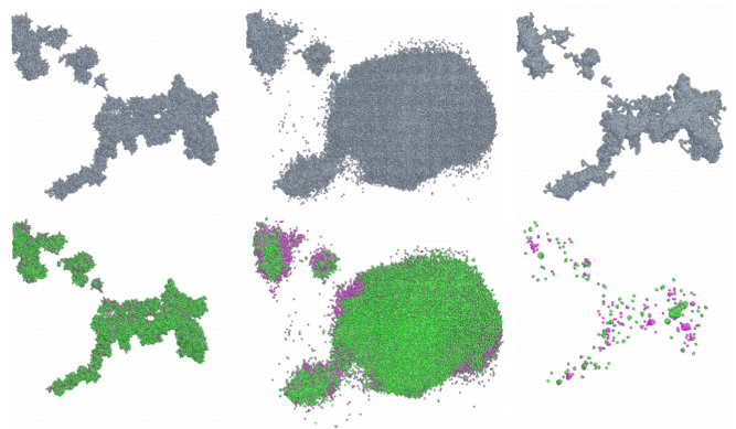
FIG. 2: Displaced (top) and defect (bottom) atoms in a representative 0.2 MeV collision cascade. The knock-on atom moves from the top left to the bottom right corner. The three frames for each type of atoms correspond to 0.3 ps, 3 ps and 80 ps, respectively. Cascade size (maximal separation between any two atoms in the cascade) is 560 Å. Vacancies (interstitials) are represented in purple (green); we used Atomeye software 27 to visualize cascade evolution.
