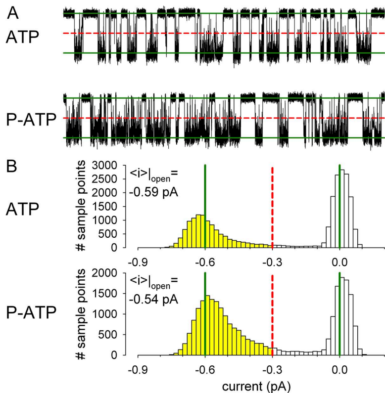
Figure S1. Average unitary conductance is smaller for channels opened by P-ATP. (A) 25-s segments of recording of a single WT CFTR channel gating first in ATP (top) and then in P-ATP (bottom); V_m = -80 mV. Solid green lines, conductance levels used for idealization; dotted red line, half-amplitude threshold. (B) Amplitude histograms for the segments of record shown in A. Bins corresponding to data points above the idealization threshold (red dotted lines) are highlighted in yellow. Average currents for such data points (i.e., during idealized “open” events) are plotted in each panel.
