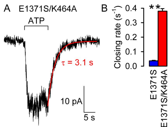
Figure S2. The K464A mutation accelerates nonhydrolytic closure of E1371S CFTR. (A) Macroscopic current of prephosphorylated E1371S/K464A CFTR channels elicited by transient exposure (bar) to 10 mM ATP. Current decay time course upon sudden ATP removal was fitted with a single exponential (red solid line); time constant (in seconds) reflects mean burst duration. (B) Nonhydrolytic closing rate of E1371S/K464A (red bar), calculated as the inverse of the decay time constant upon ATP removal. As a comparison, E1371S closing rate (blue bar) is re-plotted from Fig. 3 F.
