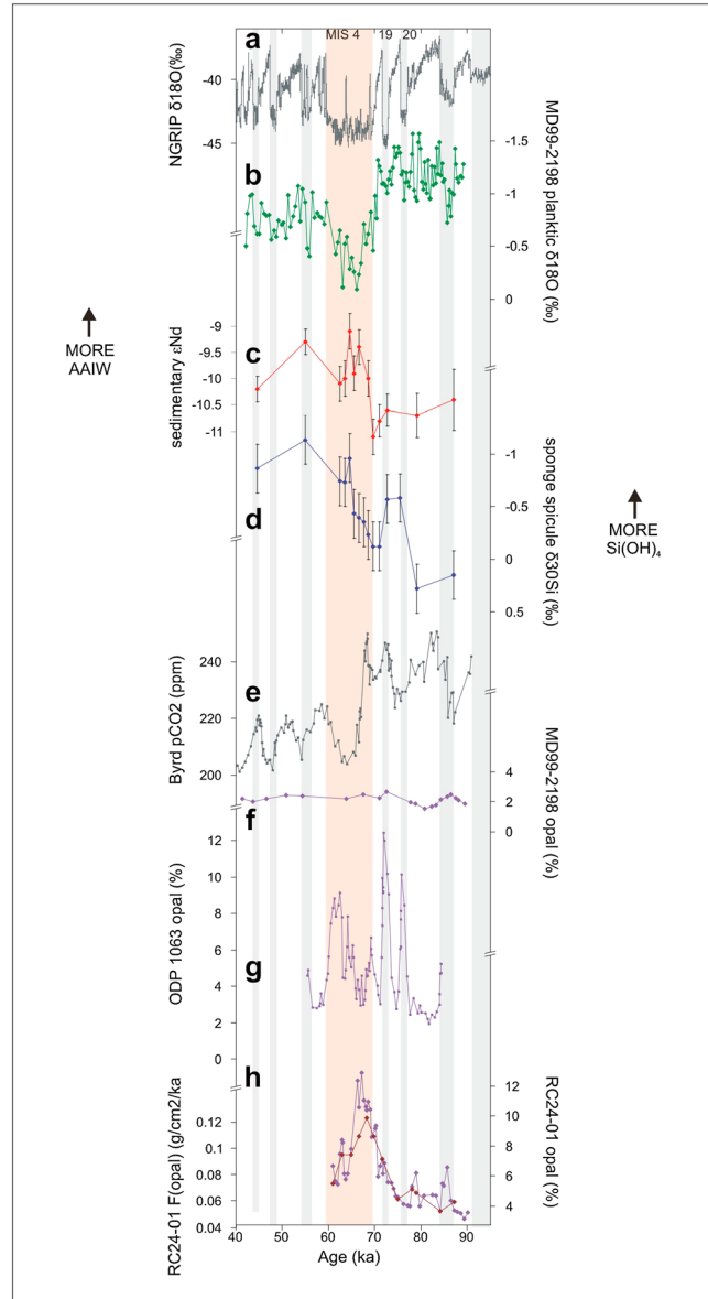
Figure 5. (a) NGRIP \delta^{18}\text{O} [Andersen et al. , 2007], adjusted to the Hulu-Sanbao speleothem record [Wang et al. , 2001, 2008]. (b) MD99-2198 planktic \delta^{18}\text{O} (‰) (green curve). (c) MD99-2198 sedimentary \epsilon_{\text{Nd}} (red curve); error bars are 2 sigma standard deviation at the 95% confidence limit ( 2\sigma\text{SD} ). (d) MD99-2198 sponge spicule \delta^{30}\text{Si} (blue curve); error bars are 2\sigma\text{SD} . (e) Byrd (Antarctica) ice core p\text{CO}_2 [Ahn and Brook, 2008]. (f) MD99-2198 opal (%) (purple curve). (g) ODP 1063 opal (%) (purple curve). (h) RC24-01 opal (%) (purple curve), overlain with RC24-01 thorium-normalized preserved opal flux rate ( \text{g}/\text{cm}^2/\text{ka} ) (brown curve). All percent opal measurements are plotted on the same y axis. Northern Hemisphere cold periods are marked by grey bands, and MIS 4 (light orange shading) and cold D-O 19 and 20 are annotated.
