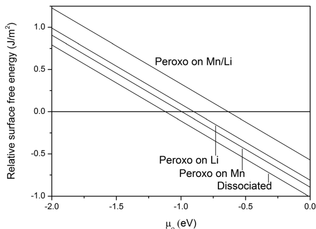
Fig. 11 Surface free energies of the oxidised Li/MnO 2 (110) surfaces with respect to the non-oxidised termination.
