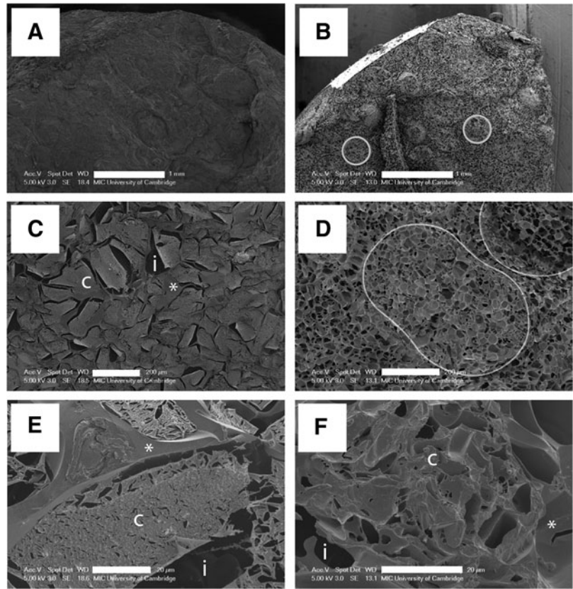
FIG. 4. Cryoscanning electron microscopy of fractured cryovials after cooling at a linear rate of 1^{\circ}\text{C}/\text{min} . Ultrastructure resulting from controlled ice nucleation ( A , C , E ) is compared to spontaneous ice nucleation ( B , D , F ). In all samples the spaces originally occupied by ice crystals are revealed as voids following sublimation of ice. In figures ( B , D ) sectioned alginate beads that are \sim 500\ \mu\text{m} in diameter are outlined. In ( C , E , F ), cell clusters (c), ice voids (i), and smooth freeze concentrated alginate and cryoprotectant (CPA) (*) have been labeled. Scale bars on ( A , B ) 1 mm, on ( C , D ) 200 \mu\text{m} , and on ( E , F ) 20 \mu\text{m} .
