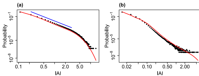
Fig. 14 Distribution of IAI for the system driven from subcritical and supercritical states. The theoretical (red) and simulated (black) IAI distributions with \alpha = 1.1 (subcritical) (a) and \alpha = 0.9 (supercritical) (b) parameters. The blue line in a indicates a linear fit, i.e. a fitted power law with an exponent of 2.37. These distributions are with N = 800 , w = 1 , h = 1/N and the theoretical distributions were calculated up to a level of initial active neurons which occur with a cumulative probability of 0.9 and 0.13, respectively (see main text)
