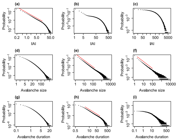
Fig. 17 IAI, avalanche size and duration distributions for the system with the saturating activation function. The distributions are for simulations with h = 1/N ( a , d , g ), h = 0.1/N ( b , e , h ) and h = 0.01/N ( c , f , i ). For all simulations N = 800 , \alpha = 0.25 , w = 1 and the distributions are pooled from 10 simulations each of length 10^4 seconds. The red lines indicate linear fits on the double logarithmic scale, i.e. fitted power laws with exponents of 2.65 ( a ), 1.81 ( e ), 1.49 ( f ) and 1.84 ( h )
