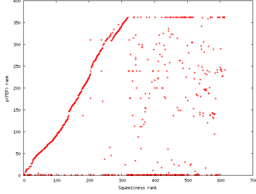
Figure 3: The rank correlation of p(\text{FEP}) and Squeeziness for all programs (EXP2).
