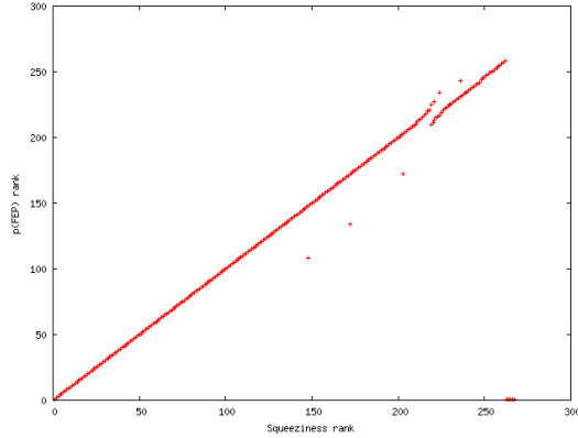
Figure 4: The rank correlation of p(\text{FEP}) and Squeeziness for statistical programs (EXP2).
