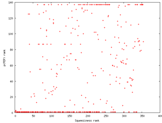
Figure 5: The rank correlation of p(\text{FEP}) and Squeeziness for small programs (EXP2).
