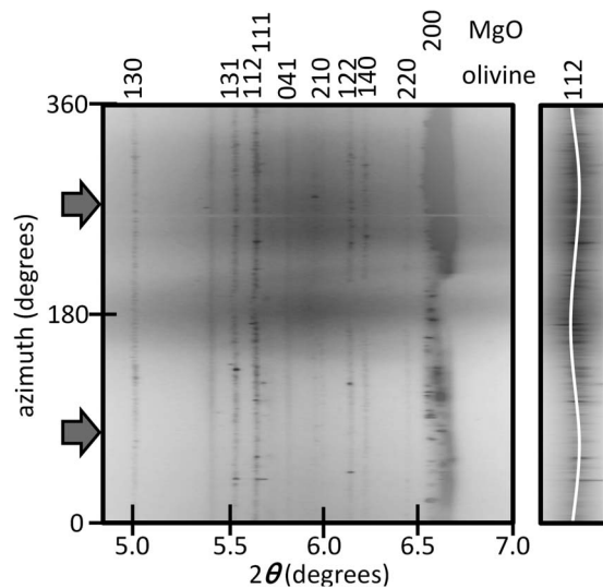
FIG. 6. Sample olivine diffraction pattern from experiment SiO_43 (445 kN) during deformation at 800 °C. The diffraction pattern has been unwrapped to allow distortions of the Debye rings to be recognised. The vertical axis is the angle of the diffraction vector from horizontal (0°). The grey arrows at 90° and 270° denote the orientation of the maximum stress direction, which are vertical in the press; the differential stress was measured to be 1.0 \pm 0.3 GPa. Despite the boron epoxy windows significantly improving the pattern, there are still diffraction peaks from MgO, graphite, and crushable alumina present in the diffraction pattern. The doubling of the MgO {200} peak arises because the MgO is up-stream and down-stream of the sample making two different volumes with different “sample”–detector distances; the unindexed diffraction peaks are from the graphite heater and crushable alumina insulating sleeve. On the right-hand side the sub-figure expands {112} olivine diffraction peak and highlights its modulations due to the applied stress.
