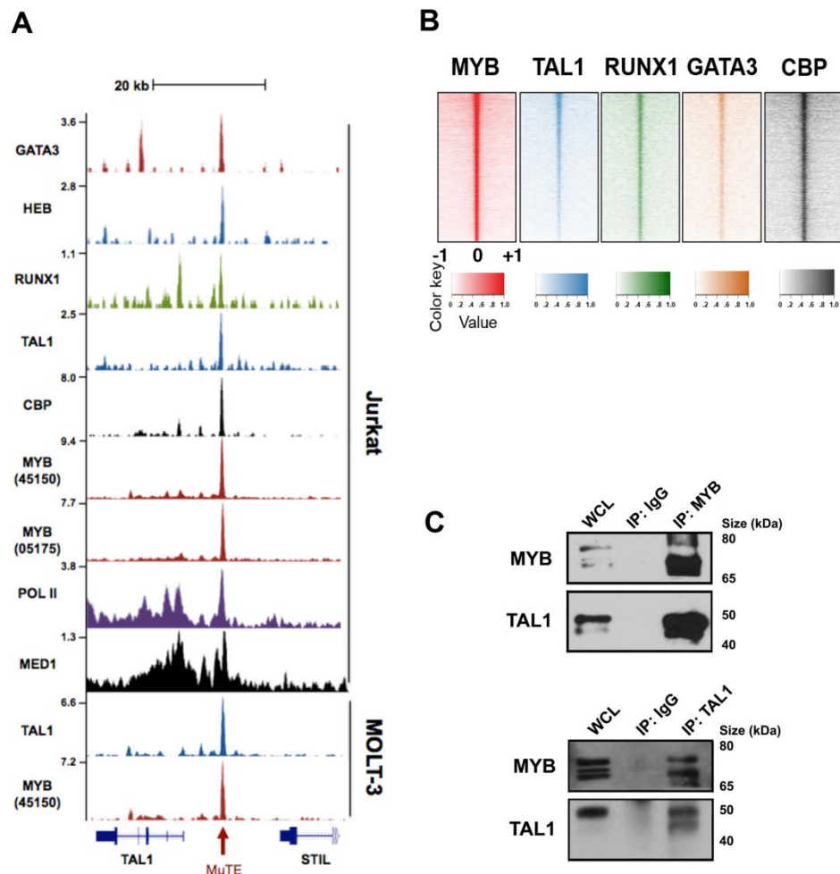
Fig. 3. MYB binds the mutant TAL1 enhancer site and is a member of the TAL1 complex. (A) ChIP-seq tracks at the STIL-TAL1 locus from Jurkat and MOLT-3 T-ALL cells for GATA3, HEB, RUNX1, TAL1, CBP, MYB (ab45150 antibody), MYB (05-175 antibody), RNA polymerase II (Pol II), and Mediator 1 (MED1). The mutation site at -7.5 kb is depicted with a red arrow. ChIP-seq read densities (y-axis) were normalized to reads per million reads sequenced in each sample. (B) Heatmaps showing genome-wide co-occupancy of MYB binding sites (+/- 1 kb) with those from TAL1, RUNX1, GATA3, and CBP sites as determined by ChIP-seq. For each region (y axis), the sequence density centered at 0 indicates overlapping bound regions. (C) Co-immunoprecipitation (Co-IP) and reciprocal Co-IP experiments performed from Jurkat lysates for MYB and TAL1. WCL, whole cell lysate; IgG, isotype control IgG antibody.
