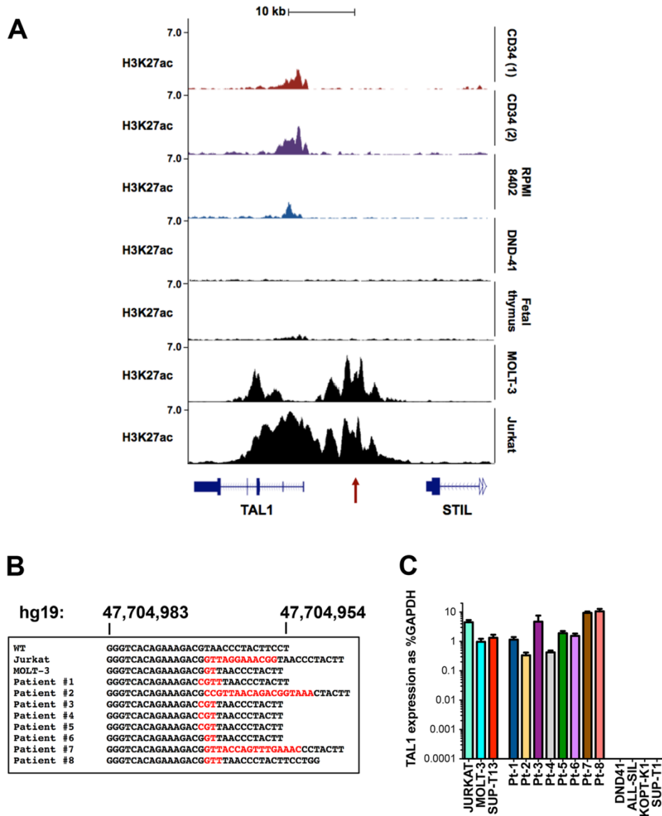
Figure 1. Mutations at an intergenic site are associated with the TAL1 super-enhancer in T-ALL cells (A) Normalized ChIP-seq tracks for H3K27ac at the STIL-TAL1 locus in two human purified normal hematopoietic stem cell samples (CD34), the RPMI-8402 T-ALL cell line that over-expresses TAL1 as a result of TAL1 d , DND-41 T-ALL cells that do not express TAL1 , human fetal thymic tissue, and MOLT-3 and Jurkat cells that have mutations at a non-coding site 7.5 kb from the TAL1 transcriptional start site (red arrow). ChIP-seq read densities (y-axis) were normalized to reads per million reads sequenced in each sample. (B) Sequence alignments of the -7.5 kb site showing wild-type (WT) sequences in black and inserted sequences in red for Jurkat and MOLT-3 T-ALL cell lines and eight pediatric T-ALL patients. (C) TAL1 mRNA expression as determined by quantitative PCR and expressed as percentage of GAPDH. Error bars are \pm SEM from two independent experiments performed in triplicate.
