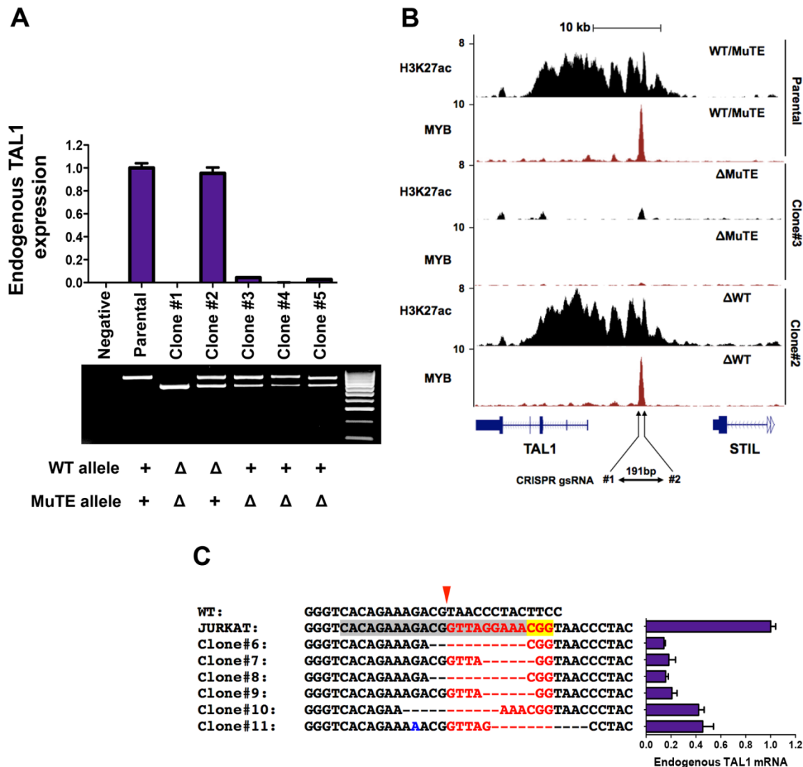
Fig. 4. Targeted deletion of the TAL1 enhancer mutation collapses the TAL1 super-enhancer. (A) Targeted deletion of 177-193 bp of the mutant but not wild-type allele in Jurkat cells abrogates expression of endogenous TAL1 , as determined by qRT-PCR. Data are mean \pm SD of two independent experiments performed in triplicate. Agarose gel of products from PCR amplification across the MuTE site for CRISPR/Cas9 Jurkat clones. All clones, including parental cells, express MSCV- TAL1 . Hyperladder IV on right. Genotype for each clone is shown below: +, allele present; \Delta , deleted allele. (B) ChIP-seq tracks for H3K27ac and MYB at the STIL- TAL1 locus from selected CRISPR/Cas9 clones. ChIP-seq read densities (y-axis) were normalized to reads per million reads sequenced in each sample. (C) Sequence alignments of Jurkat clones targeted by CRISPR/Cas9 gsRNA#3 (target sequence is highlighted in grey, PAM sequence in yellow), which targets the 12 bp insertion in Jurkat cells (red font), but not the wild-type allele. Endogenous TAL1 expression as determined by qRT-PCR for respective clones are shown. Data are mean \pm SD of two independent experiments performed in triplicate.
