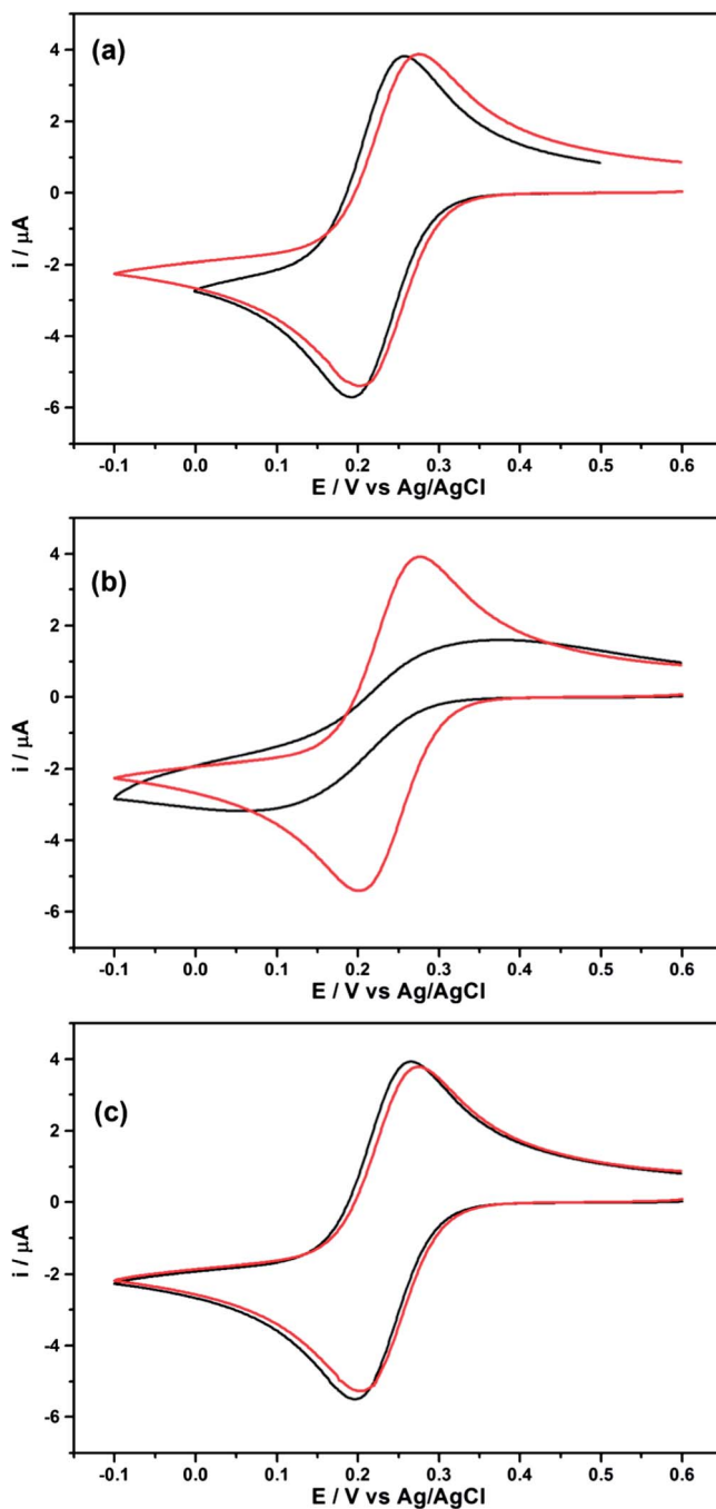
Fig. 5 The influence of pH on the ferri/ferrocyanide redox reaction at different electrodes. (a) Clean BDD; (b) BDD modified with c-GNF; (c) BDD modified with a-GNF. Supporting electrolyte: 0.1 M \text{KH}_2\text{PO}_4 (pH 4.6) (black line); 0.1 M \text{K}_2\text{HPO}_4 (pH 9.2) (red line). Potassium ferricyanide concentration 0.5 \times 10^{-3} M. Scan rate: 50 \text{ mV s}^{-1} .
