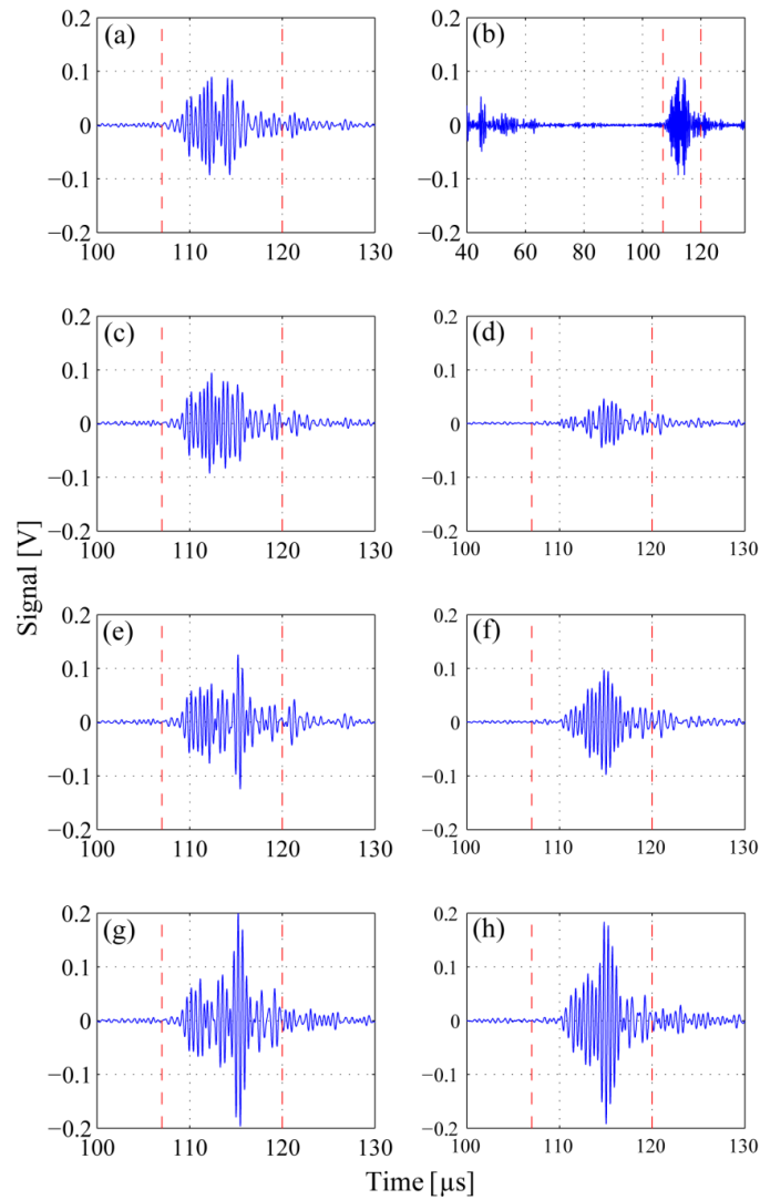
Figure 5. Measured P/E time traces and baseline subtracted signal differences (time window 107 – 120 \mu s shown); (a) zoom of signal for 10'000 cycles, no crack (baseline); (b) signal for 10'000 cycles; (c) signal for 60'000 cycles, crack length 1.06 mm, crack depth 1.06 mm; (d) signal difference for 60'000 cycles; (e) signal for 65'000 cycles, crack length 1.81 mm, crack depth 2.01 mm; (f) signal difference for 65'000 cycles; (g) signal for 70'000 cycles, crack length 3.13 mm, through thickness; (h) signal difference for 70'000 cycles.
