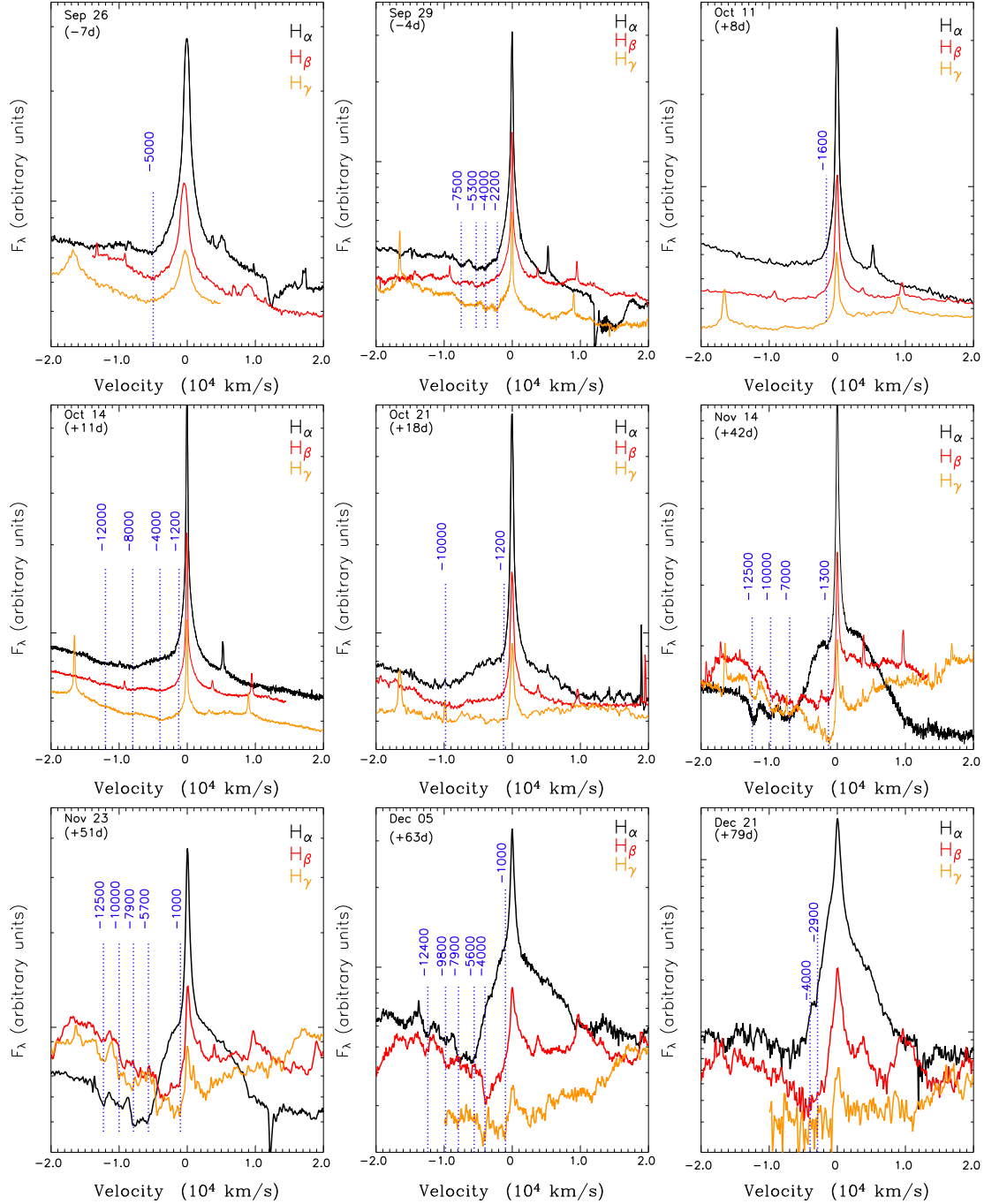
FIG. 15.— H\alpha , H\beta and H\gamma line profiles at representative epochs. Blue dotted lines: velocity of the major absorption components in the H\alpha line profile. For 2012 December 5 we also added two absorption components at -1000\text{ km s}^{-1} and -4000\text{ km s}^{-1} identified in the H\beta and H\gamma lines. The late-time spectrum acquired on t_{\text{pk}} + 101 days shows limited evolution in the H\alpha profile with respect to the previous epoch and it is not shown here.
