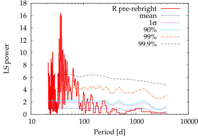
FIG. 31.— Lomb-Scargle periodogram of the R-band magnitude time series for the time interval August 2009 - April 2012 (i.e. before the 2012a and 2012b explosions). This plot shows significant power on time-scales around \sim 40 days. We emphasize that this is not a claim for periodicity. Contours at various significance levels are also shown.
