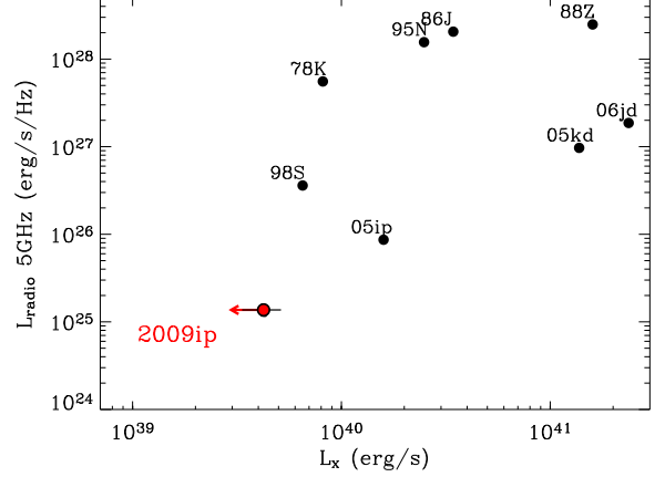
FIG. 26.— Radio luminosity at peak vs. X-ray luminosity at the radio peak for a sample of Type IIn SNe (black dots). SN 2009ip is shown in red. Data have been collected from the literature (Pooley et al. 2002; Smith et al. 2007; Stritzinger et al. 2012; Chandra et al. 2012a; Pooley et al. 2007; Chandra & Soderberg 2007; Chandra et al. 2009; Zampieri et al. 2005; Houck et al. 1998; Chevalier 1987; van Dyk et al. 1993; Fabian & Terlevich 1996; and references therein).
