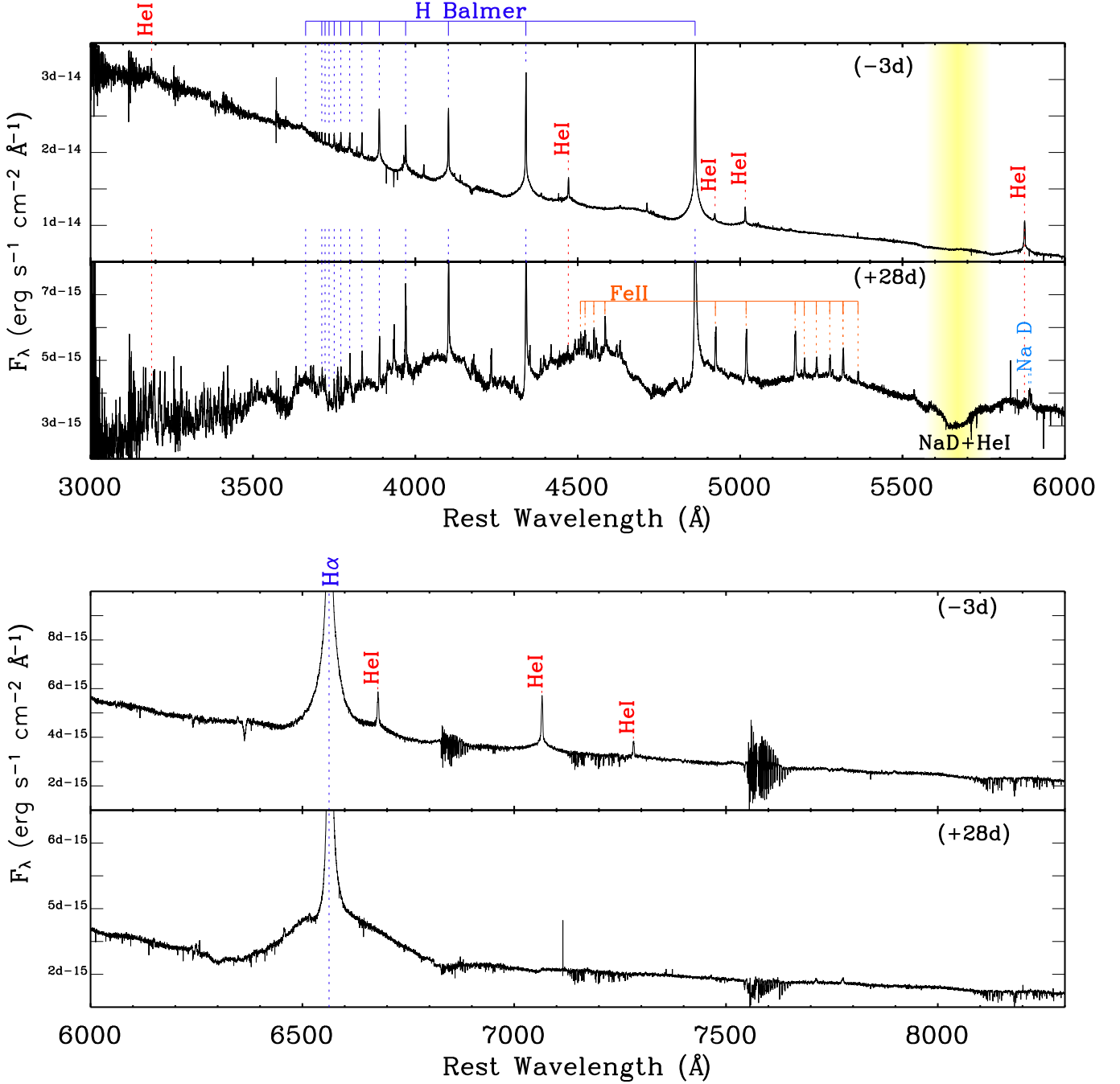
FIG. 19.— High-resolution VLT/X-shooter spectra captured the evolution of SN 2009ip in fine detail. Upper panel: around the optical peak, on 2012 September 30 ( t_{\text{pk}} - 3 days), SN 2009ip shows a narrow-line dominated spectrum typical of SNe (and LBVs) interacting with a medium. One month later ( lower panel of each plot) SN 2009ip started to develop broad emission components (see in particular the H \alpha line) and deep absorption features (e.g. the yellow-shaded band around 5650 Å) more typical of SNe IIP. The complementary 10000–24500 Å wavelength range is shown in Fig. 20. Data have been corrected for Galactic extinction.
