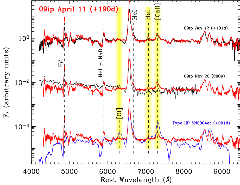
FIG. 30.— Our spectrum taken in April 2013 ( t_{pk} + 190 days) shows minimal evolution with respect to \sim 100 days before. The most notable difference with respect to spectra acquired after or during the eruptions is the presence of intermediate He I and [CaII] in emission. We still do not find evidence for SN-synthesized material (e.g. [OI] 6300 Å). We refer to Sahu et al. (2006) for details on Type IIP SN 2004et.
