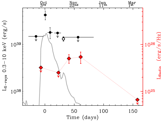
FIG. 8.— X-ray ( Swift -XRT and XMM-Newton, filled and open circle, respectively) and 9 GHz radio light-curve (red squares, VLA) of SN 2009ip. X-rays are detected when the bolometric luminosity reaches its peak. Radio emission is detected at much later times. A re-scaled version of the bolometric light-curve is also shown for comparison. This plot does not include the late time X-ray limit obtained on 2013 April 4.5 ( t_{\text{pk}} + 183 days).
