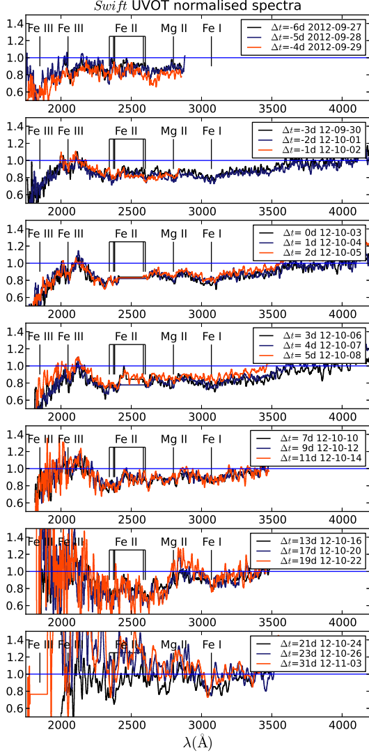
FIG. 4.— UV portion of the Swift -UVOT spectra re-normalized using the black-body fits of Sect. 3. Fe III absorption features become weaker with time, while Fe II develops stronger absorption features, consistent with the progressive decrease of the temperature with time (Fig. 11).
