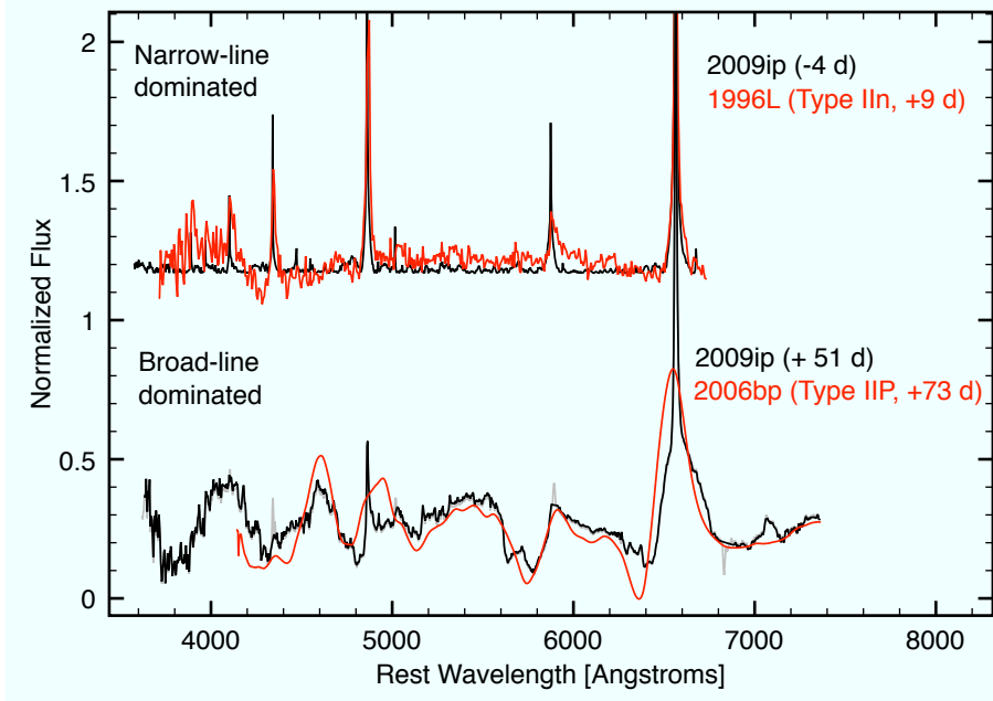
FIG. 21.— SN 2009ip evolved from a narrow-line dominated spectrum typical of Type IIn SN explosions (e.g. SN 1996L, Benetti et al. 1999) to a spectrum that clearly shows broad absorption features more typical of Type IIP SNe (like SN 2006bp, Quimby et al. 2007).
