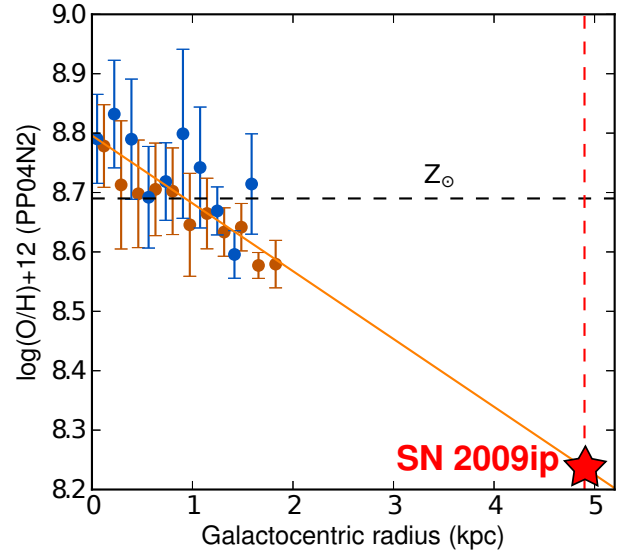
FIG. 23.— Metallicity profile of the host galaxy of SN 2009ip, NGC 7259, with best-fitting metallicity gradient. The vertical dashed line marks the SN galactocentric radius. The colors distinguish measurements from opposite sides of the galaxy center. We find 8.2 < \log(\text{O}/\text{H}) + 12 < 8.6 ( 0.4 Z_{\odot} < Z < 0.9 Z_{\odot} ) at the explosion site of SN 2009ip.
