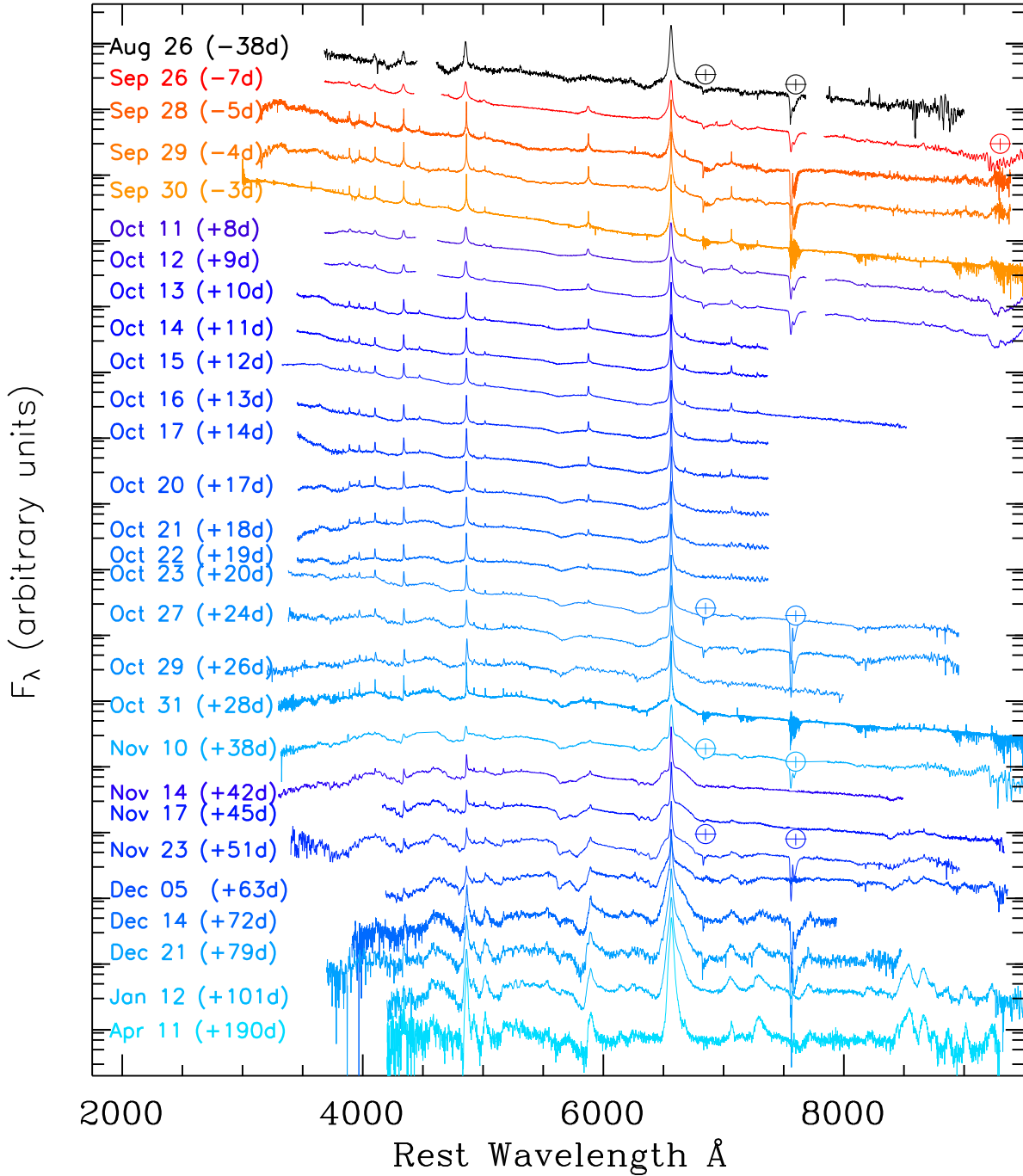
FIG. 6.— Optical spectra of SN 2009ip. Shades of red (blue) are used for spectra obtained during the rise (decay) time of the 2012b explosion. Black is used for the 2012a outburst.
