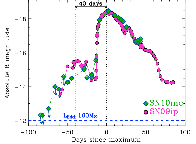
FIG. 29.— The comparison between SN 2009ip and the type II in SN 2010mc (Ofek et al. 2013b) reveals a striking similarity.
