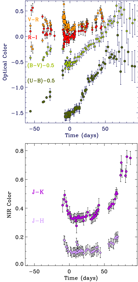
FIG. 12.— Evolution of the optical and NIR colors While SN 2009ip clearly evolves towards redder optical colors starting from t_{\text{pk}} - 3 days, no strong evolution is apparent in the NIR colors in the same time interval.
