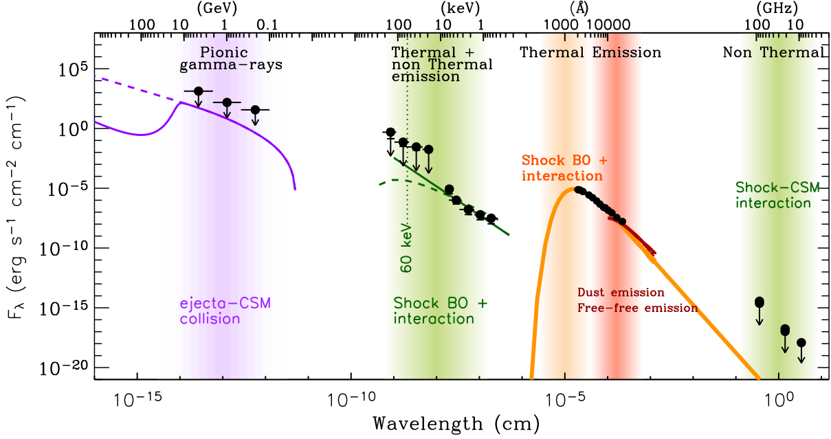
FIG. 27.— Broad-band SED of SN2009ip around the optical peak. Shaded bands highlight different components that dominate at different wavelengths. Neutral pion decay leads to \gamma -rays which are powered by the collision between the ejecta and extremely dense CSM shells. We show the limits from Fermi -LAT obtained between t_{\text{pk}} - 2 days and t_{\text{pk}} + 4 days. Dashed purple line: expected GeV emission based on Section 7.2 assuming no attenuation. The thick-line model includes partial attenuation as relevant for a clumpy and/or asymmetric medium (Sec. 7.4). Soft and hard X-ray emission originates from the interaction of the shock with the CSM: both thermal and non-thermal emission might arise, mainly depending on the environment density. We show here a power-law (non-thermal emission, thick line with F_{\lambda} \propto \lambda^{-2.4} ) and a thermal bremsstrahlung model with kT = 60 keV (dashed line) that fit the Swift -XRT 0.3-10 keV data obtained between t_{\text{pk}} - 2 days and t_{\text{pk}} + 4 days. Swift -BAT 15-150 keV data acquired at t_{\text{pk}} \pm 1 days are also shown. The dotted line marks the energy of 60 keV: this is the typical frequency of high-energy photons emitted by the collision-less shock that forms at shock break-out (Katz et al. 2011). Optical and UV emission is powered by the shock break-out plus continued shock interaction with the environment. Orange line: best-fitting black-body with T \approx 17000 K at t \approx t_{\text{pk}} . NIR and IR emission could originate from dust (formation, vaporization or light-echo) or free-free emission. Due to the high temperature ( T \approx 3000 K, crimson solid line) only dust vaporization or (more likely) free-free emission from an extended outflow can explain our observations. Shock-CSM interaction is also the source of millimeter and radio photons through synchrotron emission. At these times this emission was quenched by free-free absorption by the dense shell of material.
