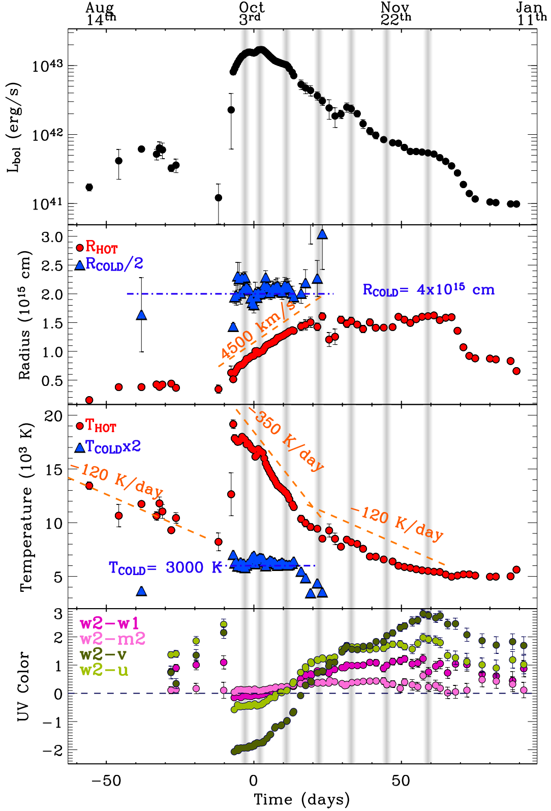
FIG. 11.— Upper panel: Bolometric light-curve of SN 2009ip calculated from the best-fitting black-body temperatures and radii displayed in the intermediate panels. Lower panel: UV color evolution with time. The onset of the 2012b explosion corresponds to a sudden change in UV colors. After that, the UV colors become progressively redder. Vertical shaded bands mark the time of observed bumps in the photometry of Fig. 2: some are powerful enough to be clearly visible in the bolometric luminosity curve as well.
