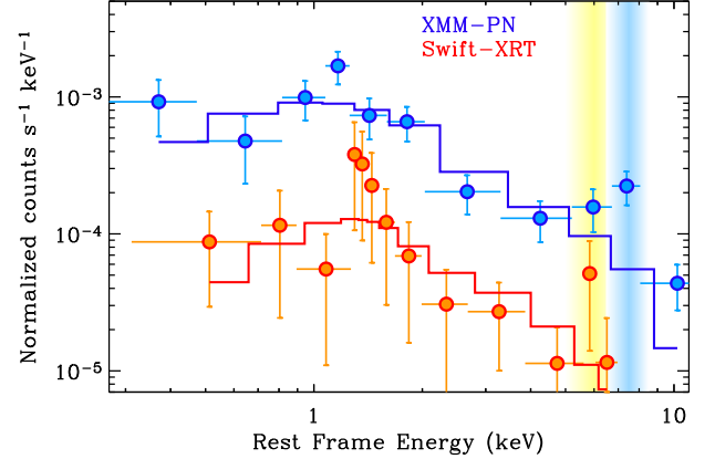
FIG. 9.— X-ray spectra of SN 2009ip. The Swift -XRT spectrum collects observations obtained around the optical peak ( t_{\text{pk}} - 2 days until t_{\text{pk}} + 13 days, total exposure time of 86 ks). The XMM EPIC-PN spectrum was obtained on 2012 November 3 ( t_{\text{pk}} + 31 days, total exposure of 55 ks). The spectral model consists of absorbed bremsstrahlung emission at kT = 60 keV and intrinsic absorption ( \text{NH}_{\text{int}} = 0.10^{+0.06}_{-0.05} \times 10^{22} \text{ cm}^{-2} and \text{NH}_{\text{int}} < 3.1 \times 10^{21} \text{ cm}^{-2} for the XMM and XRT spectra, respectively). Contamination by a nearby source lying \approx 6'' from SN 2009ip is expected for the XMM spectrum. The color-coded shaded areas highlight the presence of possible emission excess with respect to the model.
