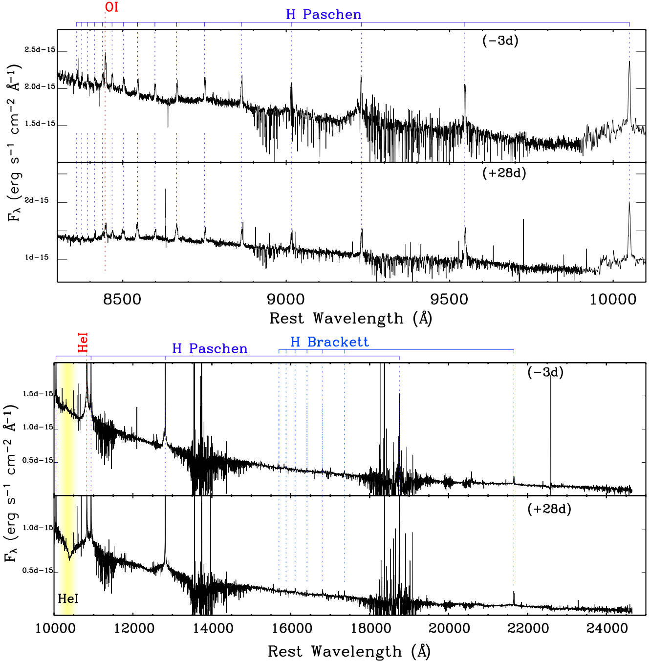
FIG. 20.— High-resolution VLT/X-shooter spectra from 10000 to 24500 Å. Continued from Fig. 19.
