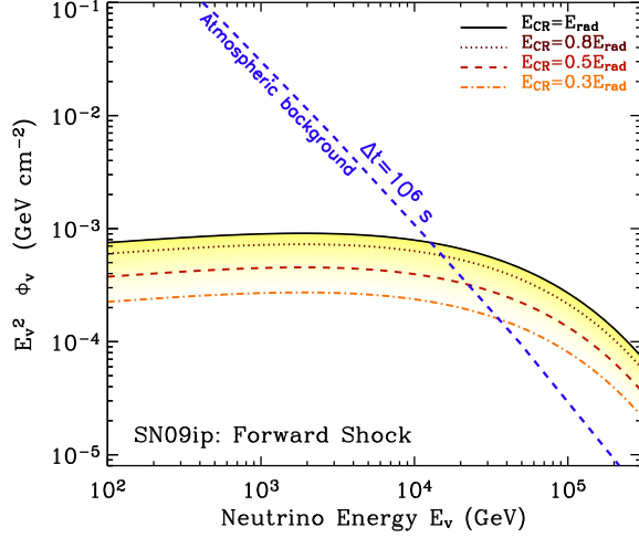
FIG. 28.— Predicted muon and anti-muon neutrino fluence for different values of the total energy in cosmic rays E_{\text{CR}} , here parametrized as a function of the radiated energy at t_{\text{rise}} . Since E_k > E_{\text{rad}} , larger values of E_{\text{CR}} are also possible. Dashed blue line: atmospheric neutrino background integrated over \Delta t \approx t_{\text{rise}} (zenith-angle averaged within 1^\circ ). For this event, the atmospheric neutrino background is more severe since SN 2009ip occurred in the southern hemisphere. For better localized explosions, this plot shows how limits on the neutrino emission can be used to constrain E_{\text{CR}} .
