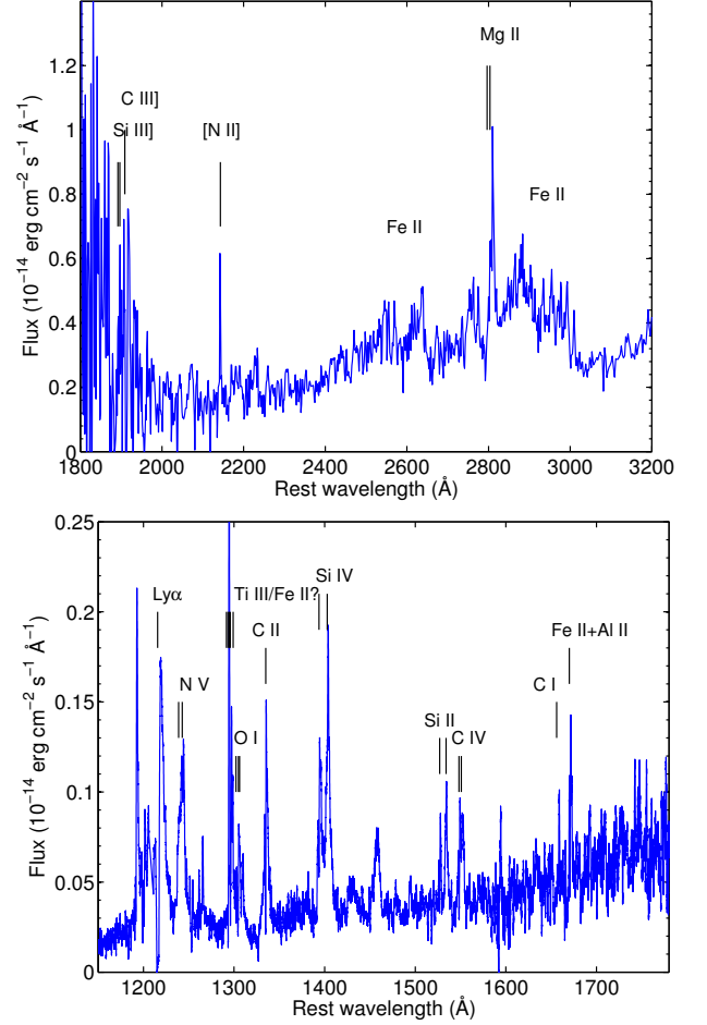
FIG. 5.— Upper panel : HST-STIS spectrum obtained on 2012 October 29 ( t_{\text{pk}} + 26 days). The C III] and Si III] identifications are in a noisy part of the spectrum and are therefore uncertain. Lower panel : HST-COS spectrum obtained on 2012 November 6 ( t_{\text{pk}} + 34 days).
