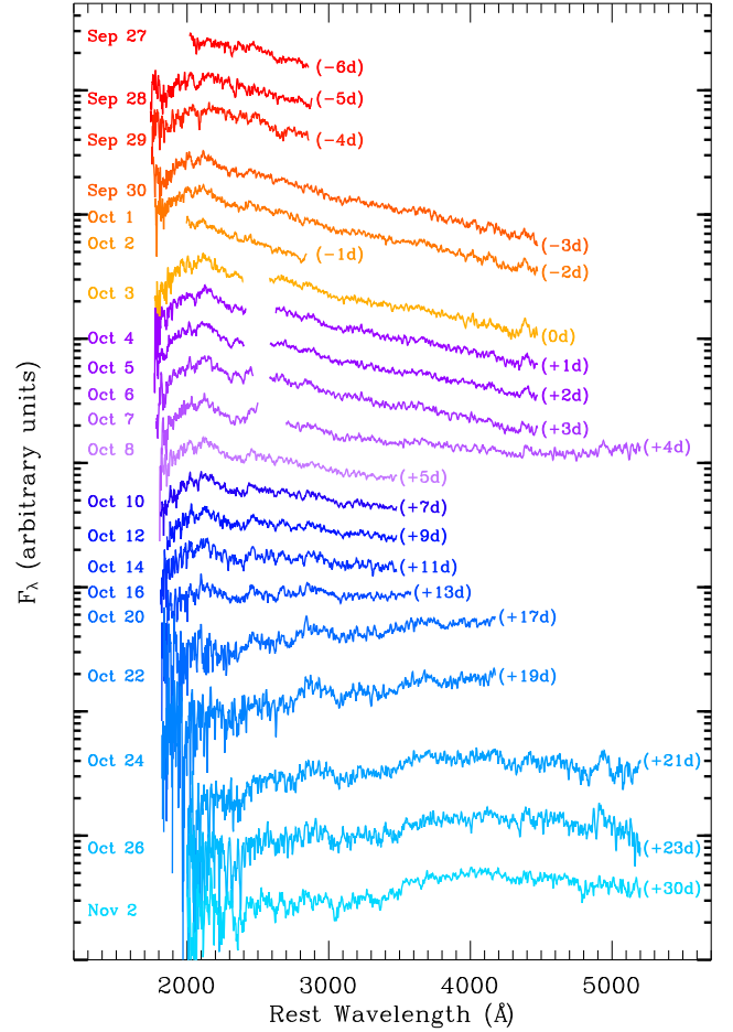
FIG. 3.— Sequence of Swift -UVOT spectra of SN 2009ip covering the rise time (red to orange), peak time (shades of purple) and decay time (shades of blue) of the 2012b explosion.
