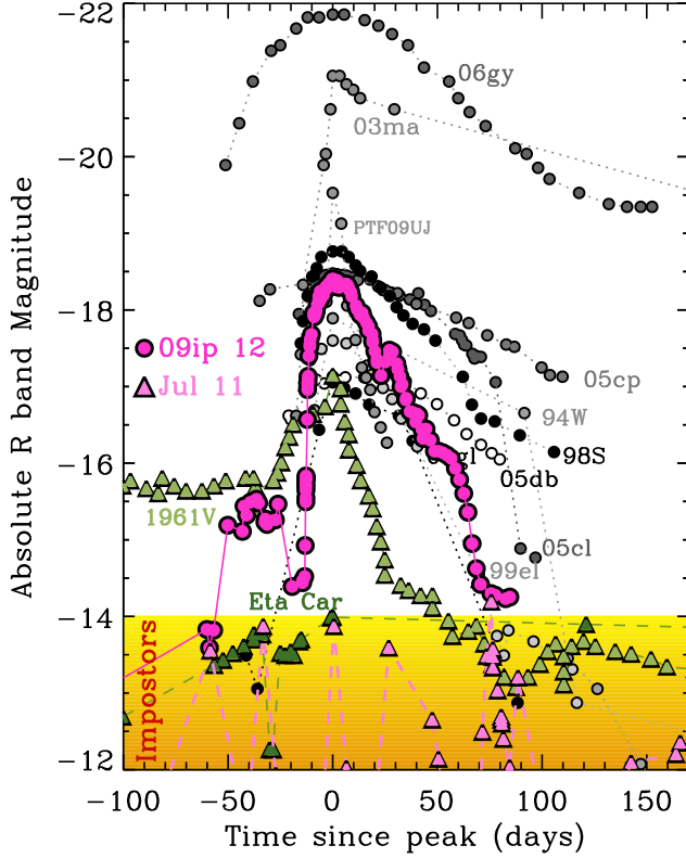
FIG. 24.— Absolute R-band magnitude of SN 2009ip (pink dots) compared to the sample of Type IIc SNe with R-band photometric coverage around the peak (from Kiewe et al. 2012, Ofek et al. 2010). Colored area: typical absolute magnitude of LBV-like eruption episodes. Pink triangles mark the luminosity of SN 2009ip during the 2011 outburst ( t = 0 corresponds here to 2011 July 8 for convenience). The exceptional SN (impostor?) SN1961V (photographic plate magnitudes, from Pastorello et al. 2012) and \eta Carinae during the 19th century Great Eruption ( M_{\text{vis}} as compiled by Frew 2004, see also Smith & Frew 2011) are shown with green triangles. The comparison with SN 2010mc is shown in Fig. 29.
