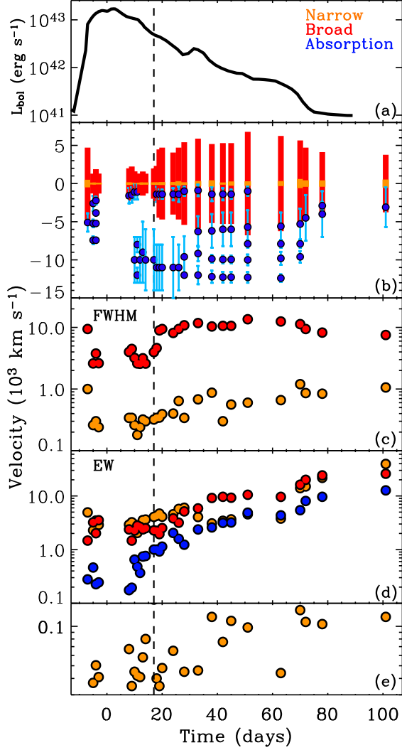
FIG. 16.— Evolution of the H\alpha line with time. We model the H\alpha line with a combination of Lorentzian and Gaussian functions. Orange, red and blue is used for the narrow, broad and blue-shifted absorption components, respectively. Panel (a): bolometric light-curve. Panel (b): the red (orange) bars span the FWHM of the broad (narrow) component. These values are also reported in panel (c). Blue dots: absorption minima as obtained by modeling the absorption with a combination of Gaussians. Negative values indicate blue-shifted components. We use light-blue bars to mark the 1\sigma width. Panel (d) shows the evolution of the equivalent width of the different components. The peak of the narrow component progressively shifts to larger redshifted velocities as illustrated in Panel (e) and independently found by Fraser et al. (2013). The vertical dashed line marks an important time in the evolution of SN 2009ip from different perspectives: from this plot it is clear that around this time the width of broad component undergoes a remarkable transition from \text{FWHM} \sim 3000 \text{ km s}^{-1} to \text{FWHM} \sim 10000 \text{ km s}^{-1} .
