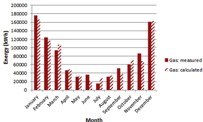
Fig. 3. Monthly gas use: calculated vs. measured.
