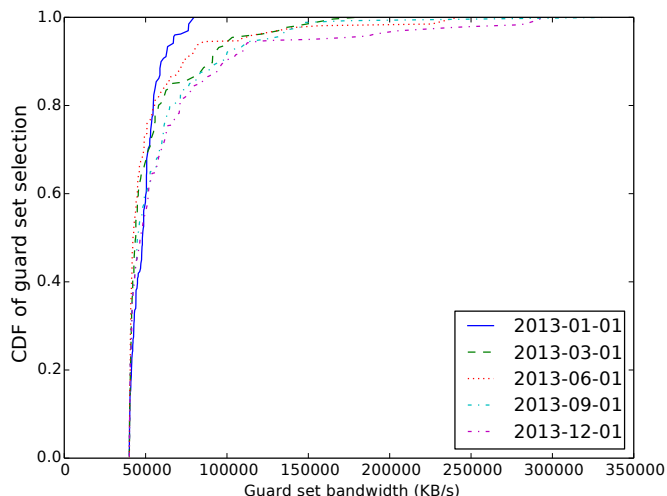
(b) CDF of probabilities of guard set bandwidth (consensus bandwidth)
