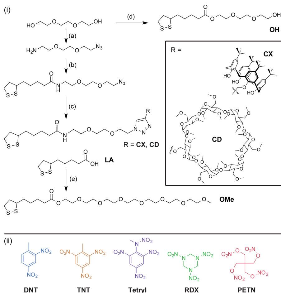
Figure 2. Synthesis and molecules used for surface creation and testing. (i, a) Mesyl chloride, triethylamine (TEA), THF, RT, then NaN 3 , H 2 O, 100 °C, then PPh 3 , 1 M HCl, EtOAc, RT, 65%; (b) LA, DCC, DMAP, DCM, RT, 97%; (c) Cu@C catalyst, monopropargyl cavitand, TEA, dioxane, 70 °C, 3 days; (d) as (b), 0.1 equiv LA, 60%; and (e) methoxyPEG 350, as (b), 82%. (ii) Analytes tested.
