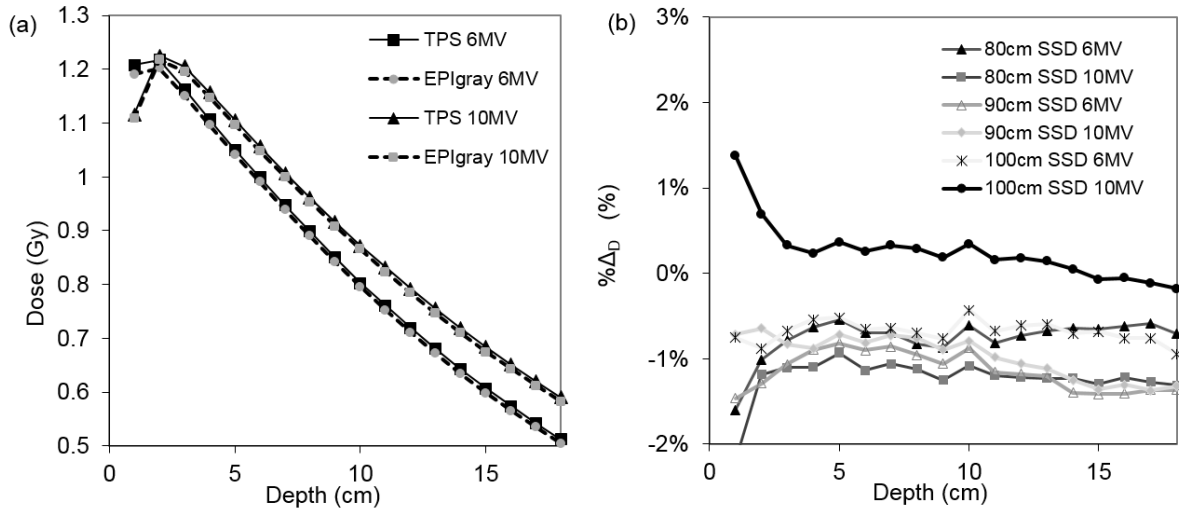
Figure 2 (a) EPIgray and TPS reconstructed doses over a range of depths along the cax: 10 \times 10 \text{ cm}^2 field (100 MU, 6 MV and 10 MV) delivered to a 20 cm thick solid water phantom at 90 cm SSD, (b) \% \Delta_D of reconstructed doses at a range of depths measured at 80 cm, 90 cm and 100 cm SSD.
