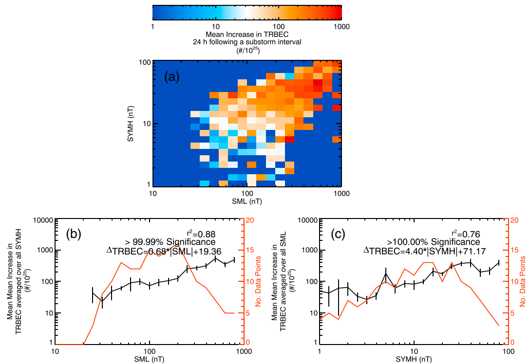
Figure 5. (a) Two-dimensional histogram of the mean increase of TRBEC (divided by 10 25 ) 24 h following substorm intervals against |SML| and |SYM-H|. (b) The mean increase in TRBEC averaged over all |SYM-H| against |SML|. (c) The mean increase in TRBEC averaged over all |SML|. The red traces in Figures 5b and 5c show the number of data points making up the mean values. The square of the Rank Order Correlation coefficient is given in Figures 5b and 5c, along with the significance of this correlation determined by the Student's T test.
