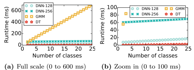
Figure 6: DSP runtime of the inference stage of the various classifiers as a function of the number of classes. The results suggest that DNNs scale extremely well with the increase in the number of classes, in a manner similar to a DT, while often providing superior accuracy.
