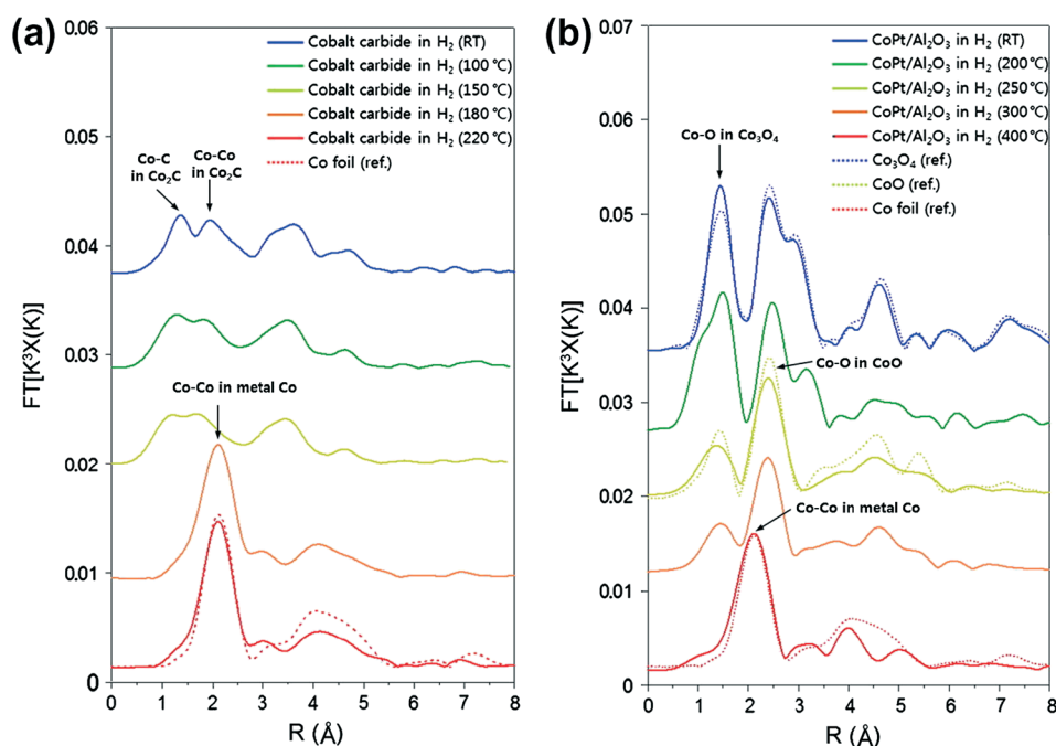
Fig. 8 k^3 -weighted Fourier-transform magnitudes of Co K-edge EXAFS spectra of the reduction in H 2 of a) Co 2 C and b) CoPt/Al 2 O 3 . Reproduced with permission from Elsevier, Kwak et al. J. Catal. , 2013, 307 , 27–36. 78
