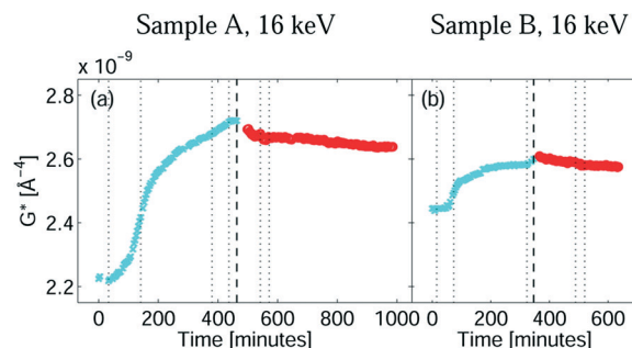
Fig. 5 Variation in the scattering invariant ( G^* ) over reduction and FTS. Reproduced with permission from the American Chemical Society, Høydalsvik et al. J. Phys. Chem. C , 2014, 118 , 2399–2407. 50
