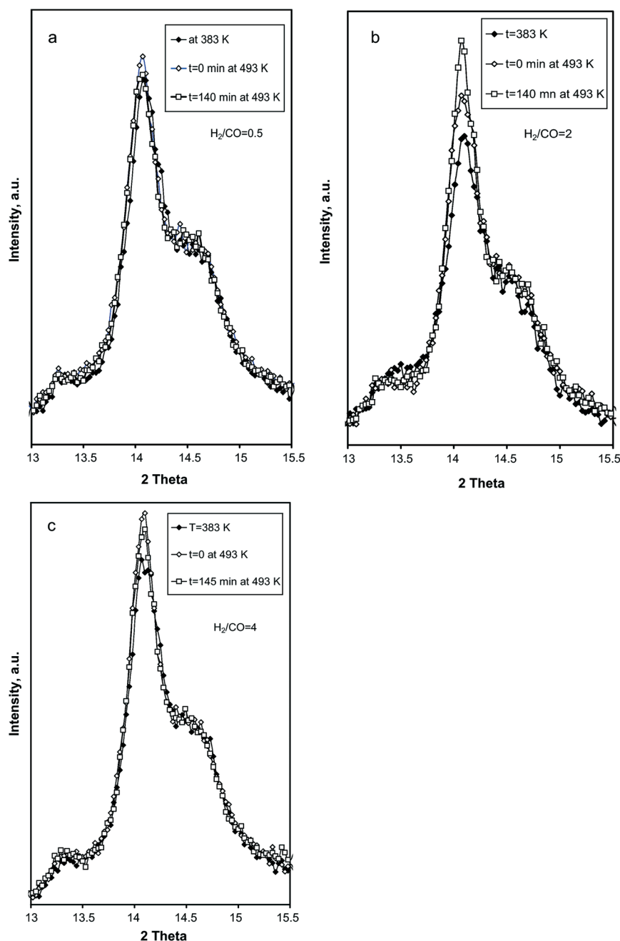
Fig. 2 XRPD diffraction patterns of \text{CoPt}/\text{Al}_2\text{O}_3 catalysts under syngas at a pressure of 20 bar. All three frames display diffraction patterns before the temperature ramp to FTS conditions, at the beginning of FTS and after \sim 140 min. Of various syngas ratios a) \text{H}_2/\text{CO} = 0.5 b) \text{H}_2/\text{CO} = 2 and c) \text{H}_2/\text{CO} = 4 . Reproduced with permission from Elsevier, Sadeqzadeh et al. Catal. Today , 2011, 164 , 62–67. 37
