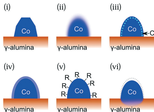
Fig. 6 Schematic representations of the possible cobalt particle changes during FTS which could explain the observed data changes in the SAXS data: (i) faceting, (ii) surface reconstruction and relaxation, (iii) formation of a subsurface carbon layer, (iv) surface reoxidation, (v) adsorbed monolayer of CO or a layer of hydrocarbons, and (vi) diffusion/interaction with the alumina support. Reproduced with permission from the American Chemical Society, Høydalsvik et al. J. Phys. Chem. C , 2014, 118 , 2399–2407. 50
