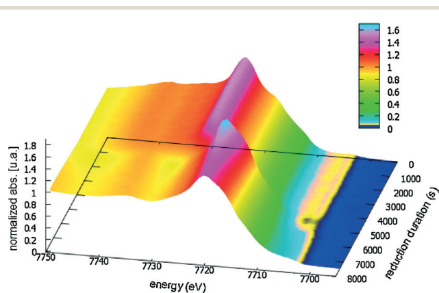
Fig. 7 Time-resolved XANES spectra corresponding to the reduction of a \text{Co}/\text{Al}_2\text{O}_3 catalyst (7 wt%) in a flow of \text{H}_2 heated from RT to 400 °C with a ramp rate of 5 °C \text{min}^{-1} . Reproduced with permission from Elsevier, Rochet et al. Catal. Today , 2011, 171, 186–191. 76
