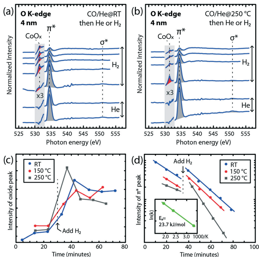
Fig. 14 XAFS spectra of O K-edge and Co L-edge of 4 nm CoO particle sizes at a) room temperature and b) 250 °C and graphs displaying how the intensity of the c) CoO_x and d) \pi^* peaks vary with treatment time run at various temperatures (note logarithmic y-axis in d; the inset in d shows the apparent E_a for the process changing the \pi^* peak intensity in the region after H_2 addition. Reproduced with permission from the American Chemical Society, Tuxen et al. J. Am. Chem. Soc. , 2013, 135 , 2273–2278. 91
