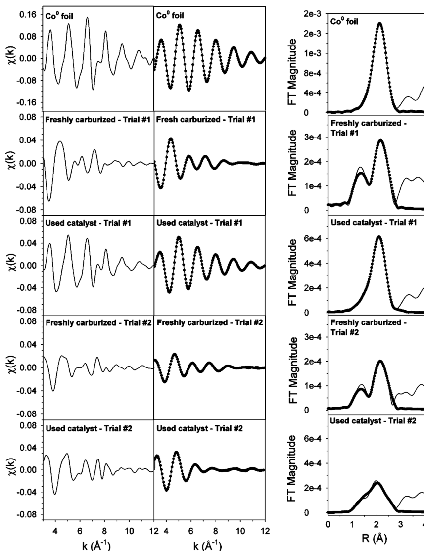
Fig. 9 EXAFS and Fourier Transform magnitude spectra of a \text{Co}^0 reference, \text{Co}_2\text{C} catalyst once prepared and once spent, recorded at the Co K-edge. Reproduced with permission from the American Chemical Society, Mohandas et al. ACS Catal. , 2011, 1, 1581–1588. 81
