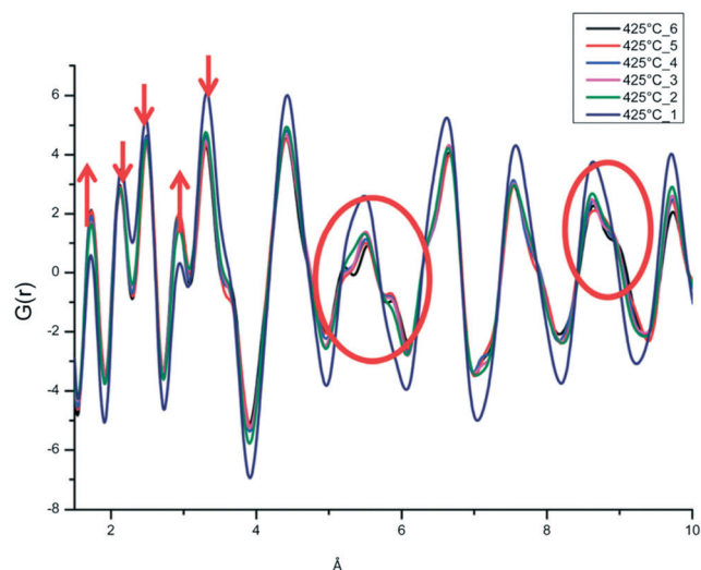
Fig. 3 PDFs acquired during the reduction of Co/Al 2 O 3 . The temperature was held at 425 °C for 2 h. The numbers 1–6 in the figure legend correspond to consecutive 20 min diffractograms over the 2 h reduction period. Reproduced with permission from the Royal Society of Chemistry, du Plessis et al. Phys. Chem. Chem. Phys. , 2013, 15 , 11640–11645. 47
