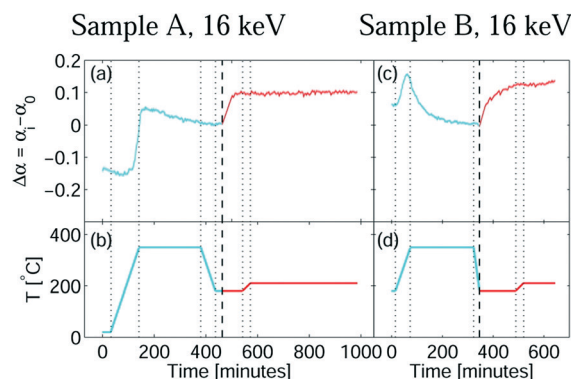
Fig. 4 Variation in the Porod exponent and temperature over reduction and FTS. Reproduced with permission from the American Chemical Society, Høydalsvik et al. J. Phys. Chem. C , 2014, 118 , 2399–2407. 50
