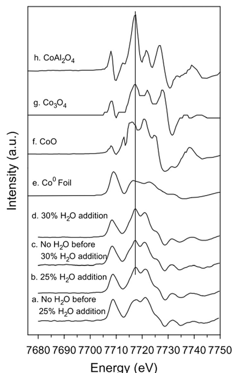
Fig. 10 XANES first derivative spectra of cobalt species present during FTS synthesis a) after stabilisation of FTS, b) after the addition of 25% \text{H}_2\text{O} , c) after a period of recovery, d) after addition of 30% \text{H}_2\text{O} , e–h) reference foils/compounds. For a \text{Co}/\text{Al}_2\text{O}_3 25 wt% catalyst. Reproduced with permission from the Elsevier, Jacobs et al. Appl. Catal., A , 2004, 270 , 65–76. 84
