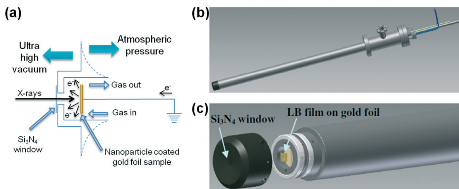
Fig. 11 a) Schematic of in situ soft XAFS cell showing gas flow and b, c) 3D visualisation of the cell and sample holder. Reproduced with permission from Wiley-VCH, Somorjai et al. Angew. Chem., Int. Ed. , 2011, 50 , 10116–10129. 89
