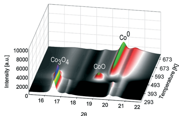
Fig. 1 In situ PXRD patterns from reduction study of Re promoted Co/ \gamma -Al 2 O 3 , recorded using a wavelength of 0.70417 Å. The samples were heated from 293 K to 673 K at 3 K min −1 . The data contain reflections corresponding to Co 3 O 4 (311) at 16.54° 2 \theta , CoO (111) at 18.93° 2 \theta , and Co 0 (111) at 20.44° 2 \theta attributed to fcc and hcp. Reproduced with permission from Elsevier, Rønning et al. Catal. Today , 2010, 155 , 289–295. 34
