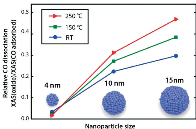
Fig. 13 Calculated variations in relative CO dissociation for particle sizes of 4, 10 and 15 nm, at temperatures of RT, 150 °C and 250 °C. Reproduced with permission from the American Chemical Society, Tuxen et al. J. Am. Chem. Soc. , 2013, 135 , 2273–2278. 91
