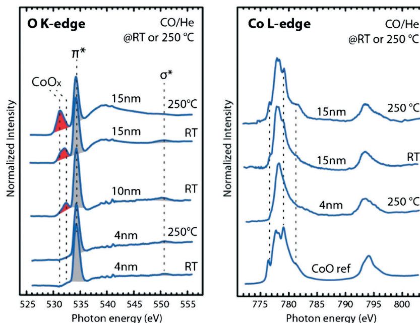
Fig. 12 XAFS spectra of O K-edge and Co L-edge of various \text{Co}^0 particle sizes and reaction temperatures. Reproduced with permission from the American Chemical Society, Tuxen et al. J. Am. Chem. Soc. , 2013, 135 , 2273–2278. 91
