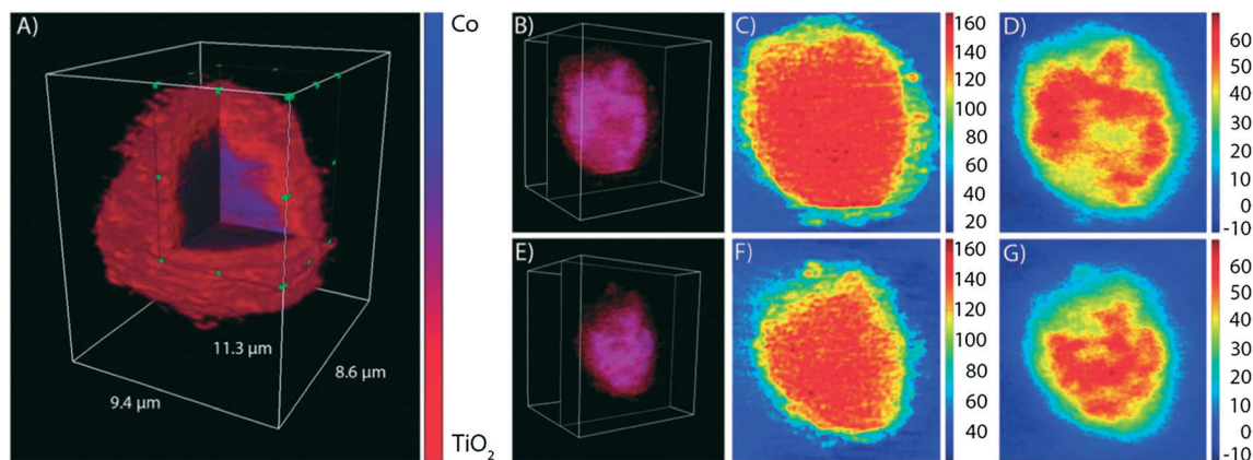
Fig. 15 TXM images. A) 3D representation of an unreduced Co/TiO 2 particle measured at the Co K-edge. Red represents contributions from TiO 2 and blue represents contributions from cobalt. Images B–D and E–G show two slices through the particle. Reproduced with permission from the Royal Society of Chemistry, Cats et al. Chem. Commun. 2013, 4622–4684. 99
