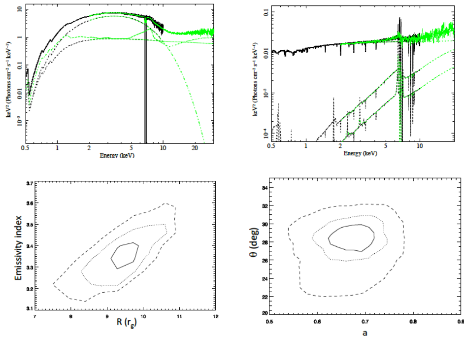
Figure 13. Upper left panel: eXTP broadband (SFA+LDA) spectrum for an exposure of 0.1 ks of a 0.5 Crab, maximally rotating XRBS BH such as GRO J1655-40 [46]. Upper right panel: eXTP spectrum obtained with a 100 ks integration of a 2 mCrab, spin a=0.5 AGN. Lower panels, confidence levels for the disc emission vs. inner radius for XRBS (left) and inclination vs. black hole spin for AGN (right) (1, 2, and 3 sigma solid, dotted, and dashed lines respectively). (Courtesy of the eXTP working group on Strong Field Gravity).
