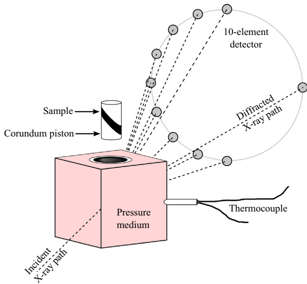
Fig. 1. Illustration of the sample assembly and elements of the 10-element detector. The detectors are positioned at 2\theta = 6.5^\circ and \psi = 0, 90, 180, 202.5, 225, 247.5, 270, 292.5, 315 and 337.5^\circ clockwise from the top when observed along the X-ray beam. For clarity the sleeve and end caps which surround the sample are omitted.
