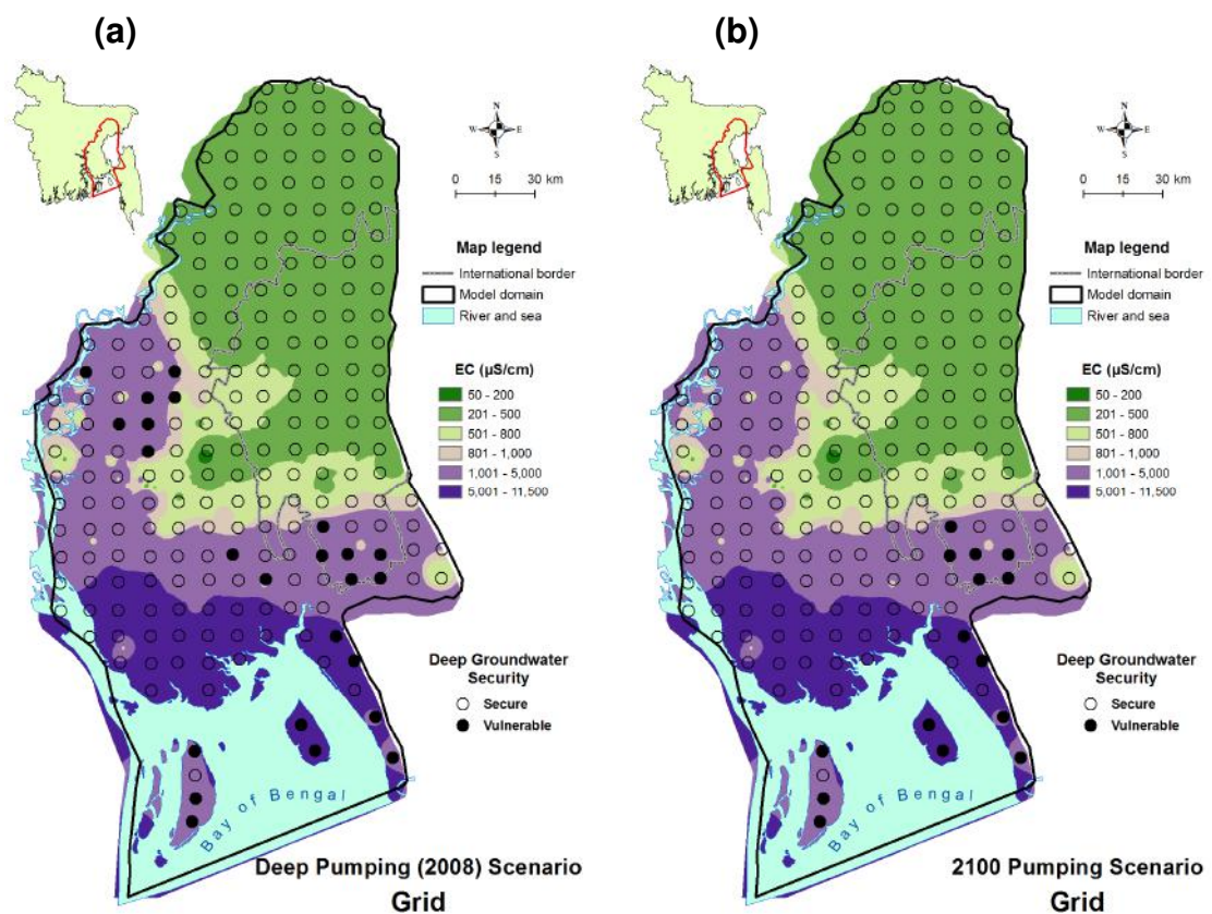
Figure 14 Maps showing the areas of secure and vulnerable deep groundwater abstraction against salinity under the deep 2008 pumping (a), and depth-distributed 2100 pumping (b) scenarios.
