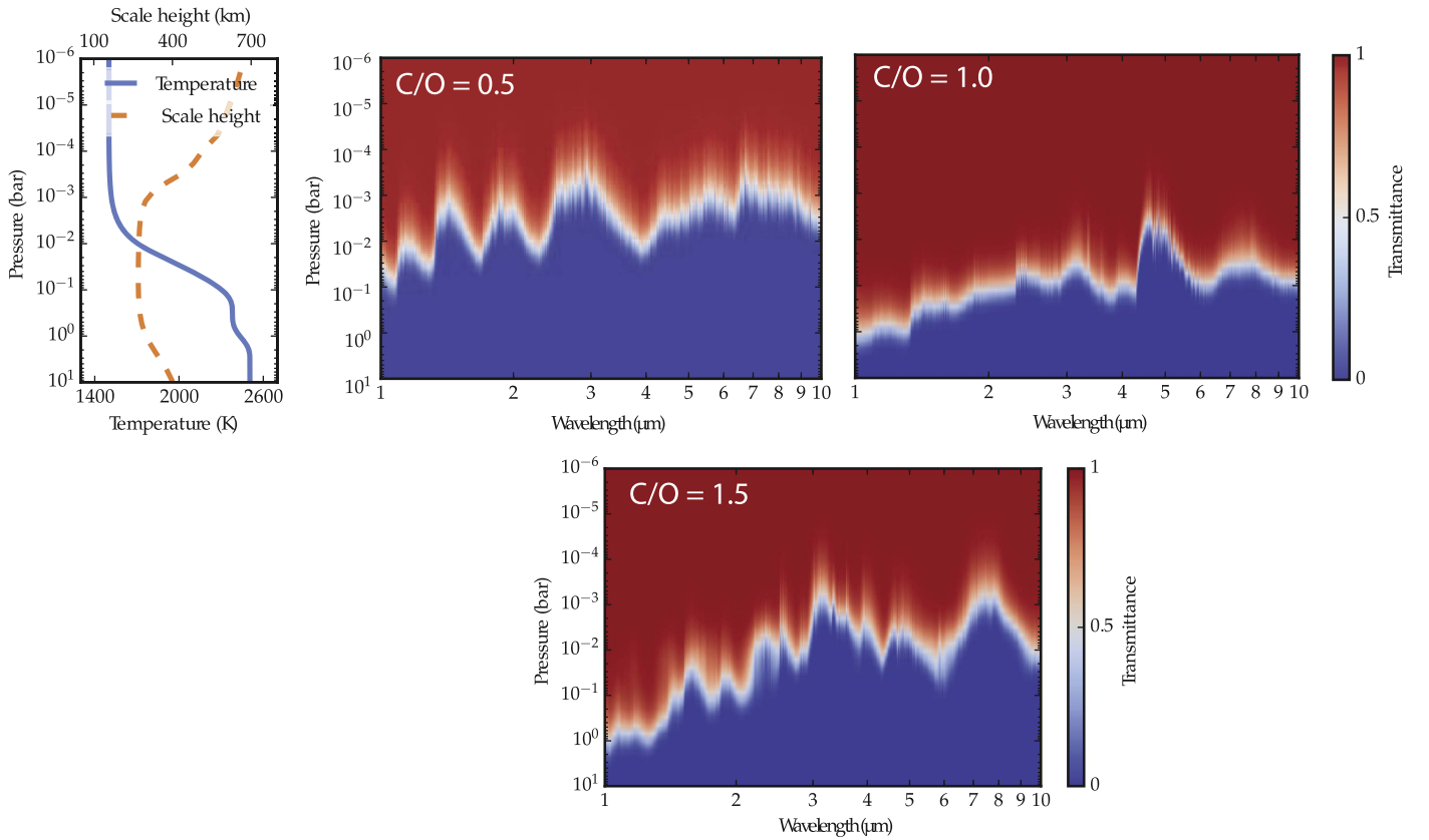
Figure 9. The first plot on the left shows the temperature profile (blue line) and scale height profile (dashed orange line) as a function of pressure. The other panels show the spectral transmittance as a function of pressure for the models with C/O of 0.5, 1.0, and 1.5. Note that the pressure axis is the same as in the first panel. The transmittance is integrated over the path parallel to the line of sight. The transmittance plots allow us to see the pressures (and therefore the temperature and scale height) probed at different wavelengths for different C/O regimes.
