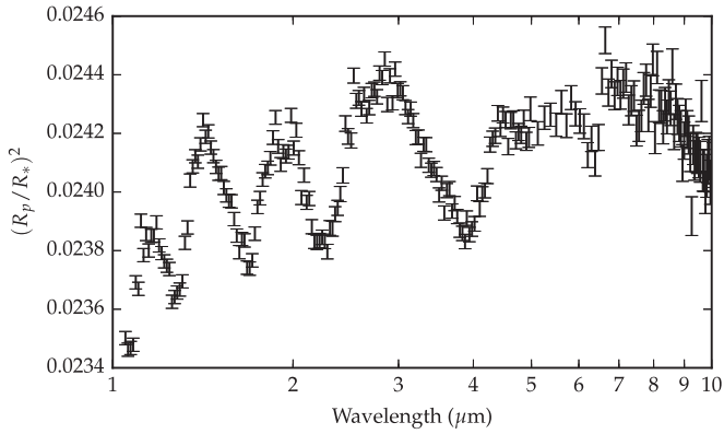
Figure 2. Simulated JWST observation for C/O = 0.5 . The spectrum was obtained combining four separate synthetic observations obtained with NIRISS, NIRCам, and MIRI to cover the 1–10 \mu\text{m} spectral range. This spectrum would therefore require observing a total of four transits.
