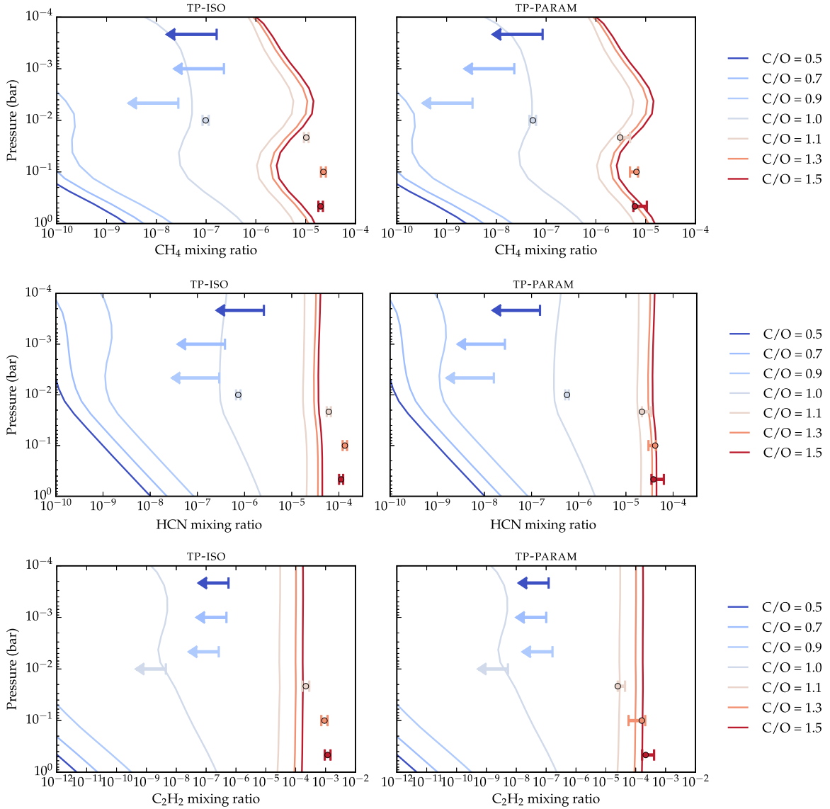
Figure 7. Retrieved \text{CH}_4 (top), \text{HCN} (middle), and \text{C}_2\text{H}_2 (bottom) abundance for \text{C}/\text{O} = 0.5\text{--}1.5 . Caption as in Figure 6.
