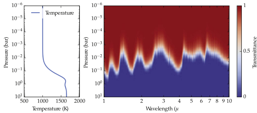
Figure 10. TP profile and spectral transmittance for a planet with a cooler TP profile. Caption as in Figure 9.
